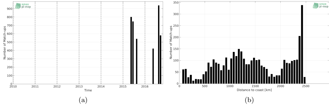
Figure 1: Number of match-ups between TSG-LEGOS-DM and SMAP-L2-JPL-V4 SSS as a function of time (a) and as function of the distance to coast (b) over the OTT zone Pi-MEP region and for the full satellite product period.
