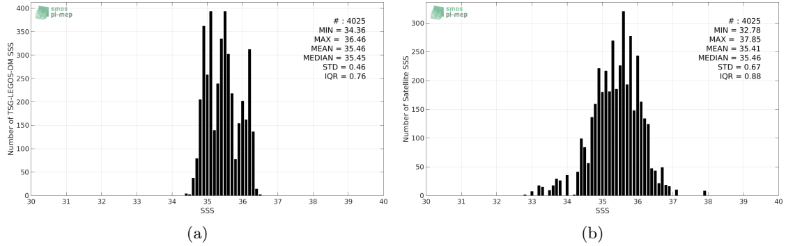
Figure 2: Histograms of SSS from TSG-LEGOS-DM (a) and SMAP-L2-JPL-V4 (b) considering all match-up pairs per bins of 0.1 over the OTT zone Pi-MEP region and for the full satellite product period.
