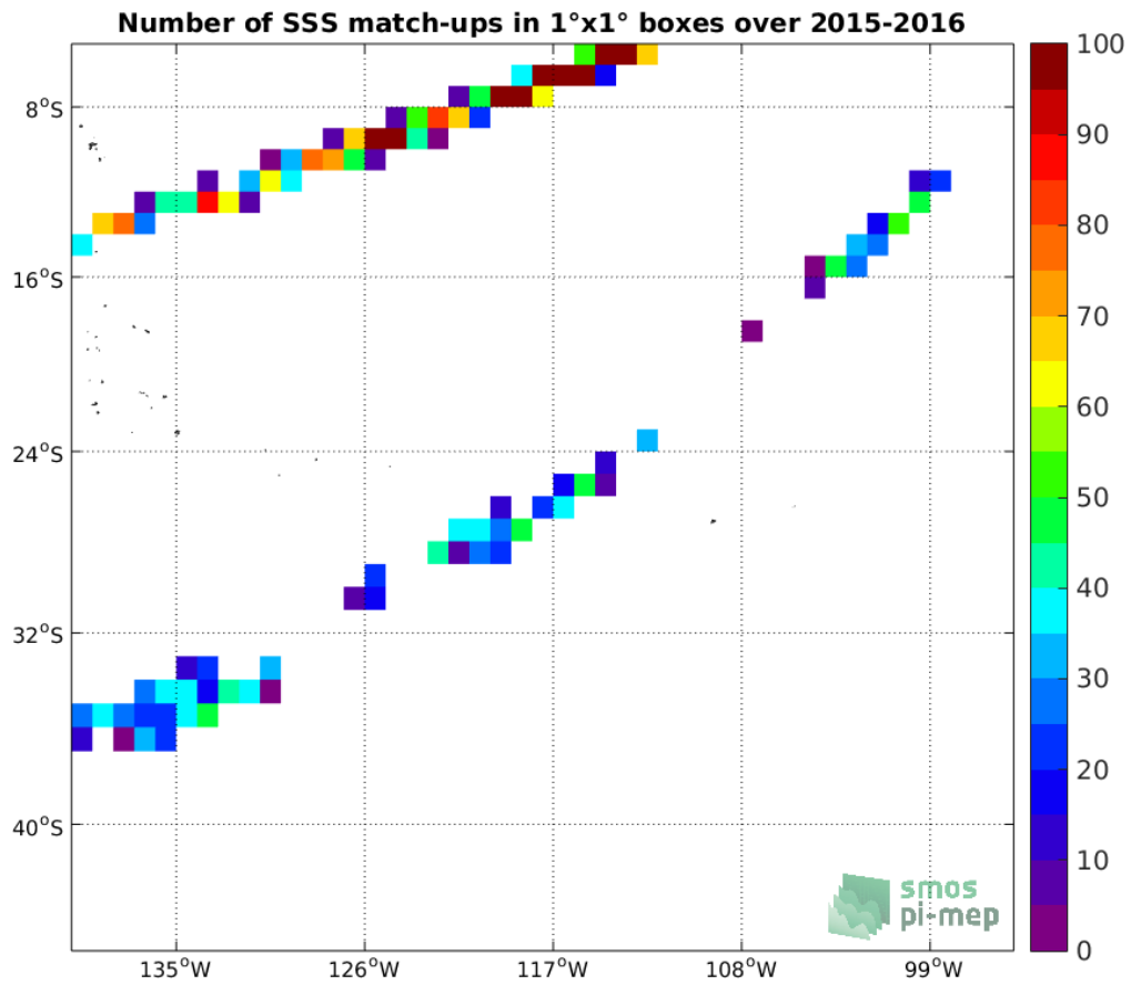
Figure 4: Number of SSS match-ups between TSG-LEGOS-DM SSS and the SMAP-L2-JPL-V4 SSS product for the OTT zone Pi-MEP region over 1°x1° boxes and for the full satellite product period.
