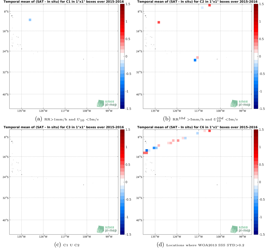
Figure 12: Temporal mean gridded over spatial boxes of size 1^\circ \times 1^\circ of \Delta SSS (SMAP-L2-JPL-V4 - TSG-LEGOS-DM) for 4 different subdatasets corresponding to: RR > 1mm/h and U_{10} < 5\text{m/s} (a), RR^{10d} > 5\text{mm/h} and U_{10}^{10d} < 5\text{m/s} (b), C1 U C2 (c), Locations where WOA2013 SSS STD > 0.2 (d).
