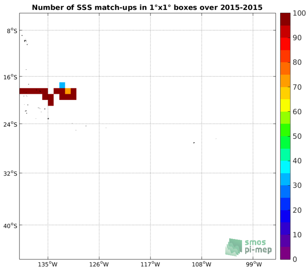
Figure 4: Number of SSS match-ups between TSG-GOSUD-Research-vessel SSS and the SMAP-L2-JPL-V4 SSS product for the OTT zone Pi-MEP region over 1°x1° boxes and for the full satellite product period.
