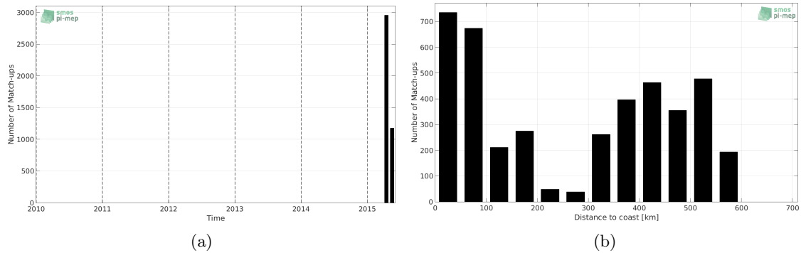
Figure 1: Number of match-ups between TSG-GOSUD-Research-vessel and SMAP-L2-JPL-V4 SSS as a function of time (a) and as function of the distance to coast (b) over the OTT zone Pi-MEP region and for the full satellite product period.
