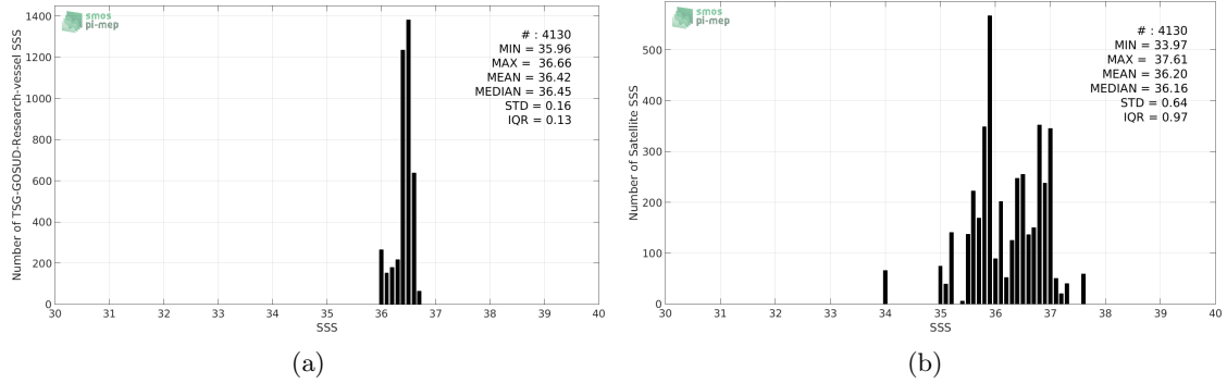
Figure 2: Histograms of SSS from TSG-GOSUD-Research-vessel (a) and SMAP-L2-JPL-V4 (b) considering all match-up pairs per bins of 0.1 over the OTT zone Pi-MEP region and for the full satellite product period.
