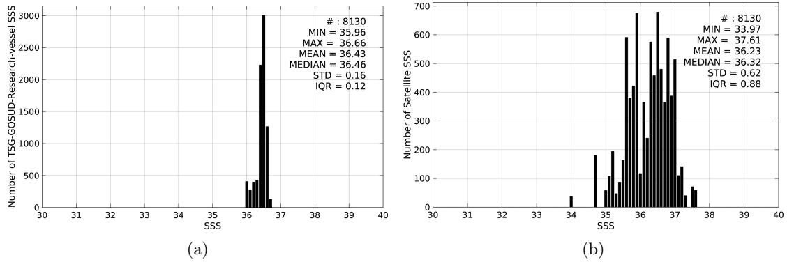
Figure 2: Histograms of SSS from TSG-GOSUD-Research-vessel (a) and SMAP-L2-JPL-V4 (b) considering all match-up pairs per bins of 0.1 over the OTT zone Pi-MEP region and for the full satellite product period.
