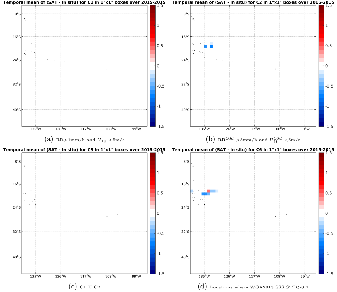
Figure 12: Temporal mean gridded over spatial boxes of size 1^\circ \times 1^\circ of \Delta SSS (SMAP-L2-JPL-V4 - TSG-GOSUD-Research-vessel) for 4 different subdatasets corresponding to: RR > 1\text{mm/h} and U_{10} < 5\text{m/s} (a), RR^{10d} > 5\text{mm/h} and U_{10}^{10d} < 5\text{m/s} (b), C1 U C2 (c), Locations where WOA2013 SSS STD > 0.2 (d).
