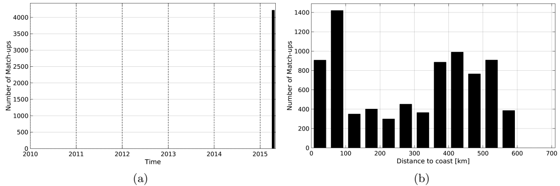
Figure 1: Number of match-ups between TSG-GOSUD-Research-vessel and SMAP-L2-JPL-V4 SSS as a function of time (a) and as function of the distance to coast (b) over the OTT zone Pi-MEP region and for the full satellite product period.
