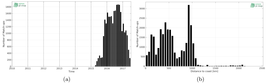
Figure 1: Number of match-ups between Surface drifters and SMAP-L2-JPL-V4 SSS as a function of time (a) and as function of the distance to coast (b) over the OTT zone Pi-MEP region and for the full satellite product period.
