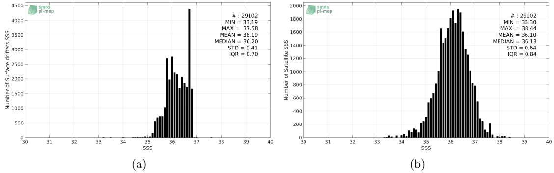
Figure 2: Histograms of SSS from Surface drifters (a) and SMAP-L2-JPL-V4 (b) considering all match-up pairs per bins of 0.1 over the OTT zone Pi-MEP region and for the full satellite product period.
