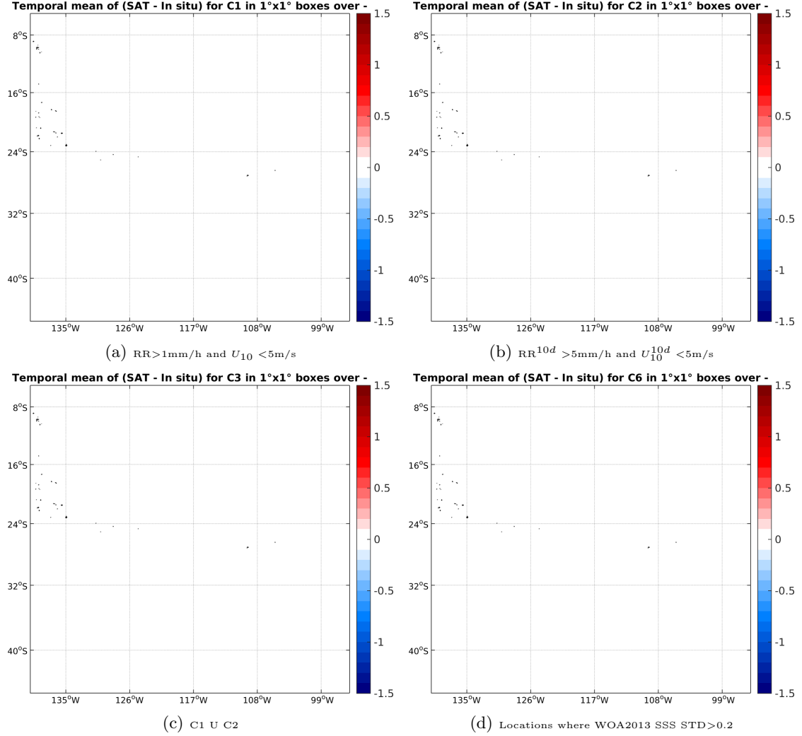
Figure 11: Temporal mean gridded over spatial boxes of size 1^\circ \times 1^\circ of \Delta SSS (SMAP-L2-JPL-V4 - Surface drifters) for 4 different subdatasets corresponding to: RR > 1mm/h and U_{10} < 5 m/s (a), RR 10d > 5mm/h and U_{10}^{10d} < 5 m/s (b), C1 U C2 (c), Locations where WOA2013 SSS STD > 0.2 (d).
