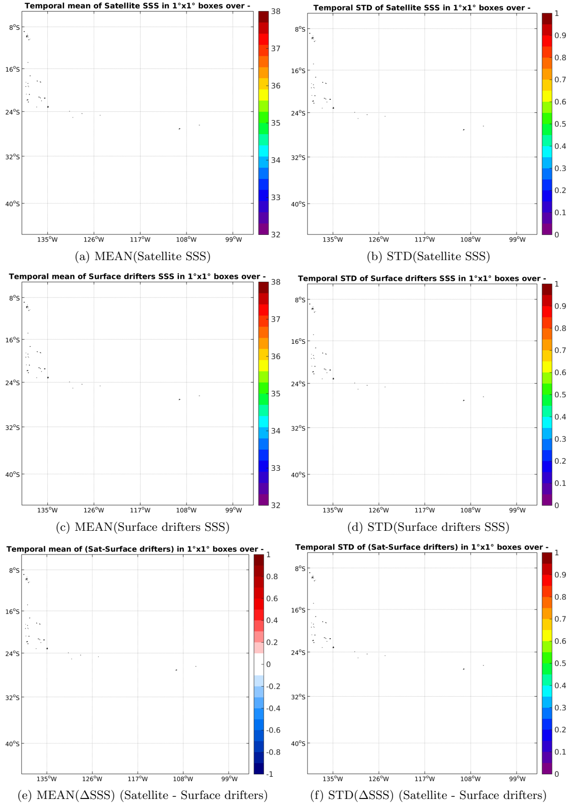
Figure 5: Temporal mean (left) and STD (right) of SSS from SMAP-L2-JPL-V4 (top), Surface drifters (middle), and of \Delta SSS (Satellite - Surface drifters). Only match-up pairs are used to generate these maps.
