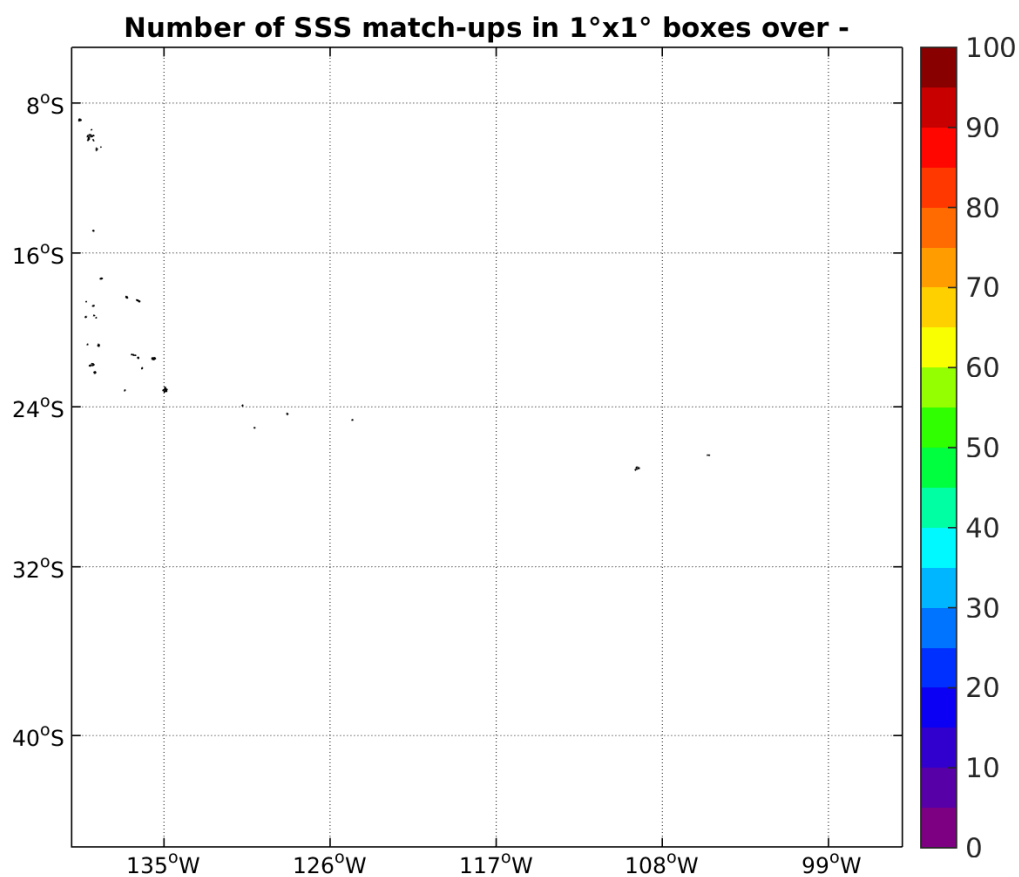
Figure 3: Number of SSS match-ups between Surface drifters SSS and the SMAP-L2-JPL-V4 SSS product for the OTT zone Pi-MEP region over 1°x1° boxes and for the full satellite product period.
