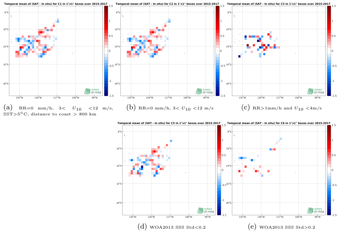
Figure 11: Temporal mean gridded over spatial boxes of size 1^\circ \times 1^\circ of \Delta SSS (SMAP-L2-JPL-V4.2 - Surface drifters) for 5 different subdatasets corresponding to:RR=0 mm/h, 3 < U_{10} < 12 m/s, SST >5^\circ C, distance to coast > 800 km (a), RR=0 mm/h, 3 < U_{10} < 12 m/s (b), RR >1 mm/h and U_{10} < 4 m/s (c), WOA2013 SSS Std <0.2 (d), WOA2013 SSS Std >0.2 (e).
