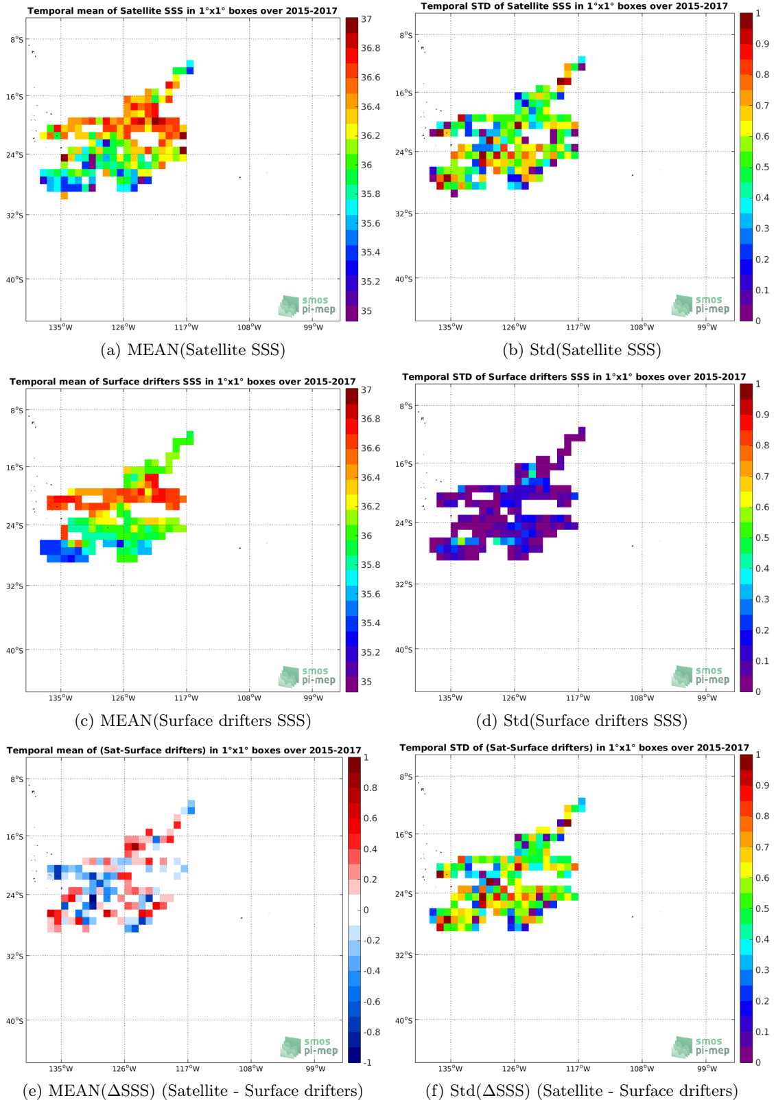
Figure 5: Temporal mean (left) and Std (right) of SSS from SMAP-L2-JPL-V4.2 (top), Surface drifters (middle), and of \Delta SSS (Satellite - Surface drifters). Only match-up pairs are used to generate these maps.
