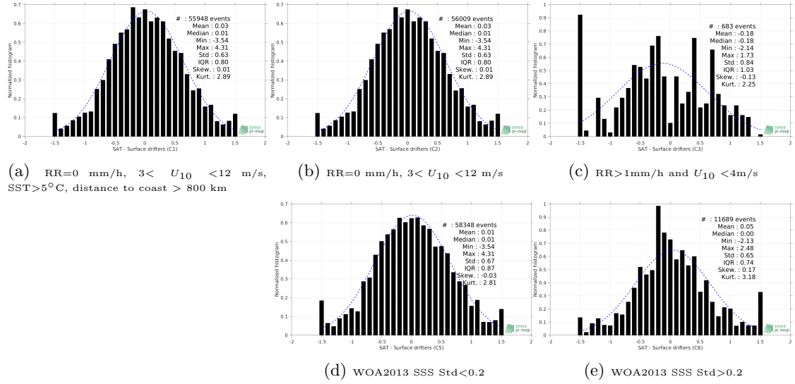
Figure 12: Normalized histogram of \Delta SSS (SMAP-L2-JPL-V4.2 - Surface drifters) for 5 different subdatasets corresponding to: RR=0 mm/h, 3 < U_{10} < 12 m/s, SST > 5°C, distance to coast > 800 km (a), RR=0 mm/h, 3 < U_{10} < 12 m/s (b), RR > 1mm/h and U_{10} < 4 m/s (c), WOA2013 SSS Std < 0.2 (d), WOA2013 SSS Std > 0.2 (e).
