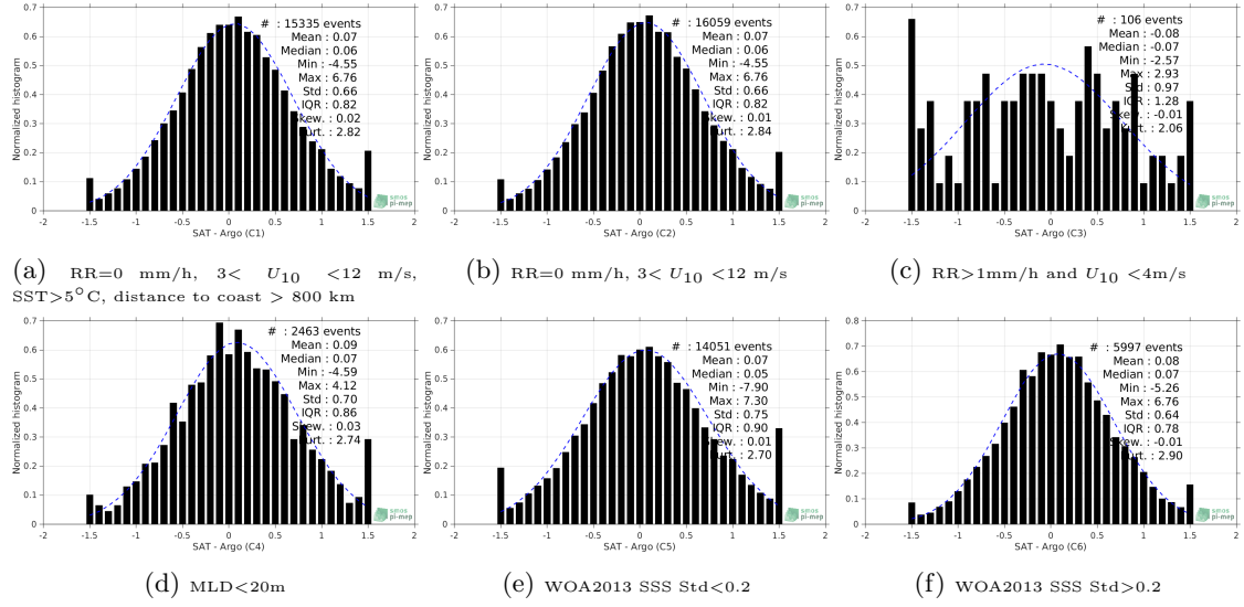
Figure 13: Normalized histogram of \Delta SSS (SMAP-L2-JPL-V4.2 - Argo) for 6 different sub-datasets corresponding to: RR=0 mm/h, 3 < U_{10} < 12 m/s, SST >5^{\circ} C, distance to coast > 800 km (a), RR=0 mm/h, 3 < U_{10} < 12 m/s (b), RR >1 mm/h and U_{10} < 4 m/s (c), MLD <20 m (d), WOA2013 SSS Std <0.2 (e), WOA2013 SSS Std >0.2 (f).
