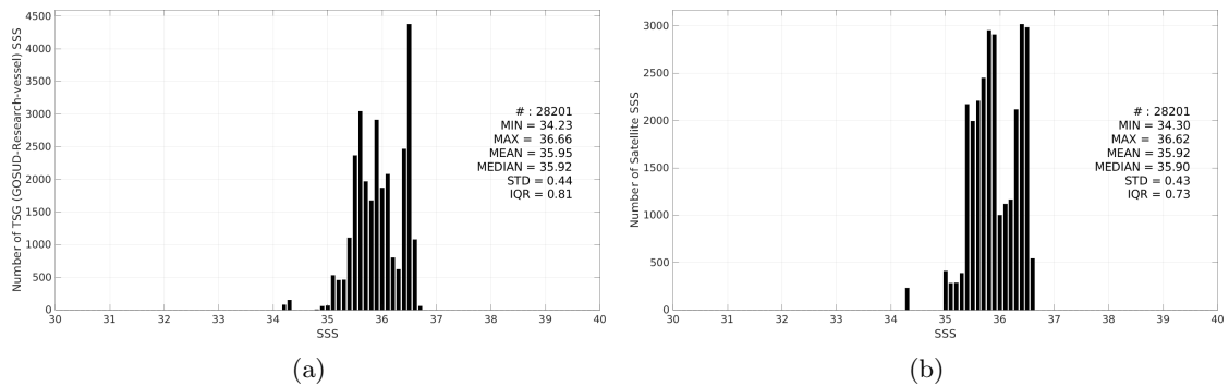
Figure 3: Histograms of SSS from TSG (GOSUD-Research-vessel) (a) and ISAS v7 - Monthly (Ifremer-LOPS-CMEMS) (b) considering all match-up pairs per bins of 0.1 over the OTT zone Pi-MEP region and for the full satellite product period.
