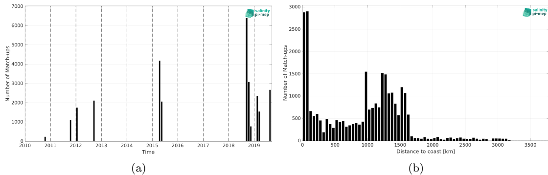
Figure 2: Number of match-ups between TSG (GOSUD-Research-vessel) and ISAS v7 - Monthly (Ifremer-LOPS-CMEMS) SSS as a function of time (a) and as function of the distance to coast (b) over the OTT zone Pi-MEP region and for the full satellite product period.
