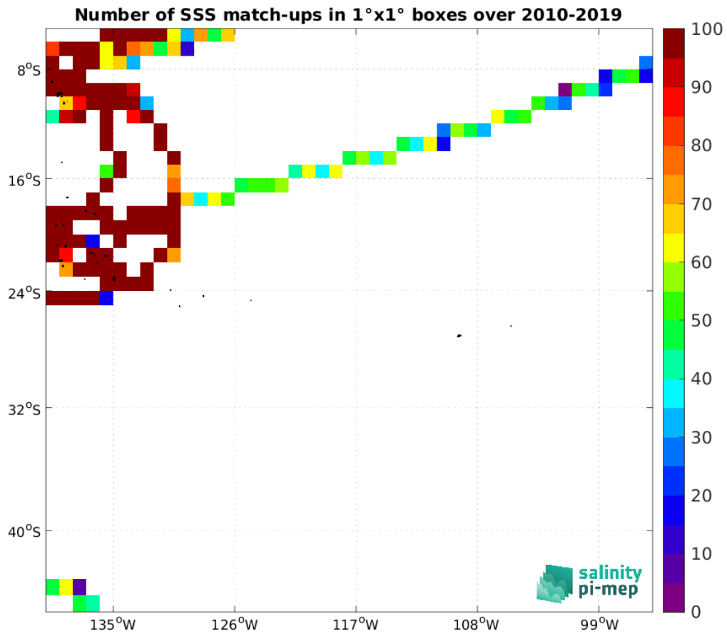
Figure 5: Number of SSS match-ups between TSG (GOSUD-Research-vessel) SSS and the ISAS v7 - Monthly (Ifremer-LOPS-CMEMS) SSS product for the OTT zone Pi-MEP region over 1^\circ \times 1^\circ boxes and for the full satellite product period.
