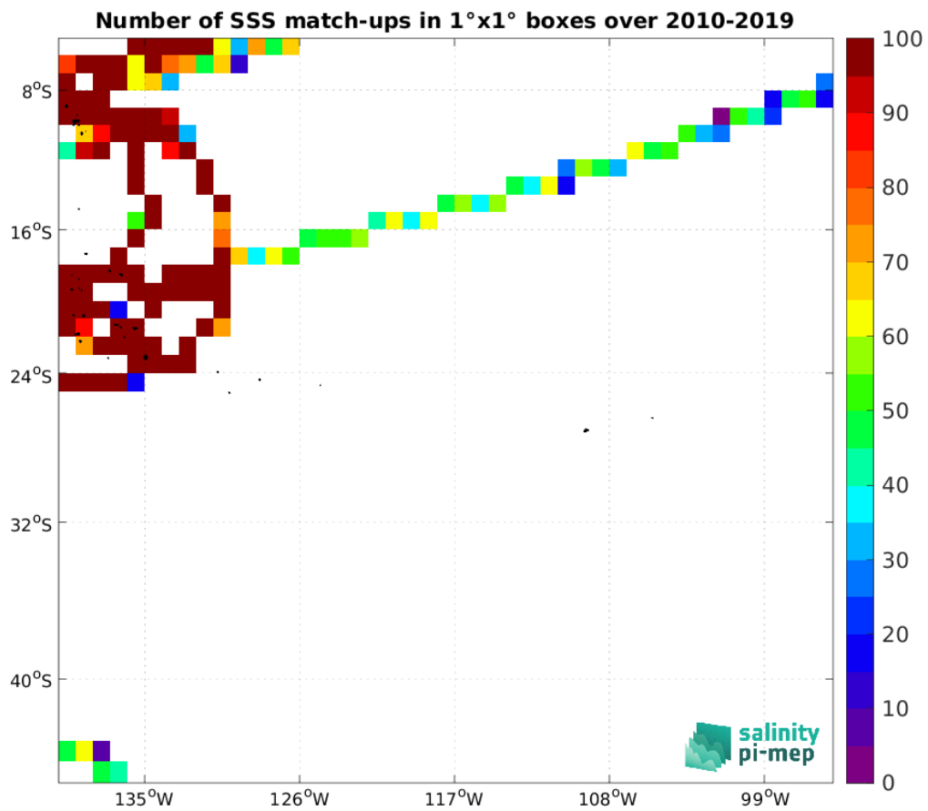
Figure 5: Number of SSS match-ups between TSG (GOSUD-Research-vessel) SSS and the ISAS SSS product for the OTT zone Pi-MEP region over 1^\circ \times 1^\circ boxes and for the full satellite product period.
