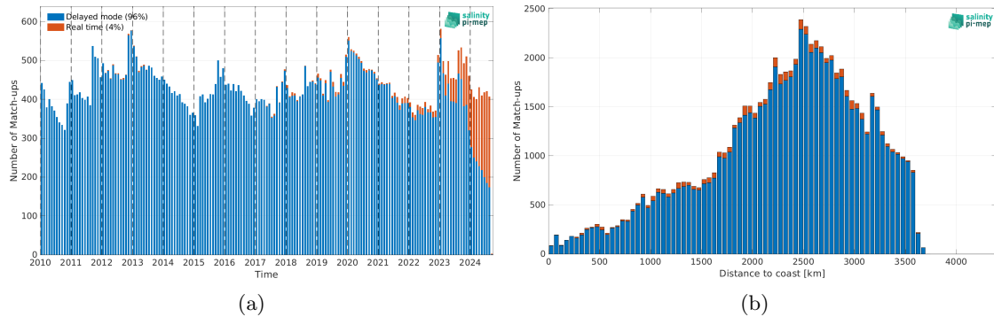
Figure 2: Number of match-ups between Argo and ISAS v7 - Monthly (Ifremer-LOPS-CMEMS) SSS as a function of time (a) and as function of the distance to coast (b) over the OTT zone Pi-MEP region and for the full satellite product period.
