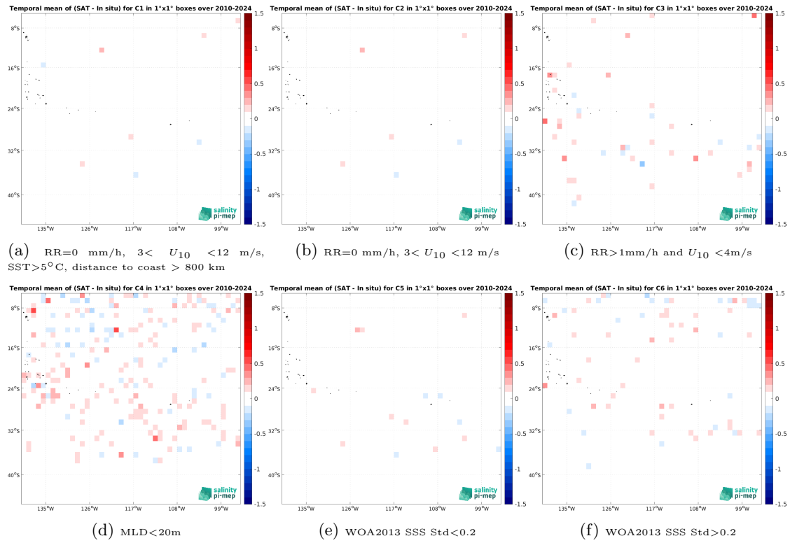
Figure 14: Temporal mean gridded over spatial boxes of size 1^\circ \times 1^\circ of \Delta\text{SSS} (ISAS v7 - Monthly (Ifremer-LOPS-CMEMS) - Argo) for 6 different subdatasets corresponding to:RR=0 mm/h, 3 < U_{10} < 12 m/s, SST>5°C, distance to coast > 800 km (a), RR=0 mm/h, 3 < U_{10} < 12 m/s (b), RR>1mm/h and U_{10} < 4 m/s (c),MLD<20m (d),WOA2013 SSS Std<0.2 (e),WOA2013 SSS Std>0.2 (f).
