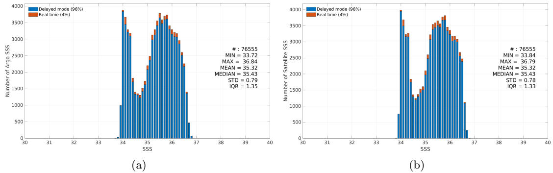
Figure 3: Histograms of SSS from Argo (a) and ISAS v7 - Monthly (Ifremer-LOPS-CMEMS) (b) considering all match-up pairs per bins of 0.1 over the OTT zone Pi-MEP region and for the full satellite product period.
