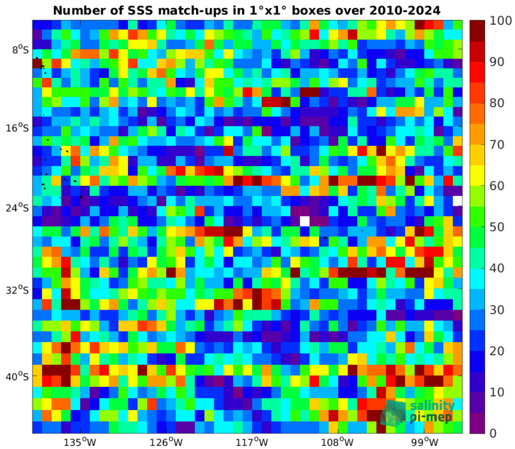
Figure 5: Number of SSS match-ups between Argo SSS and the ISAS v7 - Monthly (Ifremer-LOPS-CMEMS) SSS product for the OTT zone Pi-MEP region over 1^\circ \times 1^\circ boxes and for the full satellite product period.
