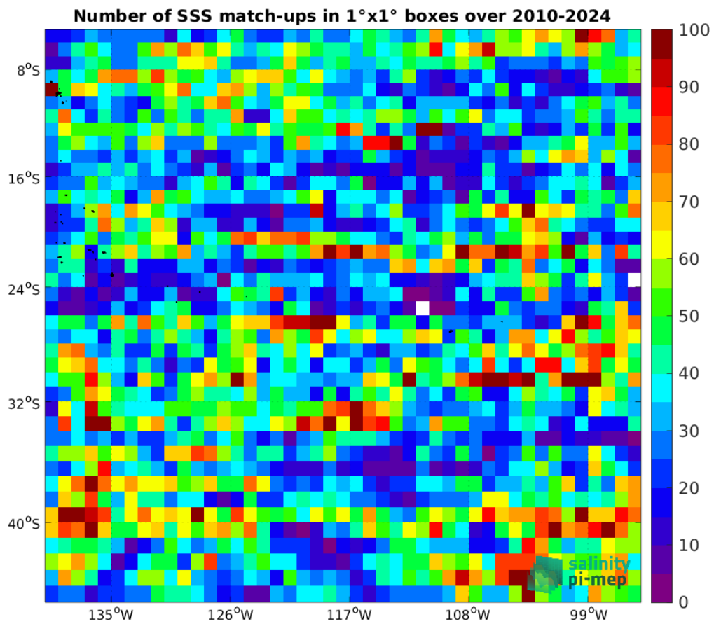
Figure 5: Number of SSS match-ups between Argo SSS and the ISAS SSS product for the OTT zone Pi-MEP region over 1°x1° boxes and for the full satellite product period.
