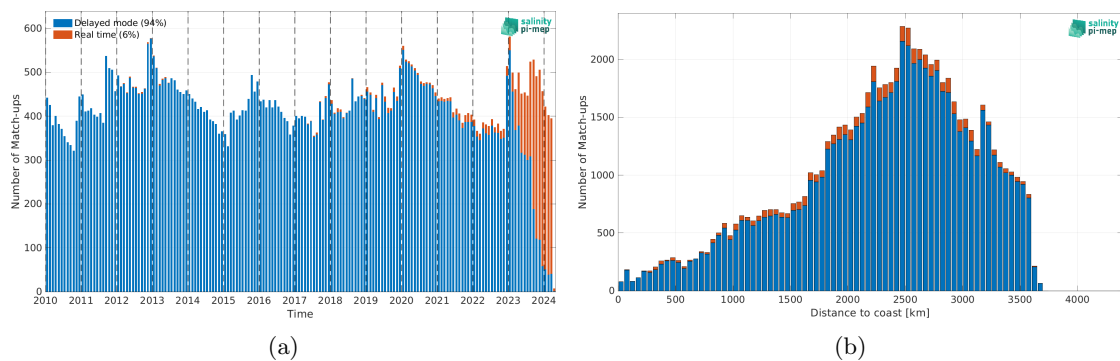
Figure 2: Number of match-ups between Argo and ISAS SSS as a function of time (a) and as function of the distance to coast (b) over the OTT zone Pi-MEP region and for the full satellite product period.
