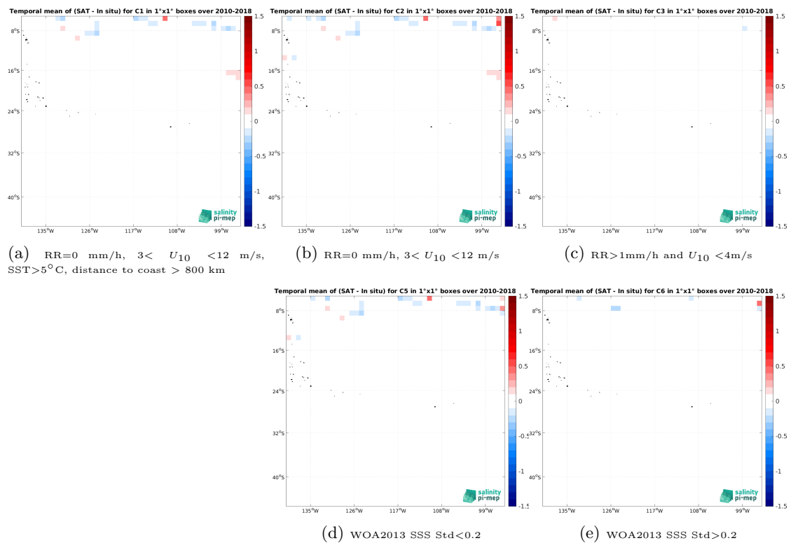
Figure 14: Temporal mean gridded over spatial boxes of size 1^\circ \times 1^\circ of \Delta SSS (CCI SSS L4 Merged-OI v5.5 - 7-day running (ESA) - TSG (SAMOS)) for 5 different subdatasets corresponding to:RR=0 mm/h, 3 < U_{10} < 12 m/s, SST >5^\circ C, distance to coast > 800 km (a), RR=0 mm/h, 3 < U_{10} < 12 m/s (b), RR >1 mm/h and U_{10} < 4 m/s (c), WOA2013 SSS Std <0.2 (d), WOA2013 SSS Std >0.2 (e).
