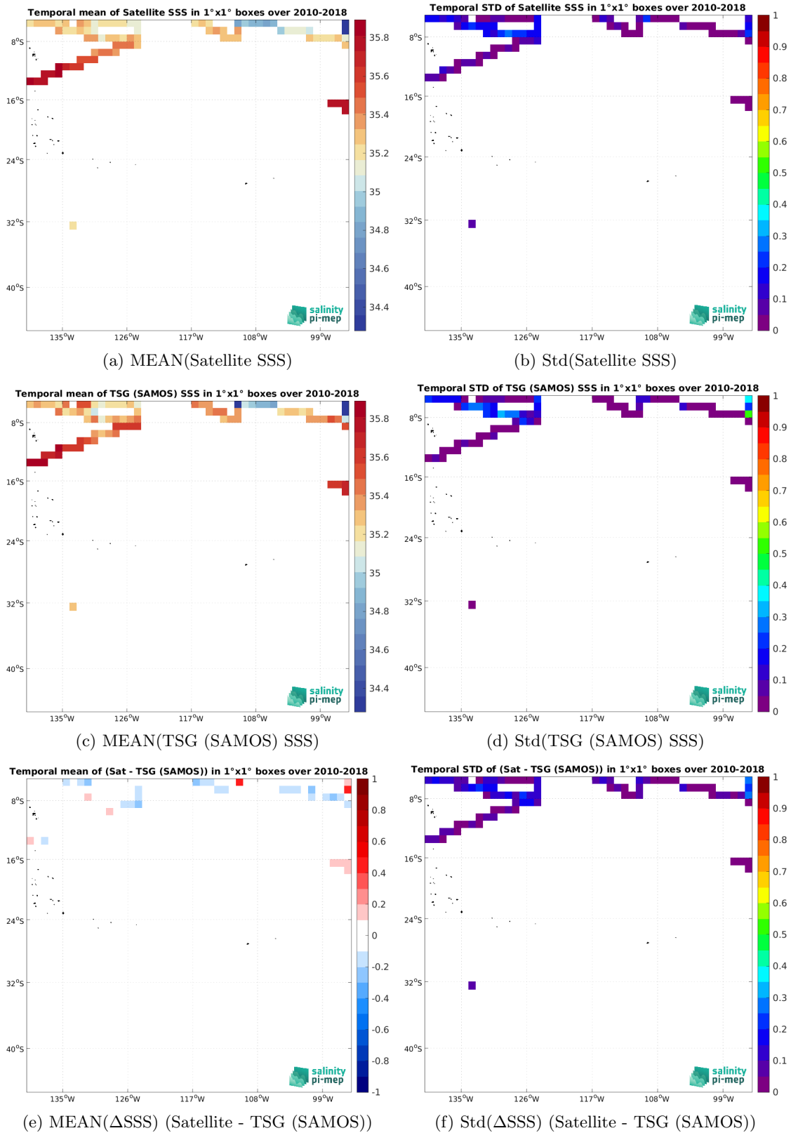
Figure 7: Temporal mean (left) and Std (right) of SSS from CCI SSS L4 Merged-OI v5.5 - 7-day running (ESA) (top), TSG (SAMOS) (middle), and of \Delta SSS (Satellite - TSG (SAMOS)). Only match-up pairs are used to generate these maps.
