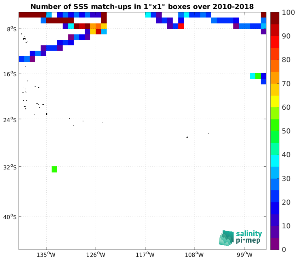
Figure 5: Number of SSS match-ups between TSG (SAMOS) SSS and the CCI SSS L4 Merged-OI v5.5 - 7-day running (ESA) SSS product for the OTT zone Pi-MEP region over 1^\circ \times 1^\circ boxes and for the full satellite product period.
