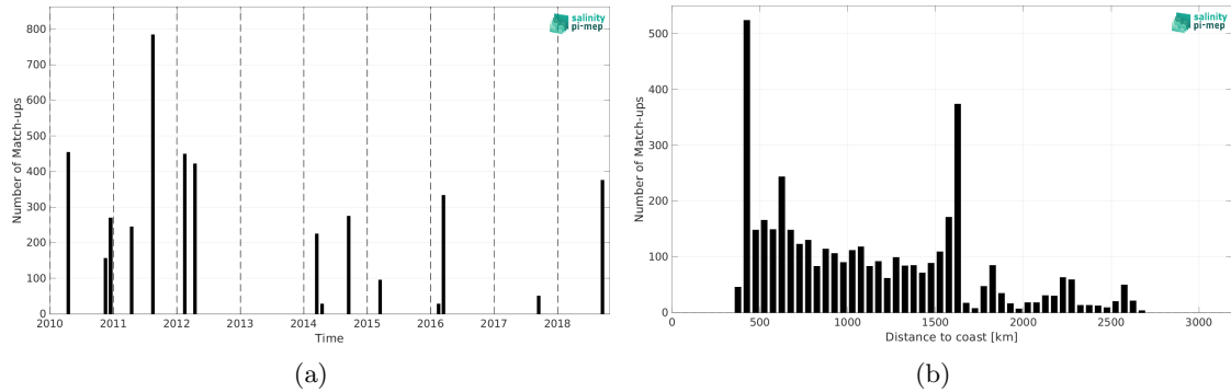
Figure 2: Number of match-ups between TSG (SAMOS) and CCI SSS L4 Merged-OI v5.5 - 7-day running (ESA) SSS as a function of time (a) and as function of the distance to coast (b) over the OTT zone Pi-MEP region and for the full satellite product period.
