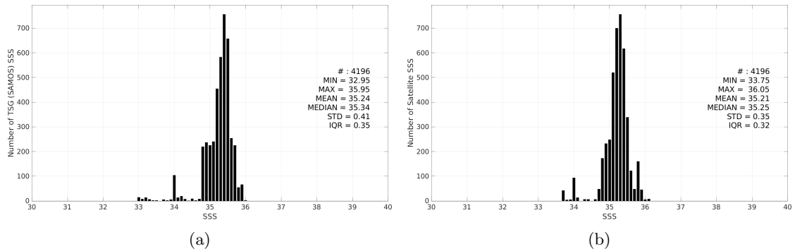
Figure 3: Histograms of SSS from TSG (SAMOS) (a) and CCI SSS L4 Merged-OI v5.5 - 7-day running (ESA) (b) considering all match-up pairs per bins of 0.1 over the OTT zone Pi-MEP region and for the full satellite product period.
