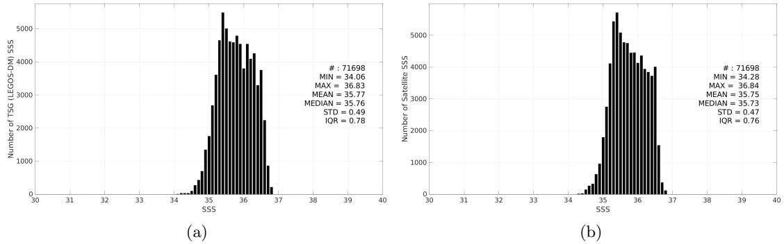
Figure 3: Histograms of SSS from TSG (LEGOS-DM) (a) and CCI SSS L4 Merged-OI v5.5 - 7-day running (ESA) (b) considering all match-up pairs per bins of 0.1 over the OTT zone Pi-MEP region and for the full satellite product period.
