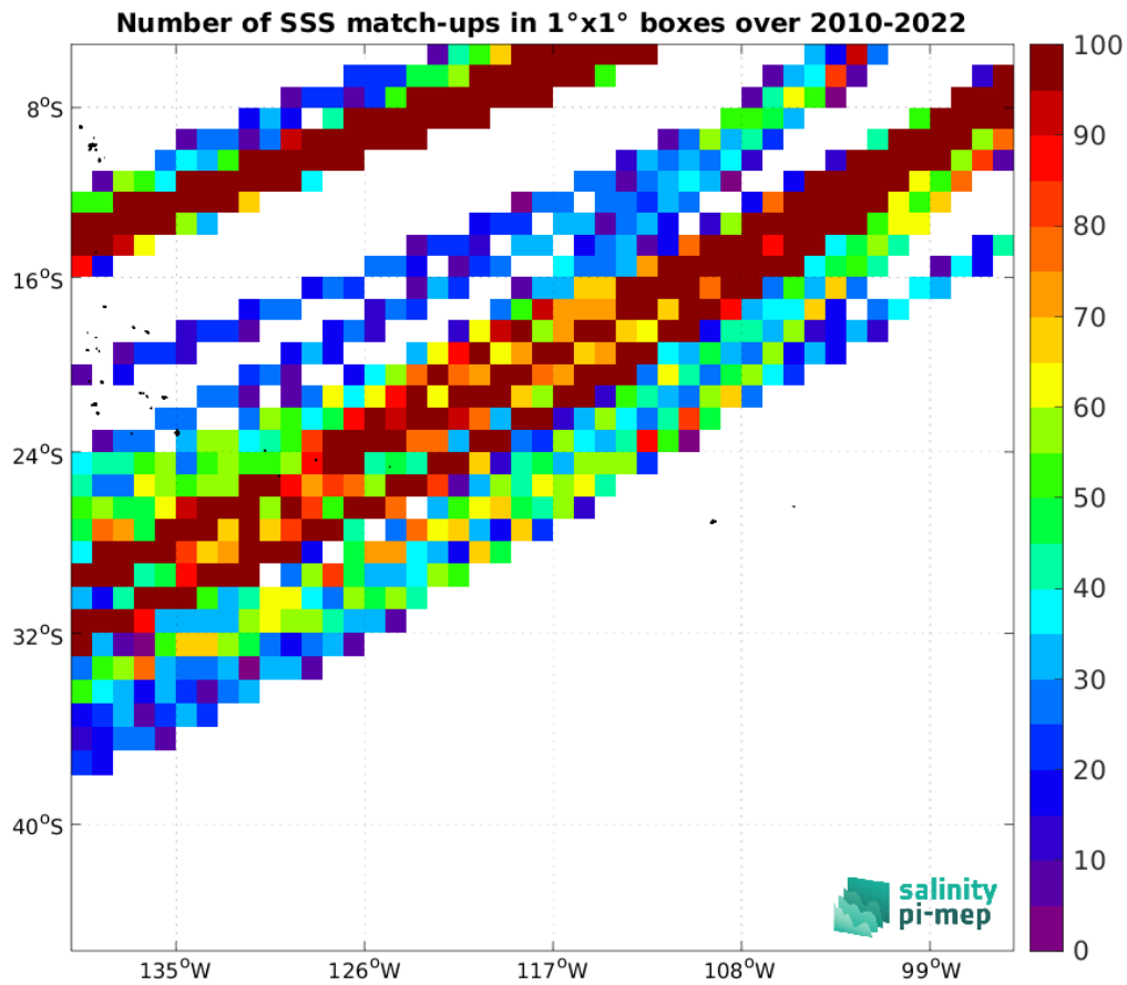
Figure 5: Number of SSS match-ups between TSG (LEGOS-DM) SSS and the CCI SSS L4 Merged-OI v5.5 - 7-day running (ESA) SSS product for the OTT zone Pi-MEP region over 1°x1° boxes and for the full satellite product period.
