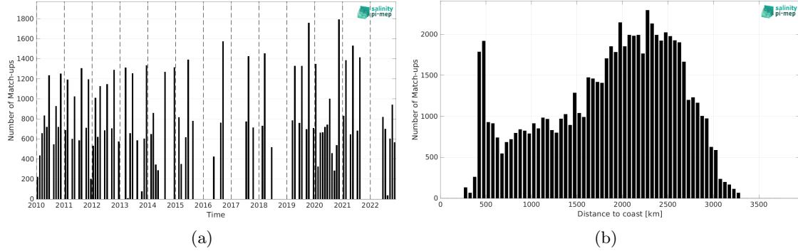
Figure 2: Number of match-ups between TSG (LEGOS-DM) and CCI SSS L4 Merged-OI v5.5 - 7-day running (ESA) SSS as a function of time (a) and as function of the distance to coast (b) over the OTT zone Pi-MEP region and for the full satellite product period.
