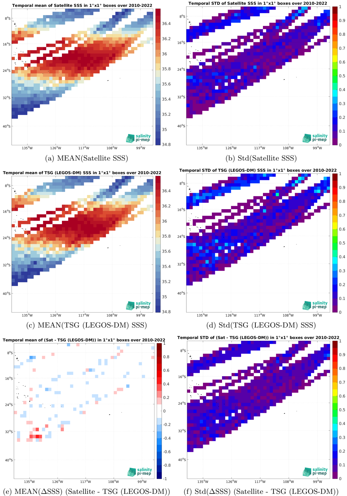
Figure 7: Temporal mean (left) and Std (right) of SSS from CCI SSS L4 Merged-OI v5.5 - 7-day running (ESA) (top), TSG (LEGOS-DM) (middle), and of \Delta SSS (Satellite - TSG (LEGOS-DM)). Only match-up pairs are used to generate these maps.
