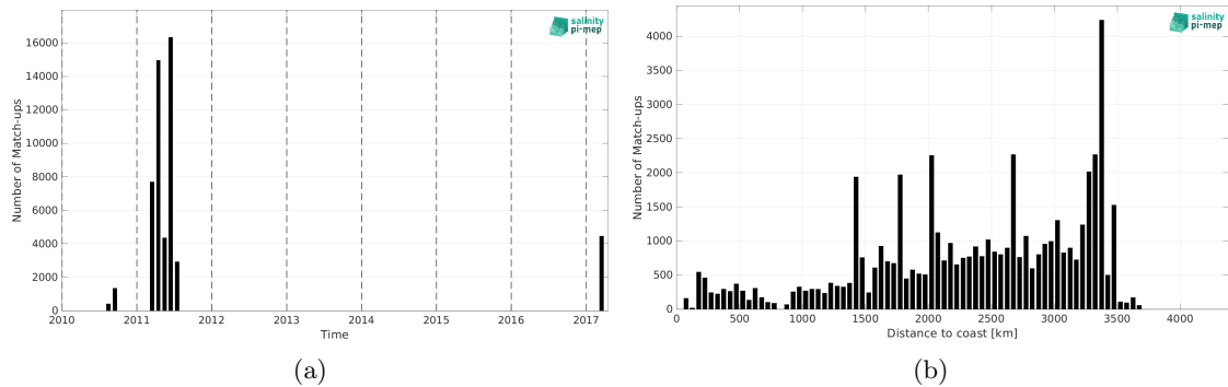
Figure 2: Number of match-ups between TSG (GOSUD-Sailing-ship) and CCI SSS L4 Merged-OI v5.5 - 7-day running (ESA) SSS as a function of time (a) and as function of the distance to coast (b) over the OTT zone Pi-MEP region and for the full satellite product period.
