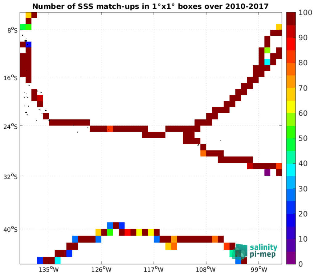
Figure 5: Number of SSS match-ups between TSG (GOSUD-Sailing-ship) SSS and the CCI SSS L4 Merged-OI v5.5 - 7-day running (ESA) SSS product for the OTT zone Pi-MEP region over 1^\circ \times 1^\circ boxes and for the full satellite product period.
