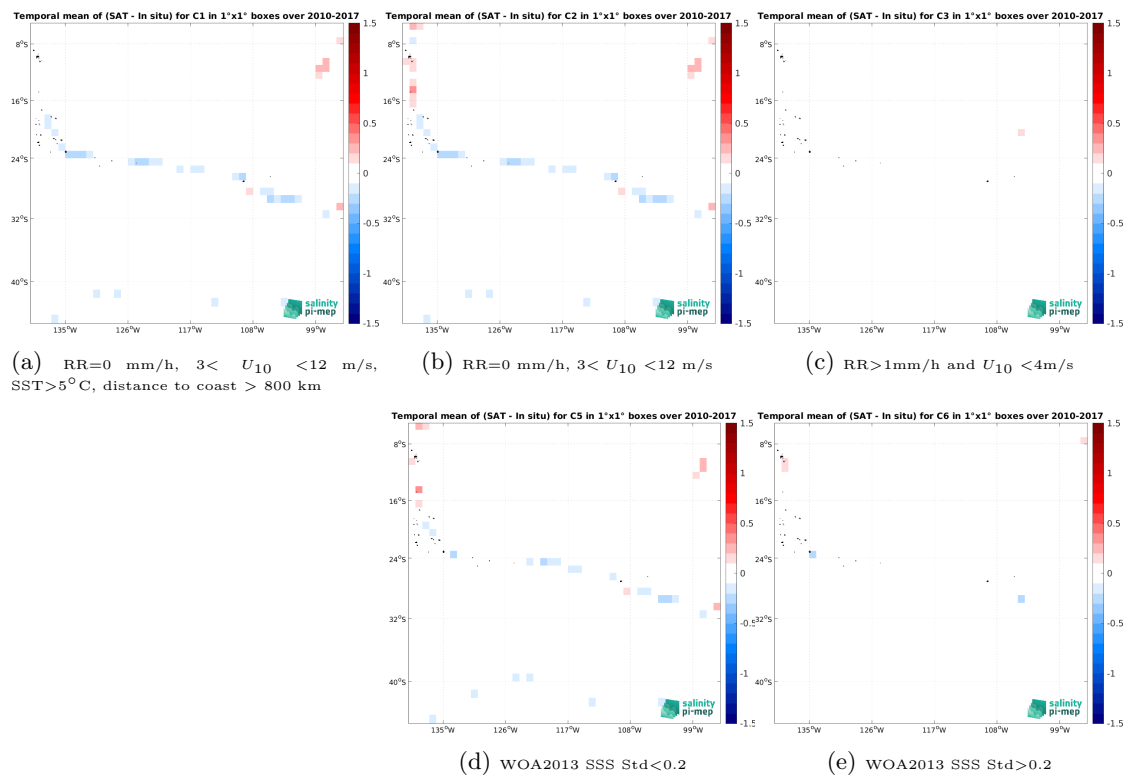
Figure 14: Temporal mean gridded over spatial boxes of size 1^\circ \times 1^\circ of \Delta SSS (CCI SSS L4 Merged-OI v5.5 - 7-day running (ESA) - TSG (GOSUD-Sailing-ship)) for 5 different subdatasets corresponding to:RR=0 mm/h, 3 < U_{10} < 12 m/s, SST >5^\circ\text{C} , distance to coast > 800 km (a), RR=0 mm/h, 3 < U_{10} < 12 m/s (b), RR >1 mm/h and U_{10} < 4 m/s (c), WOA2013 SSS Std <0.2 (d), WOA2013 SSS Std >0.2 (e).
