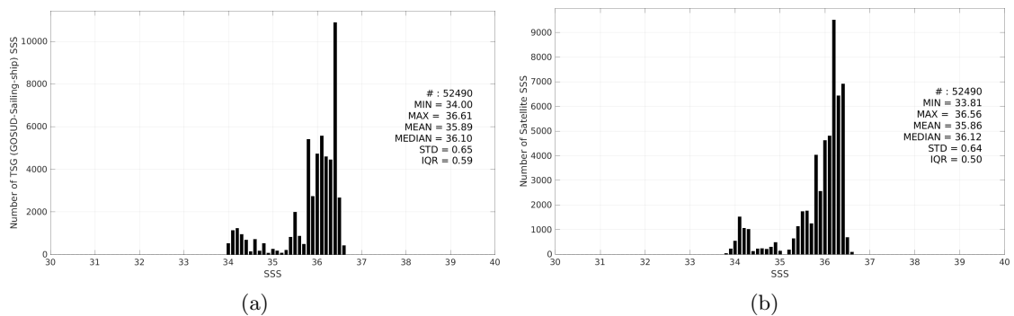
Figure 3: Histograms of SSS from TSG (GOSUD-Sailing-ship) (a) and CCI SSS L4 Merged-OI v5.5 - 7-day running (ESA) (b) considering all match-up pairs per bins of 0.1 over the OTT zone Pi-MEP region and for the full satellite product period.
