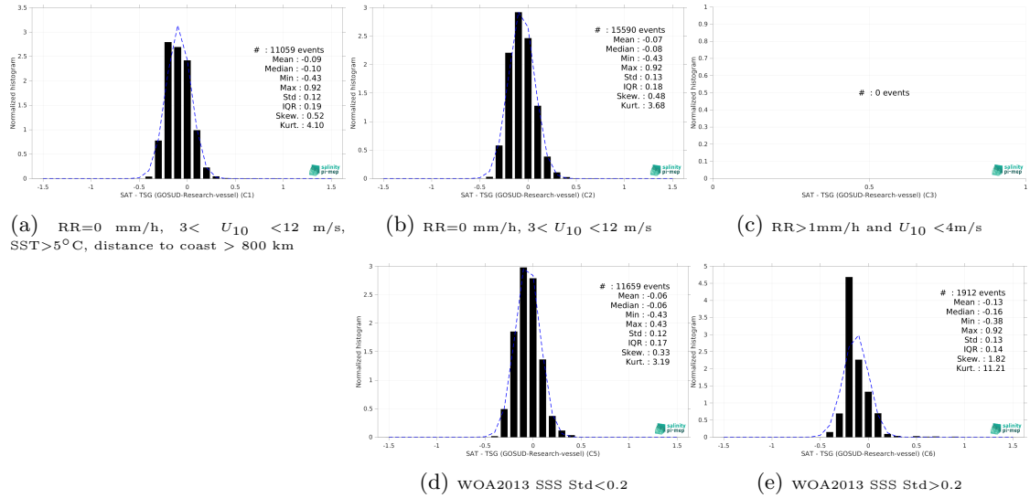
Figure 15: Normalized histogram of \Delta SSS (CCI SSS L4 Merged-OI v5.5 - 7-day running (ESA) - TSG (GOSUD-Research-vessel)) for 5 different subdatasets corresponding to: RR=0 mm/h, 3 < U_{10} < 12 m/s, SST > 5°C, distance to coast > 800 km (a), RR=0 mm/h, 3 < U_{10} < 12 m/s (b), RR > 1mm/h and U_{10} < 4 m/s (c), WOA2013 SSS Std < 0.2 (d), WOA2013 SSS Std > 0.2 (e).
