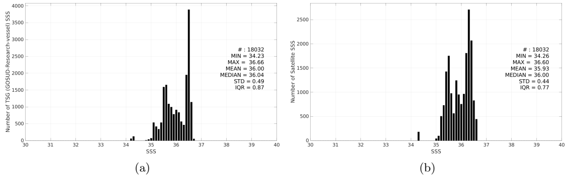
Figure 3: Histograms of SSS from TSG (GOSUD-Research-vessel) (a) and CCI SSS L4 Merged-OI v5.5 - 7-day running (ESA) (b) considering all match-up pairs per bins of 0.1 over the OTT zone Pi-MEP region and for the full satellite product period.
