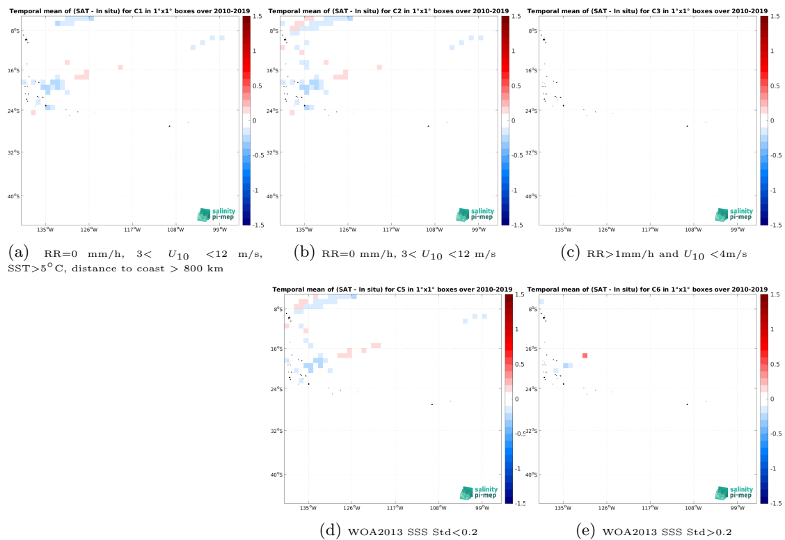
Figure 14: Temporal mean gridded over spatial boxes of size 1^\circ \times 1^\circ of \Delta SSS (CCI SSS L4 Merged-OI v5.5 - 7-day running (ESA) - TSG (GOSUD-Research-vessel)) for 5 different subdatasets corresponding to:RR=0 mm/h, 3 < U_{10} < 12 m/s, SST >5^\circ C, distance to coast > 800 km (a), RR=0 mm/h, 3 < U_{10} < 12 m/s (b), RR >1 mm/h and U_{10} < 4 m/s (c), WOA2013 SSS Std <0.2 (d), WOA2013 SSS Std >0.2 (e).
