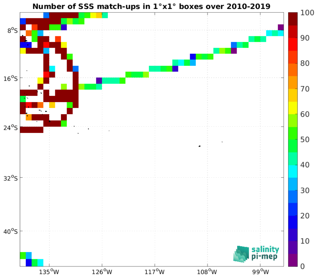
Figure 5: Number of SSS match-ups between TSG (GOSUD-Research-vessel) SSS and the CCI SSS L4 Merged-OI v5.5 - 7-day running (ESA) SSS product for the OTT zone Pi-MEP region over 1^\circ \times 1^\circ boxes and for the full satellite product period.
