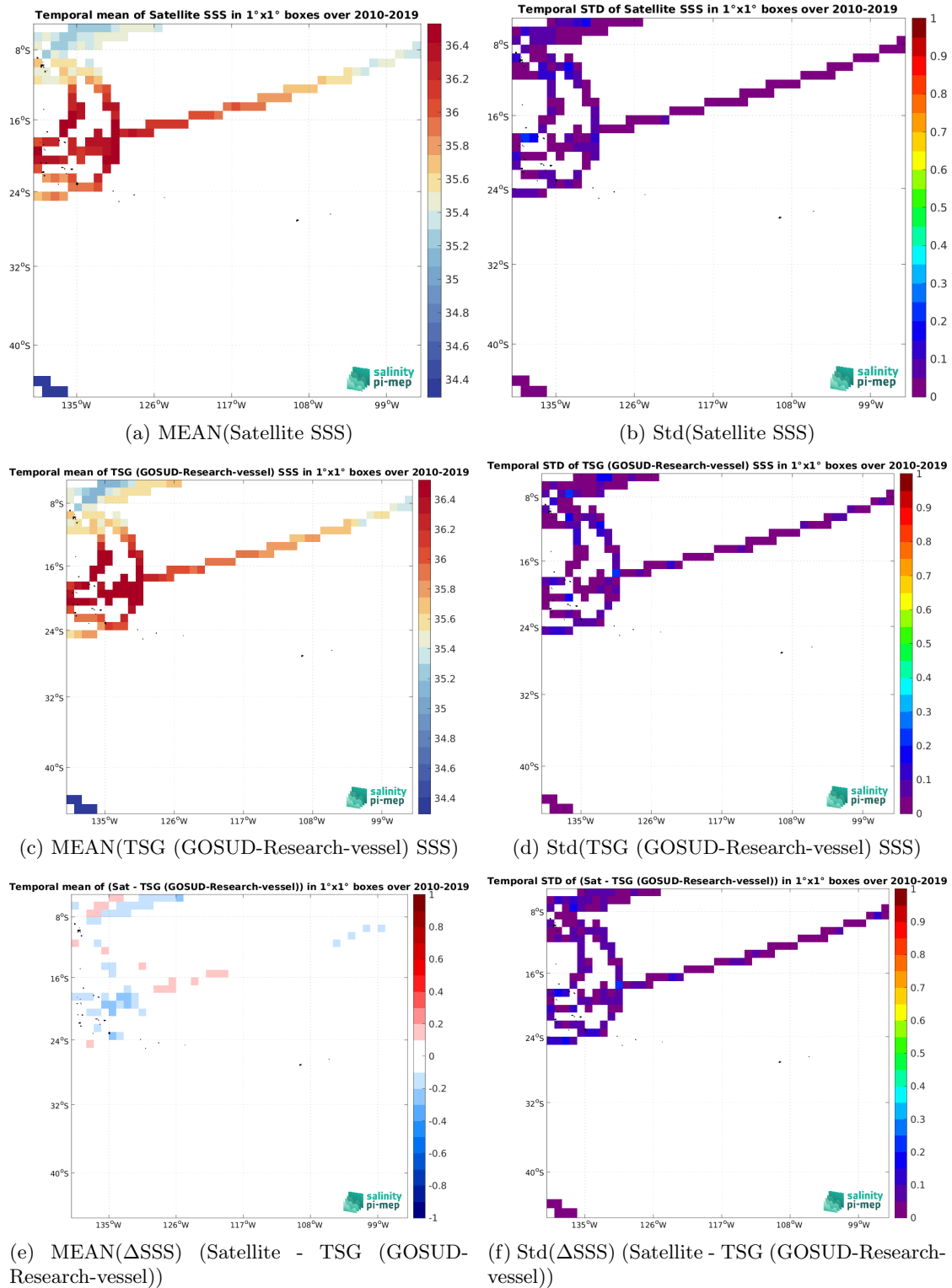
Figure 7: Temporal mean (left) and Std (right) of SSS from CCI SSS L4 Merged-OI v5.5 - 7-day running (ESA) (top), TSG (GOSUD-Research-vessel) (middle), and of \Delta SSS (Satellite - TSG (GOSUD-Research-vessel)). Only match-up pairs are used to generate these maps.
