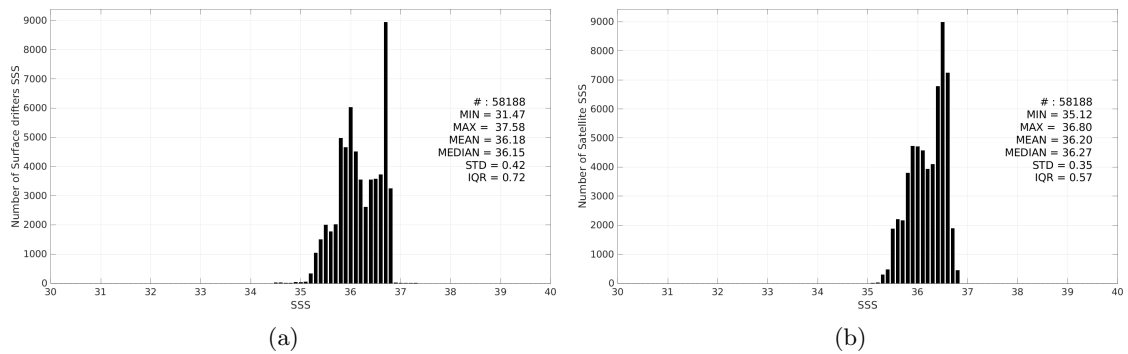
Figure 3: Histograms of SSS from Surface drifters (a) and CCI SSS L4 Merged-OI v5.5 - 7-day running (ESA) (b) considering all match-up pairs per bins of 0.1 over the OTT zone Pi-MEP region and for the full satellite product period.
