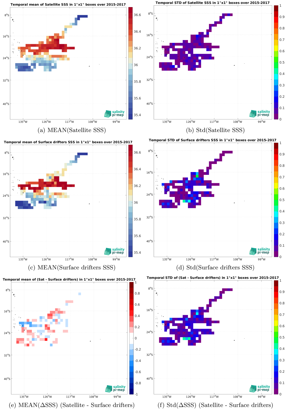
Figure 6: Temporal mean (left) and Std (right) of SSS from CCI SSS L4 Merged-OI v5.5 - 7-day running (ESA) (top), Surface drifters (middle), and of \Delta SSS (Satellite - Surface drifters). Only match-up pairs are used to generate these maps.
