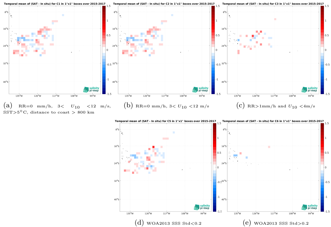
Figure 13: Temporal mean gridded over spatial boxes of size 1^\circ \times 1^\circ of \Delta SSS (CCI SSS L4 Merged-OI v5.5 - 7-day running (ESA) - Surface drifters) for 5 different subdatasets corresponding to:RR=0 mm/h, 3 < U_{10} < 12 m/s, SST > 5^\circ\text{C} , distance to coast > 800 km (a), RR=0 mm/h, 3 < U_{10} < 12 m/s (b), RR > 1 mm/h and U_{10} < 4 m/s (c), WOA2013 SSS Std < 0.2 (d), WOA2013 SSS Std > 0.2 (e).
