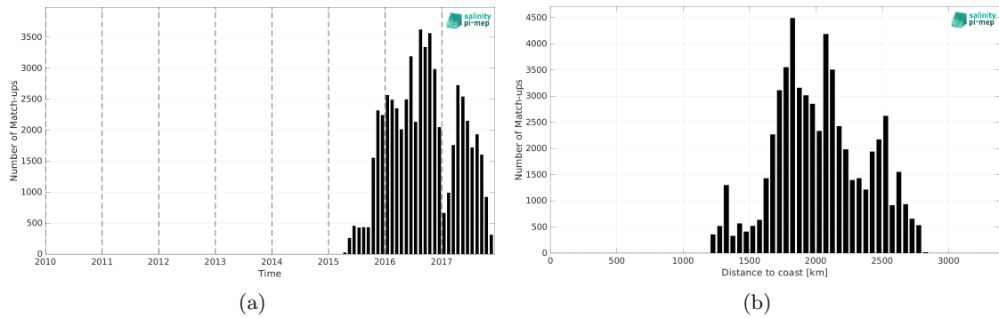
Figure 2: Number of match-ups between Surface drifters and CCI SSS L4 Merged-OI v5.5 - 7-day running (ESA) SSS as a function of time (a) and as function of the distance to coast (b) over the OTT zone Pi-MEP region and for the full satellite product period.
