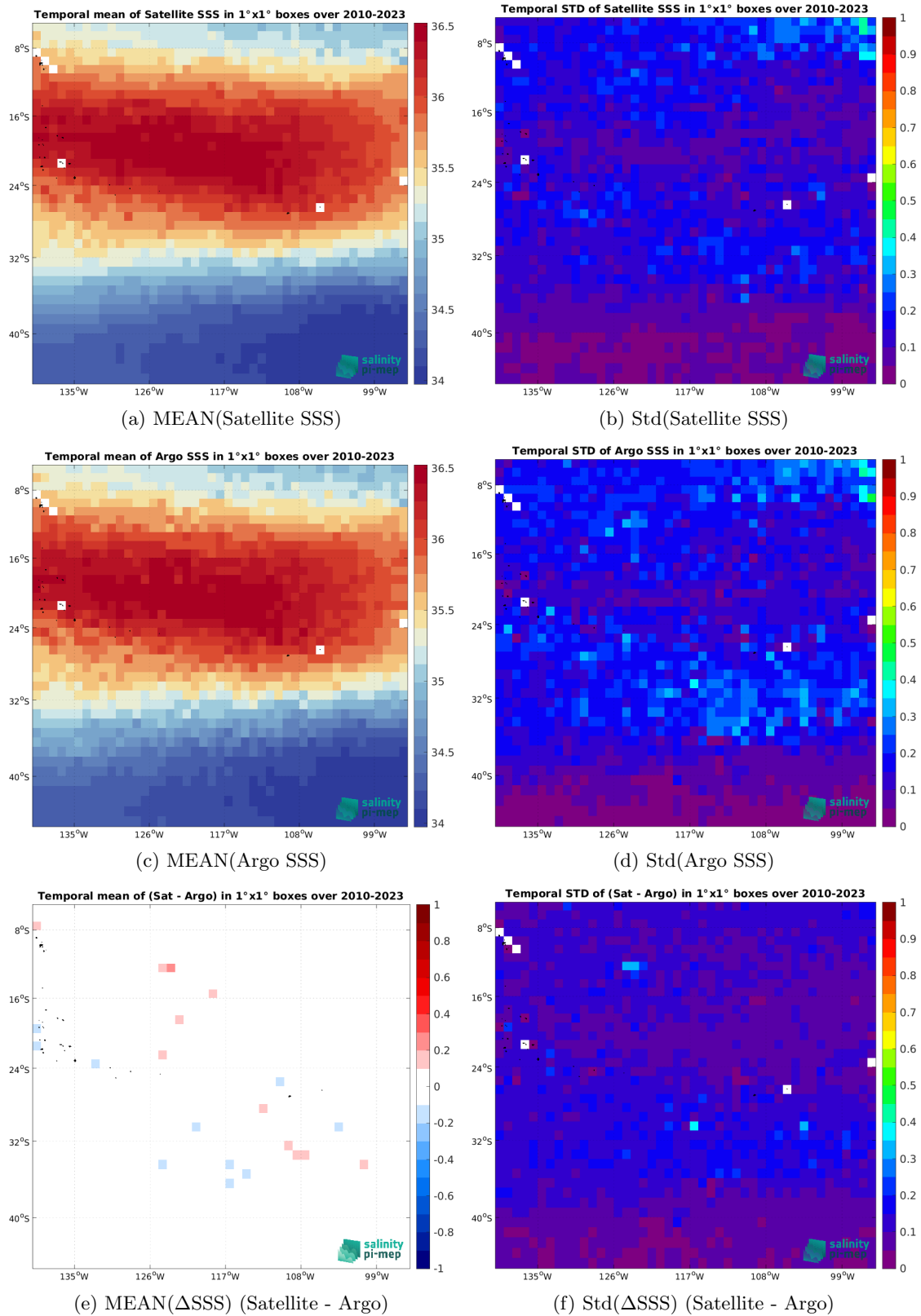
Figure 7: Temporal mean (left) and Std (right) of SSS from CCI SSS L4 Merged-OI v5.5 - 7-day running (ESA) (top), Argo (middle), and of \Delta SSS (Satellite - Argo). Only match-up pairs are used to generate these maps.
