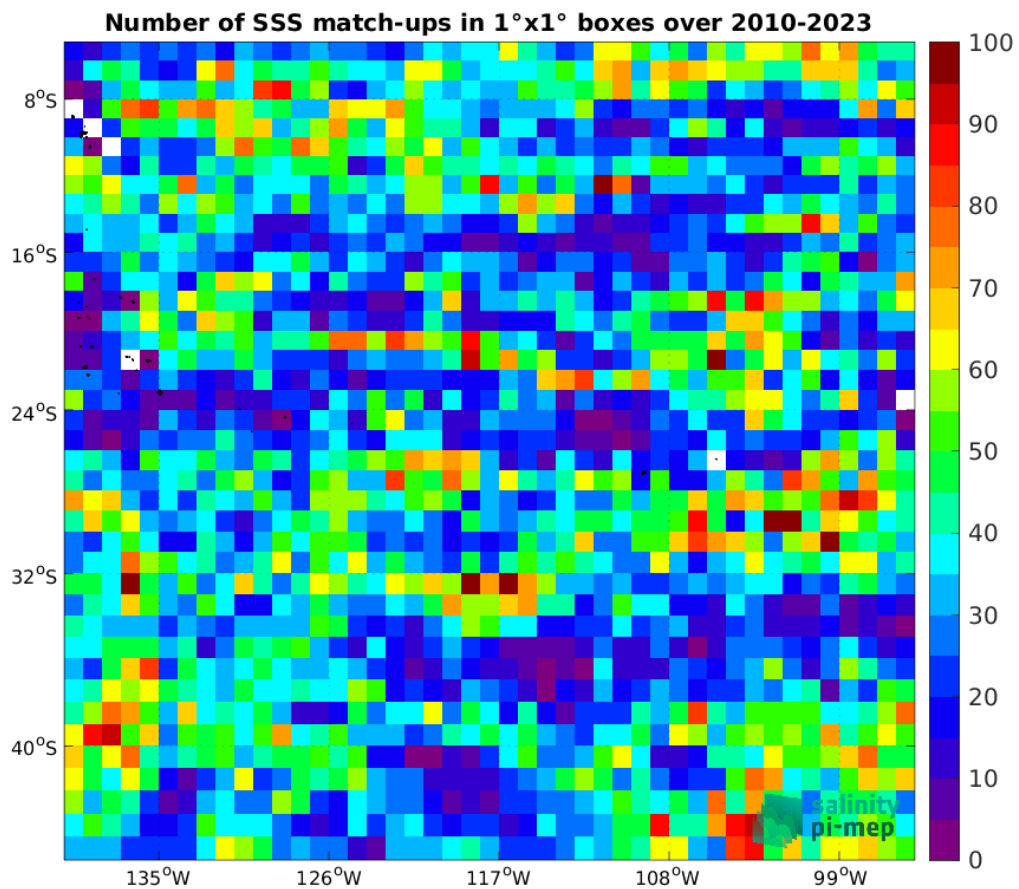
Figure 5: Number of SSS match-ups between Argo SSS and the CCI SSS L4 Merged-OI v5.5 - 7-day running (ESA) SSS product for the OTT zone Pi-MEP region over 1°x1° boxes and for the full satellite product period.
