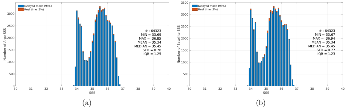
Figure 3: Histograms of SSS from Argo (a) and CCI SSS L4 Merged-OI v5.5 - 7-day running (ESA) (b) considering all match-up pairs per bins of 0.1 over the OTT zone Pi-MEP region and for the full satellite product period.
