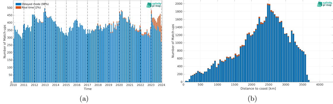
Figure 2: Number of match-ups between Argo and CCI SSS L4 Merged-OI v5.5 - 7-day running (ESA) SSS as a function of time (a) and as function of the distance to coast (b) over the OTT zone Pi-MEP region and for the full satellite product period.
