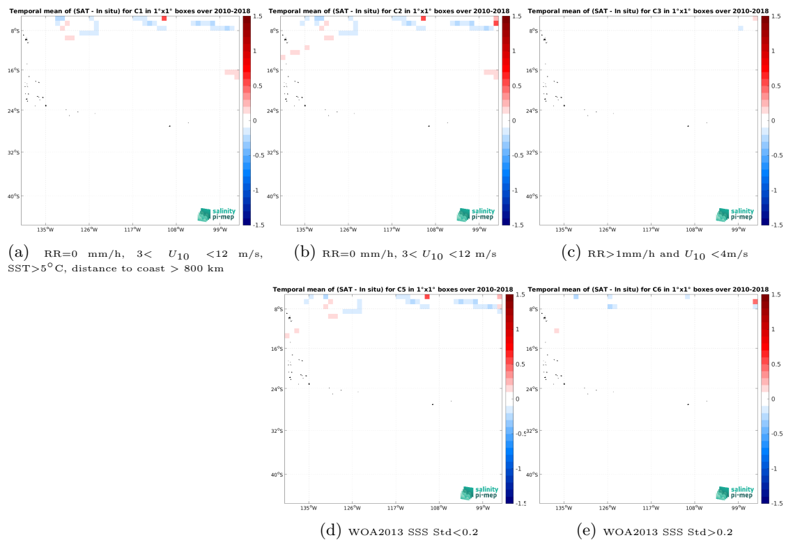
Figure 14: Temporal mean gridded over spatial boxes of size 1^\circ \times 1^\circ of \Delta SSS (CCI SSS L4 Merged-OI v5.5 - 30-day running (ESA) - TSG (SAMOS)) for 5 different subdatasets corresponding to:RR=0 mm/h, 3 < U_{10} < 12 m/s, SST >5^\circ C, distance to coast > 800 km (a), RR=0 mm/h, 3 < U_{10} < 12 m/s (b), RR >1 mm/h and U_{10} < 4 m/s (c), WOA2013 SSS Std <0.2 (d), WOA2013 SSS Std >0.2 (e).
