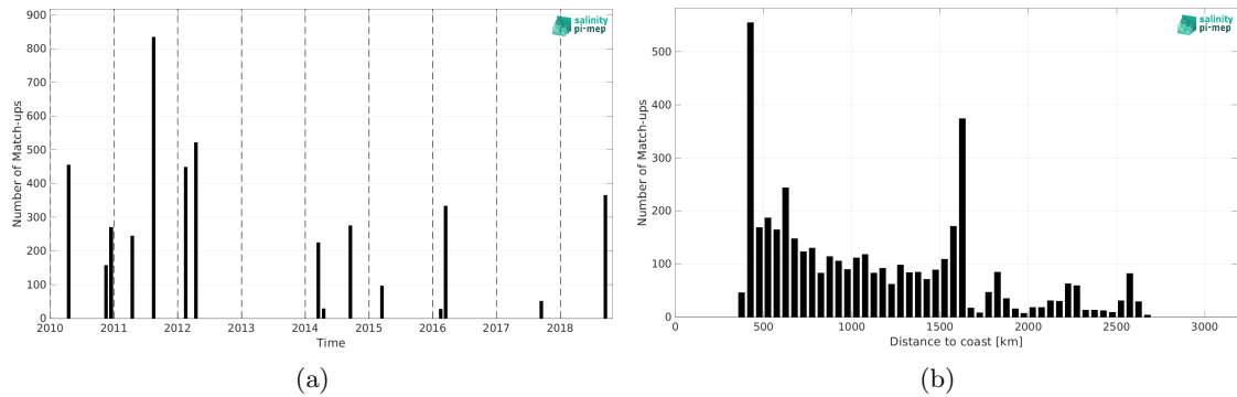
Figure 2: Number of match-ups between TSG (SAMOS) and CCI SSS L4 Merged-OI v5.5 - 30-day running (ESA) SSS as a function of time (a) and as function of the distance to coast (b) over the OTT zone Pi-MEP region and for the full satellite product period.
