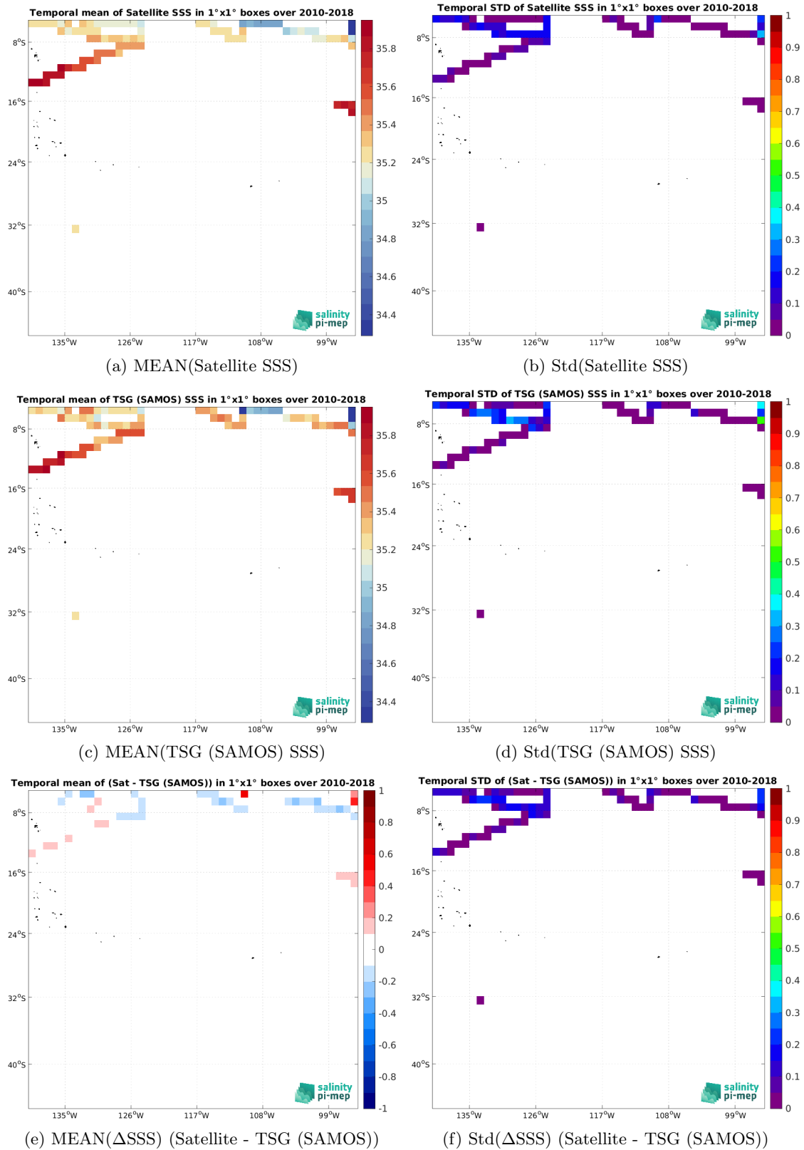
Figure 7: Temporal mean (left) and Std (right) of SSS from CCI SSS L4 Merged-OI v5.5 - 30-day running (ESA) (top), TSG (SAMOS) (middle), and of \Delta SSS (Satellite - TSG (SAMOS)). Only match-up pairs are used to generate these maps.
