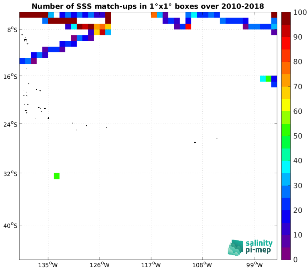
Figure 5: Number of SSS match-ups between TSG (SAMOS) SSS and the CCI SSS L4 Merged-OI v5.5 - 30-day running (ESA) SSS product for the OTT zone Pi-MEP region over 1^\circ \times 1^\circ boxes and for the full satellite product period.
