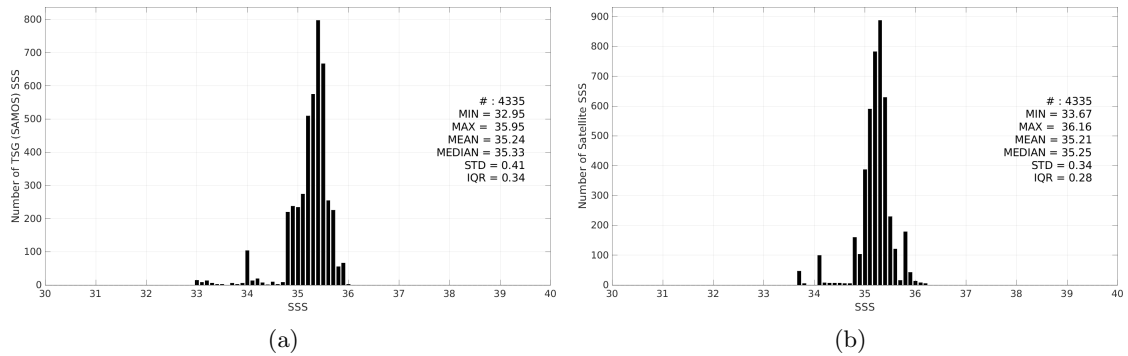
Figure 3: Histograms of SSS from TSG (SAMOS) (a) and CCI SSS L4 Merged-OI v5.5 - 30-day running (ESA) (b) considering all match-up pairs per bins of 0.1 over the OTT zone Pi-MEP region and for the full satellite product period.
