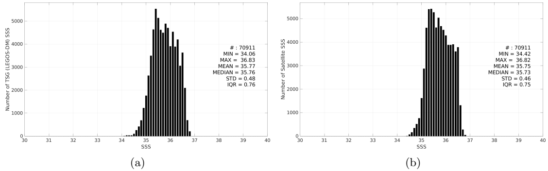
Figure 3: Histograms of SSS from TSG (LEGOS-DM) (a) and CCI SSS L4 Merged-OI v5.5 - 30-day running (ESA) (b) considering all match-up pairs per bins of 0.1 over the OTT zone Pi-MEP region and for the full satellite product period.
