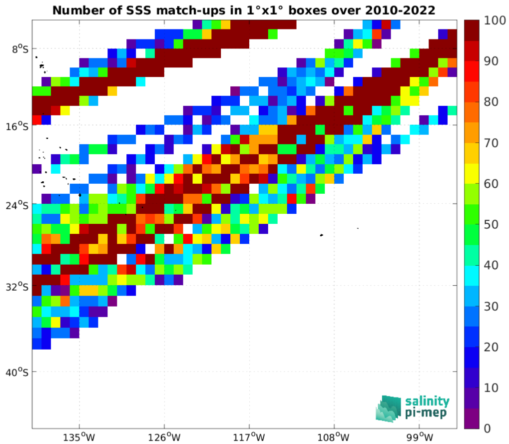
Figure 5: Number of SSS match-ups between TSG (LEGOS-DM) SSS and the CCI SSS L4 Merged-OI v5.5 - 30-day running (ESA) SSS product for the OTT zone Pi-MEP region over 1^\circ \times 1^\circ boxes and for the full satellite product period.
