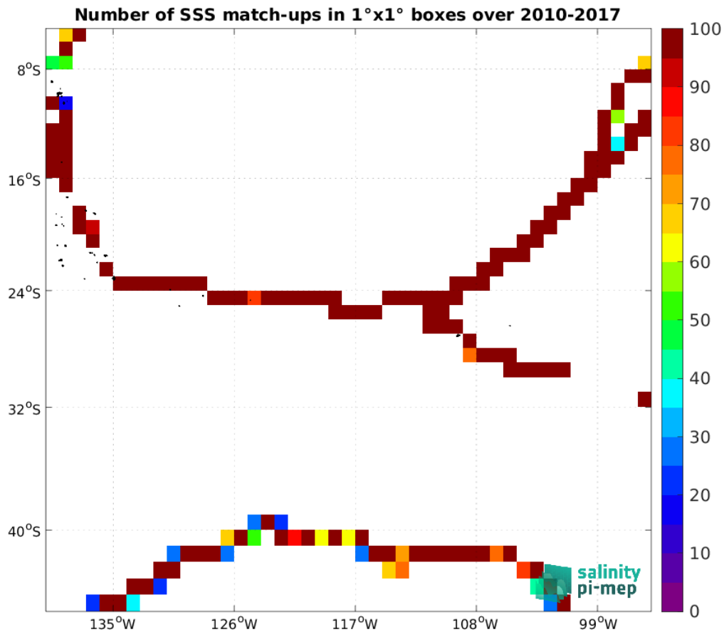
Figure 5: Number of SSS match-ups between TSG (GOSUD-Sailing-ship) SSS and the CCI SSS L4 Merged-OI v5.5 - 30-day running (ESA) SSS product for the OTT zone Pi-MEP region over 1^\circ \times 1^\circ boxes and for the full satellite product period.
