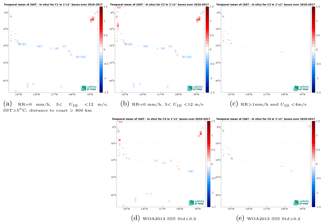
Figure 14: Temporal mean gridded over spatial boxes of size 1^\circ \times 1^\circ of \Delta\text{SSS} (CCI SSS L4 Merged-OI v5.5 - 30-day running (ESA) - TSG (GOSUD-Sailing-ship)) for 5 different subdatasets corresponding to:RR=0 mm/h, 3 < U_{10} < 12 m/s, SST >5^\circ\text{C} , distance to coast > 800 km (a), RR=0 mm/h, 3 < U_{10} < 12 m/s (b), RR >1 mm/h and U_{10} < 4 m/s (c), WOA2013 SSS Std <0.2 (d), WOA2013 SSS Std >0.2 (e).
