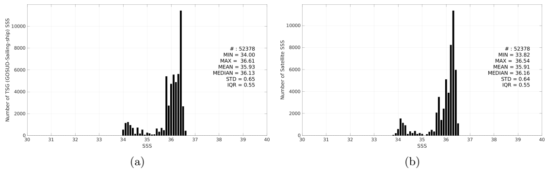
Figure 3: Histograms of SSS from TSG (GOSUD-Sailing-ship) (a) and CCI SSS L4 Merged-OI v5.5 - 30-day running (ESA) (b) considering all match-up pairs per bins of 0.1 over the OTT zone Pi-MEP region and for the full satellite product period.
