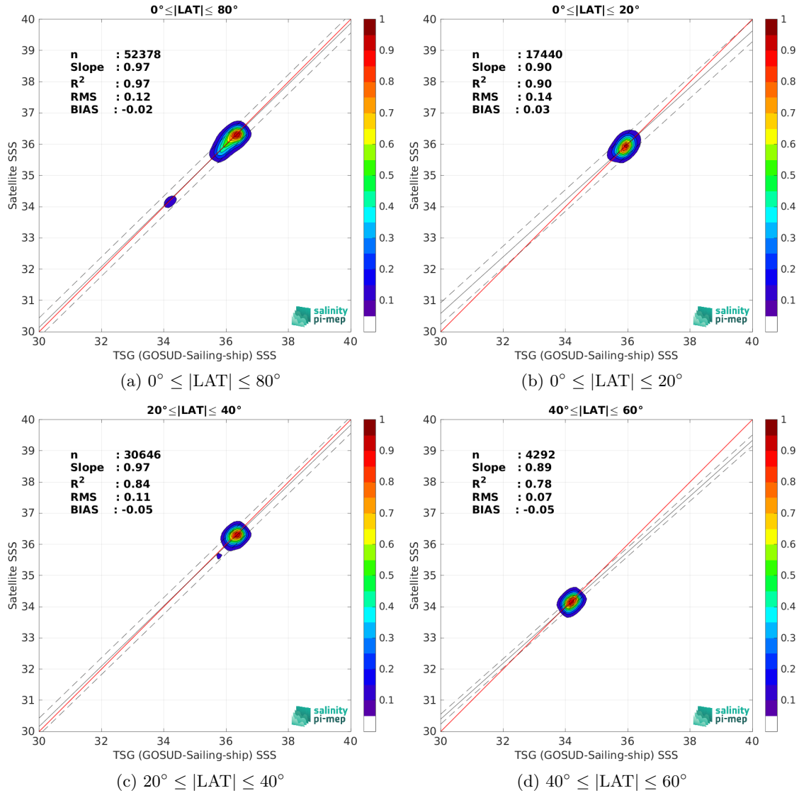
Figure 10: Contour maps of the concentration of CCI SSS L4 Merged-OI v5.5 - 30-day running (ESA) SSS (y-axis) versus TSG (GOSUD-Sailing-ship) SSS (x-axis) at match-up pairs for different latitude bands. For each plot, the red line shows x=y . The black thin and dashed lines indicate a linear fit through the data cloud and the \pm 95\% confidence levels, respectively. The number match-up pairs n , the slope and R^2 coefficient of the linear fit, the root mean square (RMS) and the mean bias between satellite and in situ data are indicated for each latitude band in each plots.
