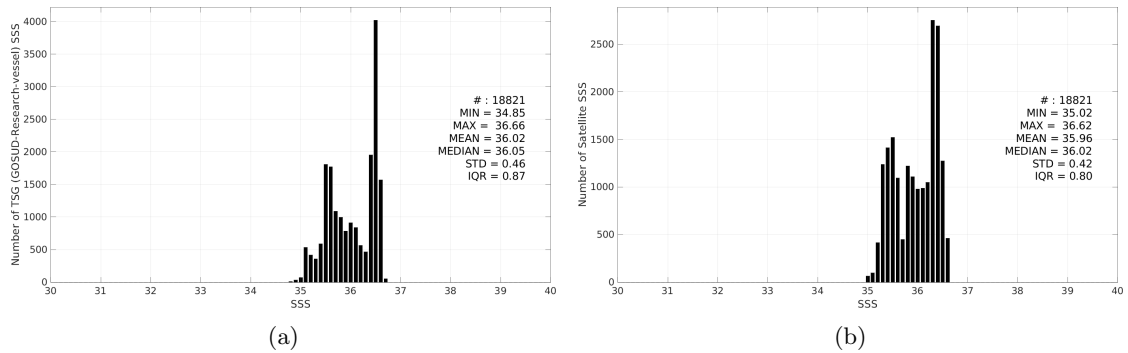
Figure 3: Histograms of SSS from TSG (GOSUD-Research-vessel) (a) and CCI SSS L4 Merged-OI v5.5 - 30-day running (ESA) (b) considering all match-up pairs per bins of 0.1 over the OTT zone Pi-MEP region and for the full satellite product period.
