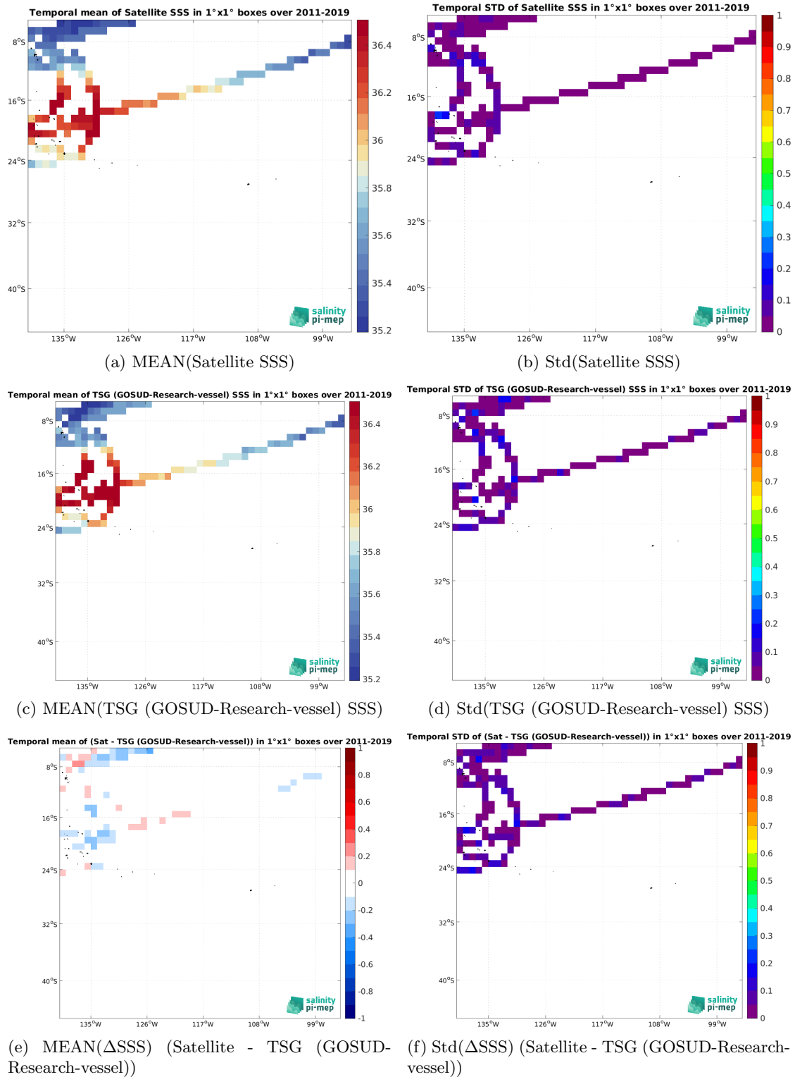
Figure 7: Temporal mean (left) and Std (right) of SSS from CCI SSS L4 Merged-OI v5.5 - 30-day running (ESA) (top), TSG (GOSUD-Research-vessel) (middle), and of \Delta SSS (Satellite - TSG (GOSUD-Research-vessel)). Only match-up pairs are used to generate these maps.
