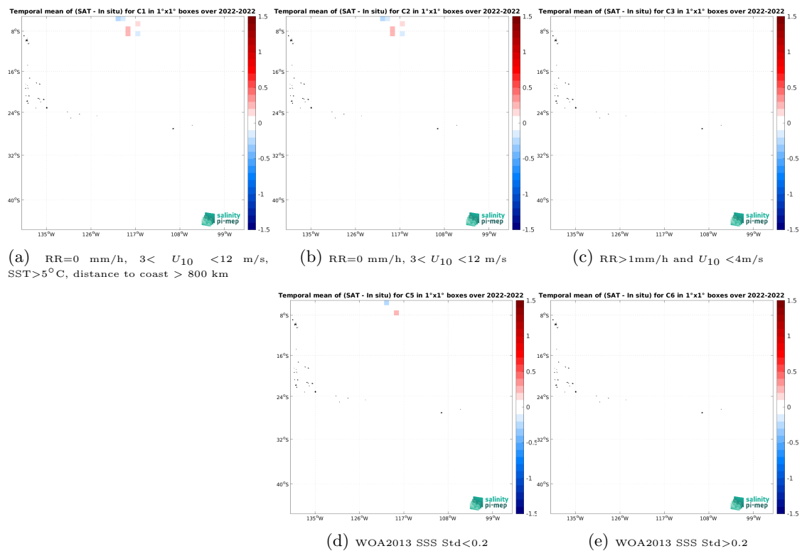
Figure 14: Temporal mean gridded over spatial boxes of size 1^\circ \times 1^\circ of \Delta SSS (CCI SSS L4 Merged-OI v5.5 - 30-day running (ESA) - Saildrone) for 5 different subdatasets corresponding to:RR=0 mm/h, 3 < U_{10} < 12 m/s, SST >5^\circ\text{C} , distance to coast > 800 km (a), RR=0 mm/h, 3 < U_{10} < 12 m/s (b), RR >1 mm/h and U_{10} < 4 m/s (c), WOA2013 SSS Std <0.2 (d), WOA2013 SSS Std >0.2 (e).
