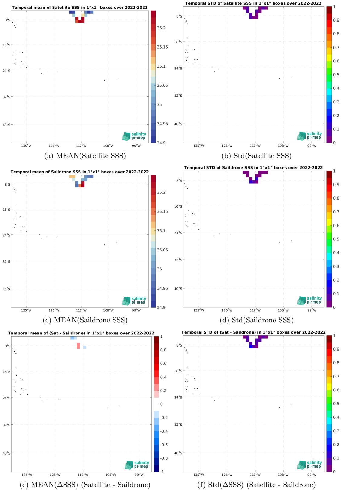
Figure 7: Temporal mean (left) and Std (right) of SSS from CCI SSS L4 Merged-OI v5.5 - 30-day running (ESA) (top), Saildrone (middle), and of \Delta SSS (Satellite - Saildrone). Only match-up pairs are used to generate these maps.
