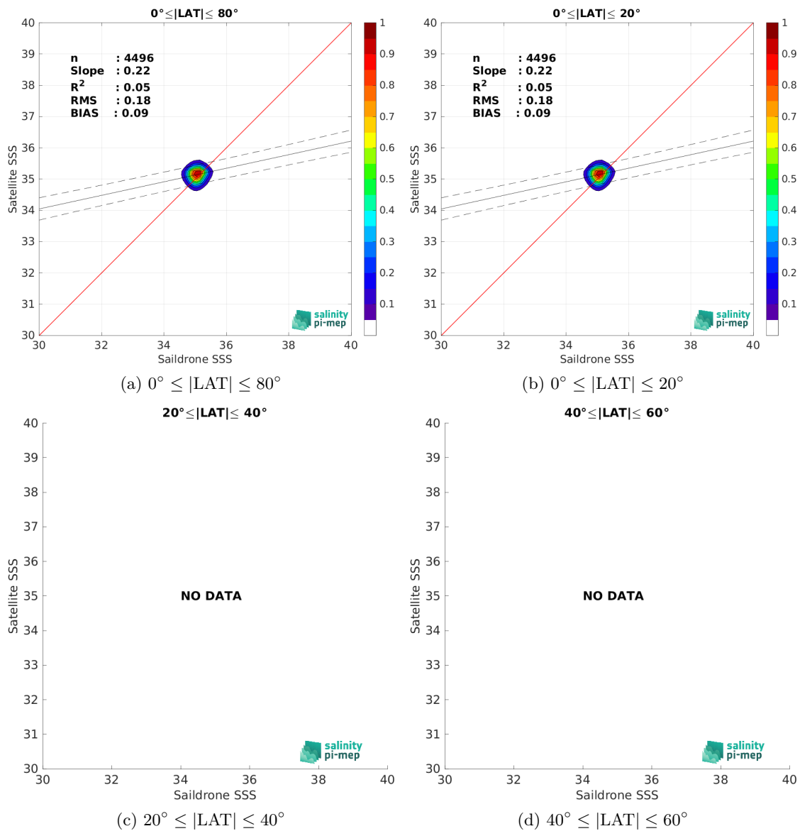
Figure 10: Contour maps of the concentration of CCI SSS L4 Merged-OI v5.5 - 30-day running (ESA) SSS (y-axis) versus Saildrone SSS (x-axis) at match-up pairs for different latitude bands. For each plot, the red line shows x=y . The black thin and dashed lines indicate a linear fit through the data cloud and the \pm 95\% confidence levels, respectively. The number match-up pairs n , the slope and R^2 coefficient of the linear fit, the root mean square (RMS) and the mean bias between satellite and in situ data are indicated for each latitude band in each plots.
