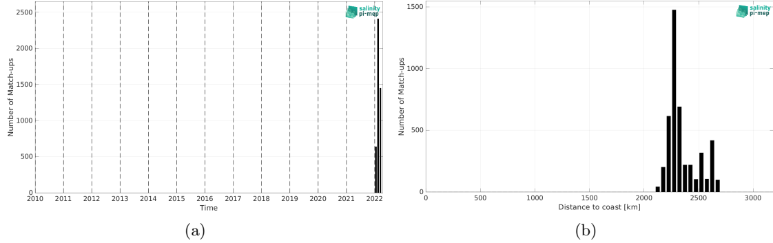
Figure 2: Number of match-ups between Saildrone and CCI SSS L4 Merged-OI v5.5 - 30-day running (ESA) SSS as a function of time (a) and as function of the distance to coast (b) over the OTT zone Pi-MEP region and for the full satellite product period.
