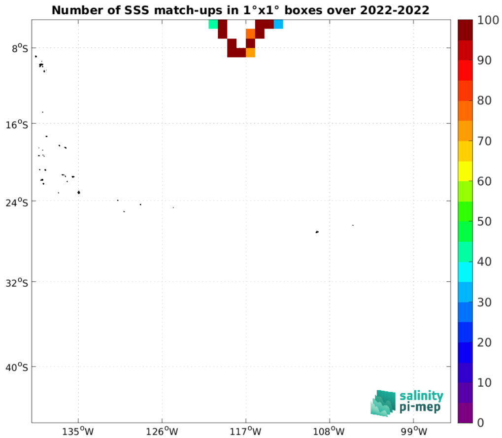
Figure 5: Number of SSS match-ups between Saildrone SSS and the CCI SSS L4 Merged-OI v5.5 - 30-day running (ESA) SSS product for the OTT zone Pi-MEP region over 1°x1° boxes and for the full satellite product period.
