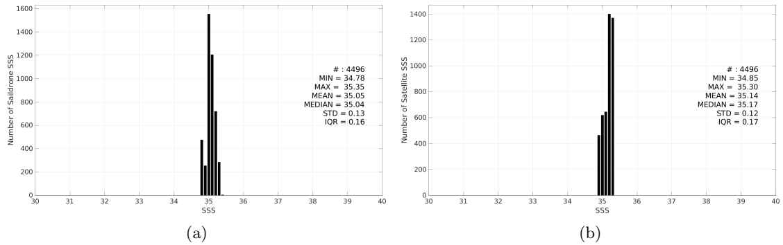
Figure 3: Histograms of SSS from Saildrone (a) and CCI SSS L4 Merged-OI v5.5 - 30-day running (ESA) (b) considering all match-up pairs per bins of 0.1 over the OTT zone Pi-MEP region and for the full satellite product period.
