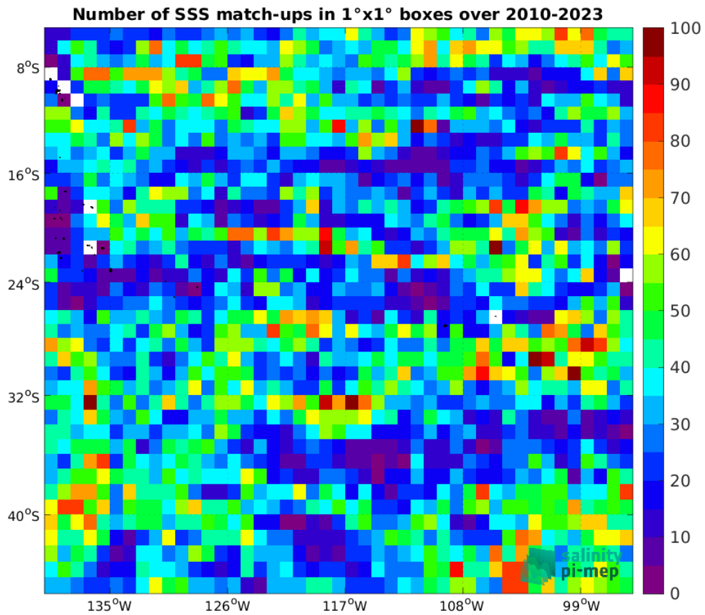
Figure 5: Number of SSS match-ups between Argo SSS and the CCI SSS L4 Merged-OI v5.5 - 30-day running (ESA) SSS product for the OTT zone Pi-MEP region over 1°x1° boxes and for the full satellite product period.
