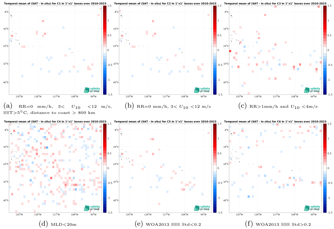
Figure 14: Temporal mean gridded over spatial boxes of size 1^\circ \times 1^\circ of \Delta SSS (CCI SSS L4 Merged-OI v5.5 - 30-day running (ESA) - Argo) for 6 different subdatasets corresponding to:RR=0 mm/h, 3 < U_{10} < 12 m/s, SST >5^\circ C, distance to coast > 800 km (a), RR=0 mm/h, 3 < U_{10} < 12 m/s (b), RR >1 mm/h and U_{10} < 4 m/s (c),MLD <20 m (d),WOA2013 SSS Std <0.2 (e),WOA2013 SSS Std >0.2 (f).
