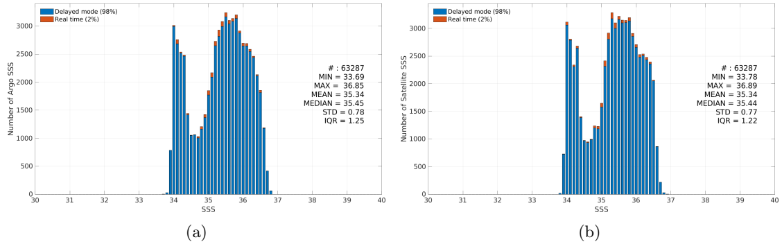
Figure 3: Histograms of SSS from Argo (a) and CCI SSS L4 Merged-OI v5.5 - 30-day running (ESA) (b) considering all match-up pairs per bins of 0.1 over the OTT zone Pi-MEP region and for the full satellite product period.
