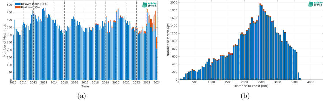
Figure 2: Number of match-ups between Argo and CCI SSS L4 Merged-OI v5.5 - 30-day running (ESA) SSS as a function of time (a) and as function of the distance to coast (b) over the OTT zone Pi-MEP region and for the full satellite product period.
