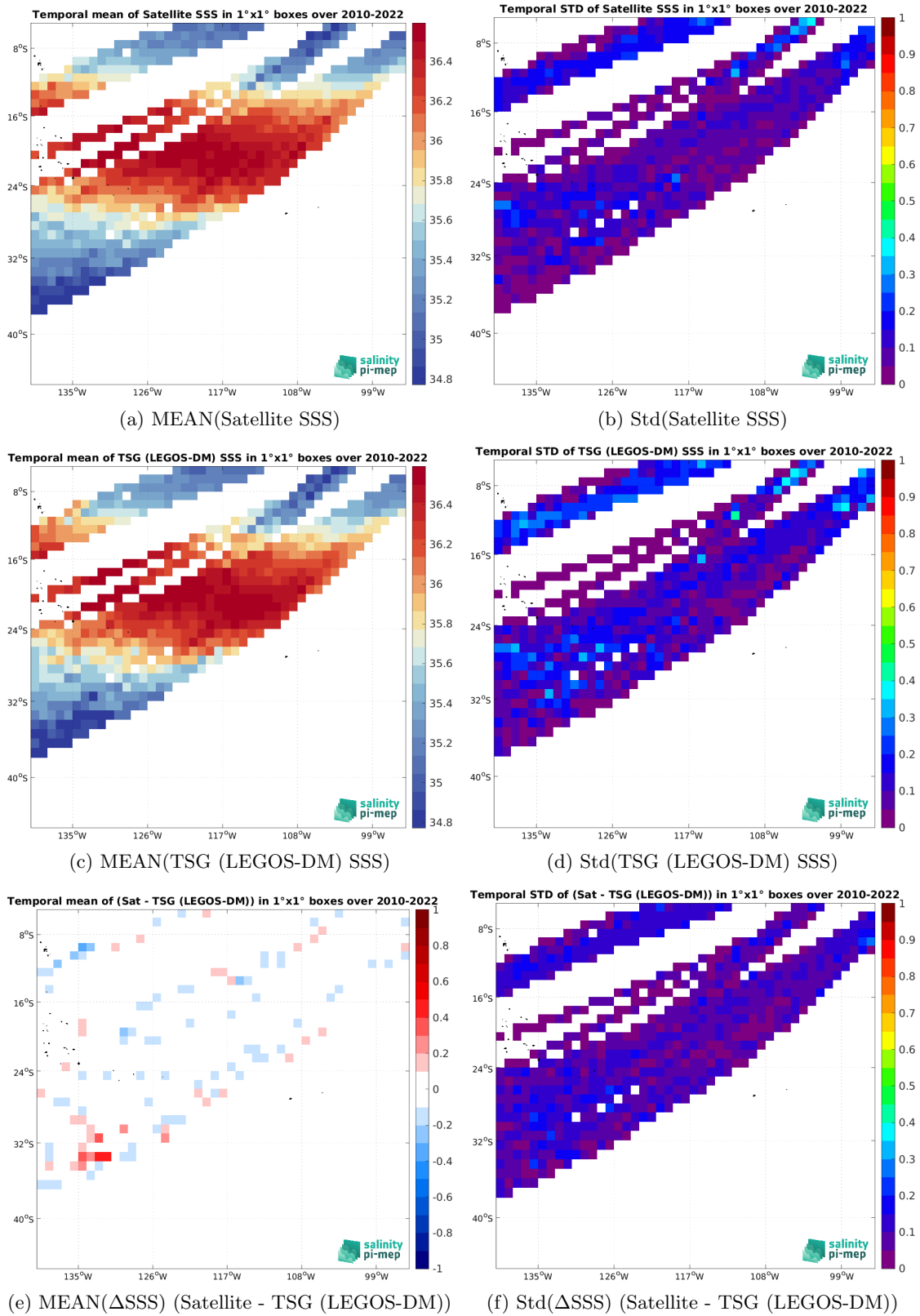
Figure 7: Temporal mean (left) and Std (right) of SSS from CCI SSS L4 Merged-OI v4.41 - 7-day running (ESA) (top), TSG (LEGOS-DM) (middle), and of \Delta SSS (Satellite - TSG (LEGOS-DM)). Only match-up pairs are used to generate these maps.
