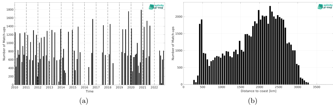
Figure 2: Number of match-ups between TSG (LEGOS-DM) and CCI SSS L4 Merged-OI v4.41 - 7-day running (ESA) SSS as a function of time (a) and as function of the distance to coast (b) over the OTT zone Pi-MEP region and for the full satellite product period.
