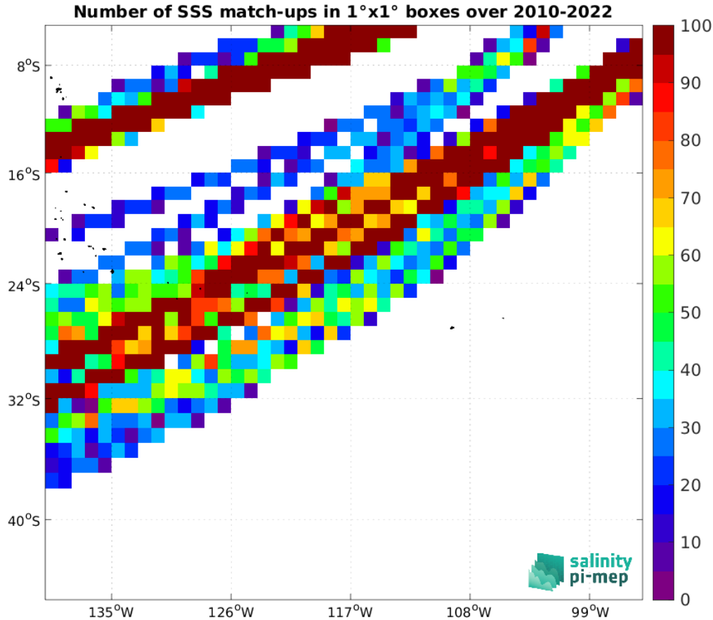
Figure 5: Number of SSS match-ups between TSG (LEGOS-DM) SSS and the CCI SSS L4 Merged-OI v4.41 - 7-day running (ESA) SSS product for the OTT zone Pi-MEP region over 1^\circ \times 1^\circ boxes and for the full satellite product period.
