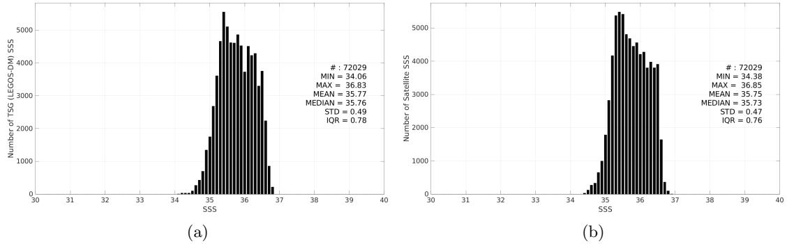
Figure 3: Histograms of SSS from TSG (LEGOS-DM) (a) and CCI SSS L4 Merged-OI v4.41 - 7-day running (ESA) (b) considering all match-up pairs per bins of 0.1 over the OTT zone Pi-MEP region and for the full satellite product period.
