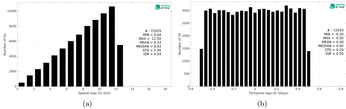
Figure 6: Histograms of the spatial (a) and temporal (b) lags between the location/time of the TSG (LEGOS-DM) measurement and the date of the corresponding CCI SSS L4 Merged-OI v4.41 - 7-day running (ESA) SSS pixel.
