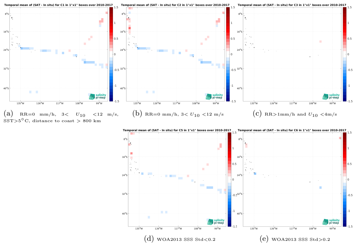
Figure 14: Temporal mean gridded over spatial boxes of size 1^\circ \times 1^\circ of \Delta\text{SSS} (CCI SSS L4 Merged-OI v4.41 - 7-day running (ESA) - TSG (GOSUD-Sailing-ship)) for 5 different subdatasets corresponding to:RR=0 mm/h, 3 < U_{10} < 12 m/s, SST >5^\circ\text{C} , distance to coast > 800 km (a), RR=0 mm/h, 3 < U_{10} < 12 m/s (b), RR >1\text{mm/h} and U_{10} < 4\text{m/s} (c), WOA2013 SSS Std <0.2 (d), WOA2013 SSS Std >0.2 (e).
