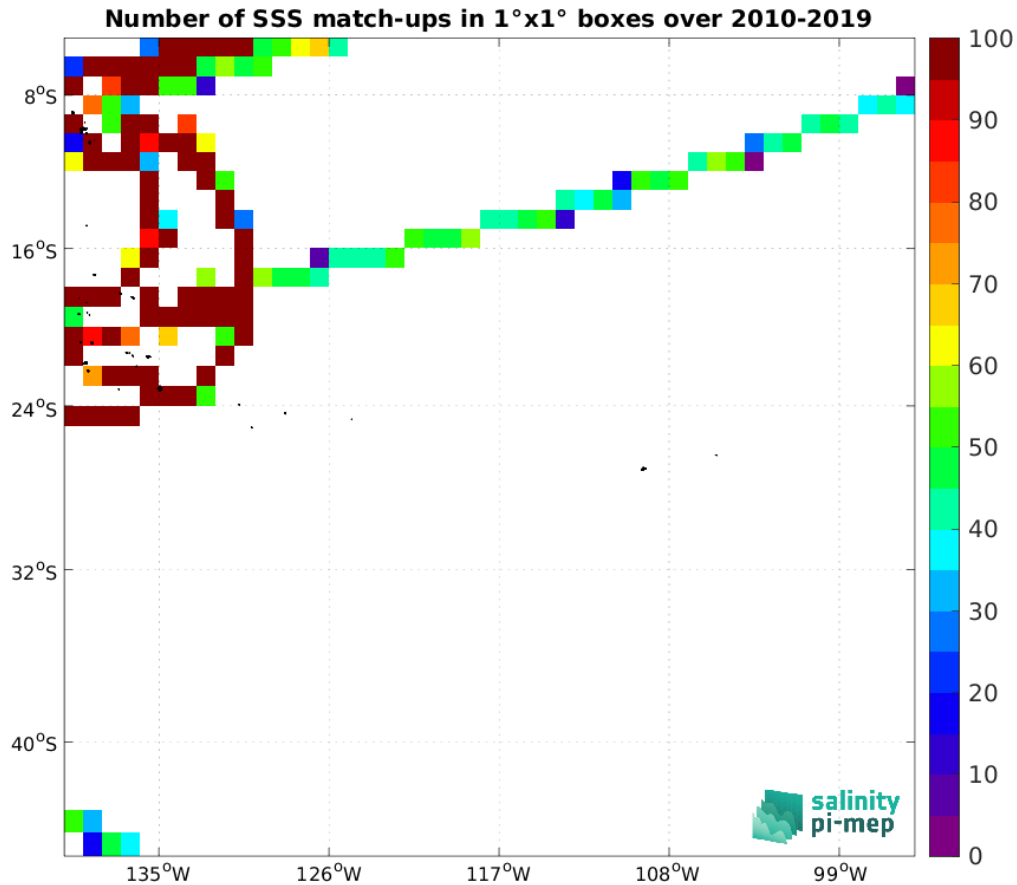
Figure 5: Number of SSS match-ups between TSG (GOSUD-Research-vessel) SSS and the CCI SSS L4 Merged-OI v4.41 - 7-day running (ESA) SSS product for the OTT zone Pi-MEP region over 1^\circ \times 1^\circ boxes and for the full satellite product period.
