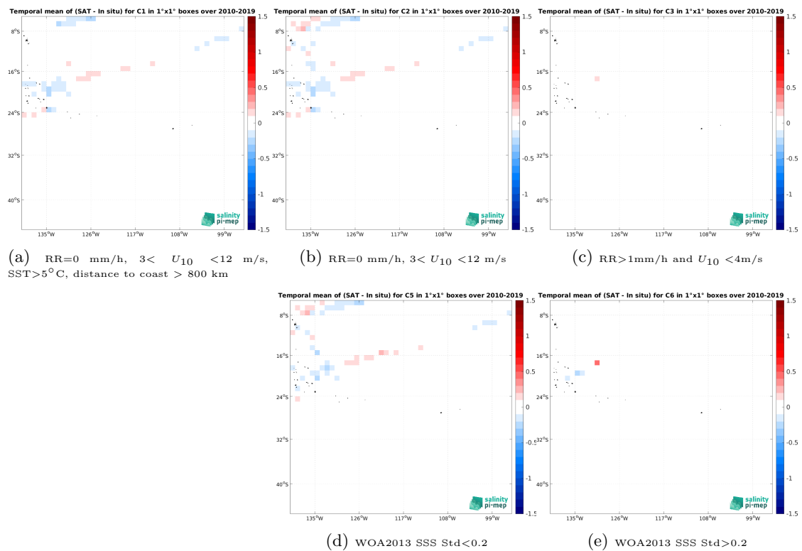
Figure 14: Temporal mean gridded over spatial boxes of size 1^\circ \times 1^\circ of \Delta\text{SSS} (CCI SSS L4 Merged-OI v4.41 - 7-day running (ESA) - TSG (GOSUD-Research-vessel)) for 5 different subdatasets corresponding to:RR=0 mm/h, 3 < U_{10} < 12 m/s, SST >5^\circ\text{C} , distance to coast > 800 km (a), RR=0 mm/h, 3 < U_{10} < 12 m/s (b), RR >1 mm/h and U_{10} < 4 m/s (c), WOA2013 SSS Std <0.2 (d), WOA2013 SSS Std >0.2 (e).
