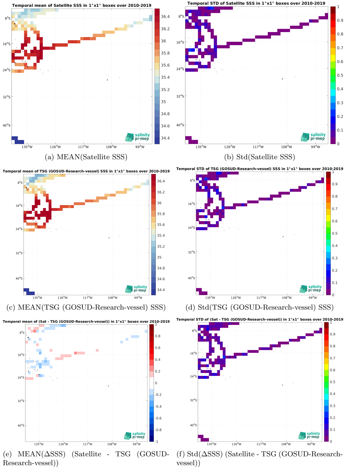
Figure 7: Temporal mean (left) and Std (right) of SSS from CCI SSS L4 Merged-OI v4.41 - 7-day running (ESA) (top), TSG (GOSUD-Research-vessel) (middle), and of \Delta SSS (Satellite - TSG (GOSUD-Research-vessel)). Only match-up pairs are used to generate these maps.
