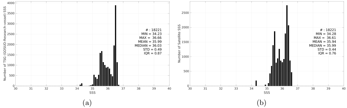
Figure 3: Histograms of SSS from TSG (GOSUD-Research-vessel) (a) and CCI SSS L4 Merged-OI v4.41 - 7-day running (ESA) (b) considering all match-up pairs per bins of 0.1 over the OTT zone Pi-MEP region and for the full satellite product period.
