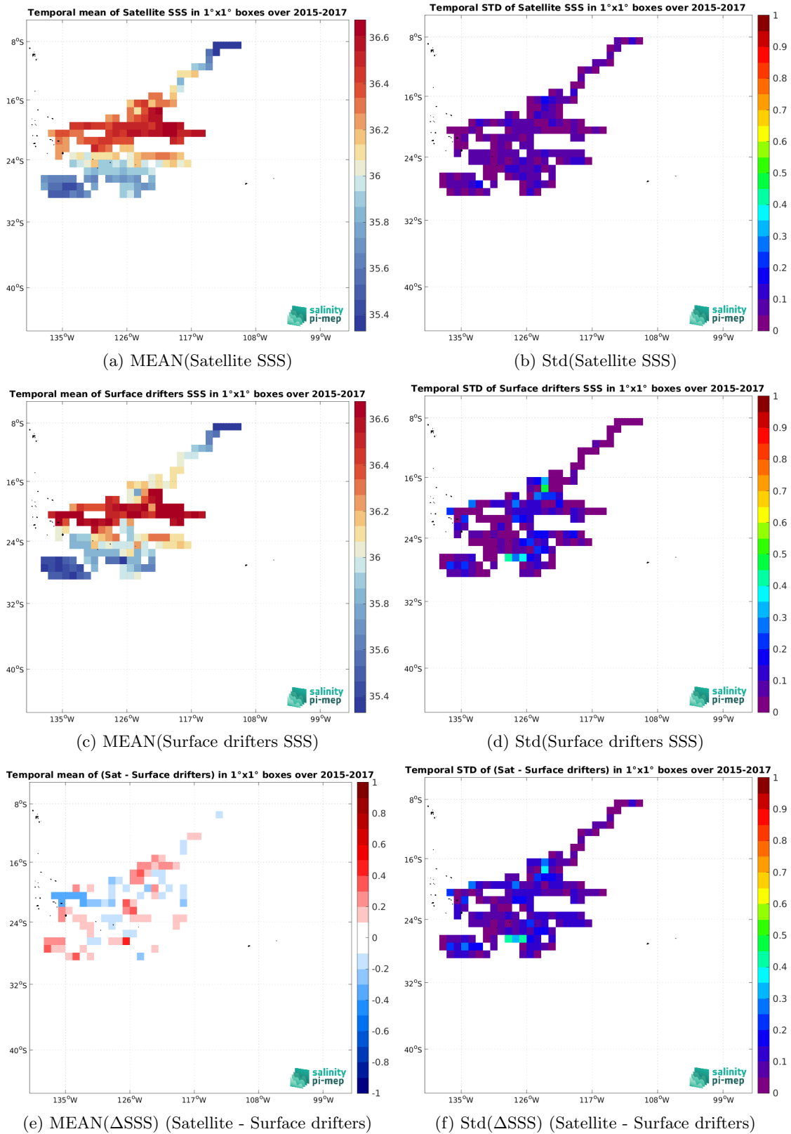
Figure 6: Temporal mean (left) and Std (right) of SSS from CCI SSS L4 Merged-OI v4.41 - 7-day running (ESA) (top), Surface drifters (middle), and of \Delta SSS (Satellite - Surface drifters). Only match-up pairs are used to generate these maps.
