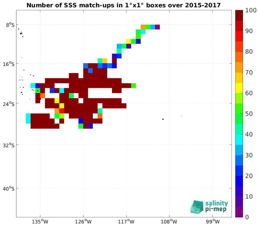
Figure 4: Number of SSS match-ups between Surface drifters SSS and the CCI SSS L4 Merged-OI v4.41 - 7-day running (ESA) SSS product for the OTT zone Pi-MEP region over 1°x1° boxes and for the full satellite product period.
