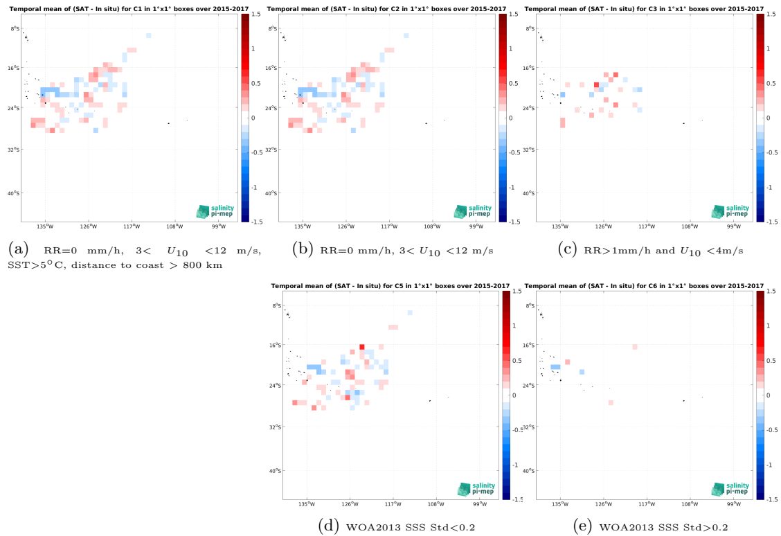
Figure 13: Temporal mean gridded over spatial boxes of size 1^\circ \times 1^\circ of \Delta\text{SSS} (CCI SSS L4 Merged-OI v4.41 - 7-day running (ESA) - Surface drifters) for 5 different subdatasets corresponding to:RR=0 mm/h, 3 < U_{10} < 12 m/s, SST >5^\circ\text{C} , distance to coast > 800 km (a), RR=0 mm/h, 3 < U_{10} < 12 m/s (b), RR >1 mm/h and U_{10} < 4 m/s (c), WOA2013 SSS Std <0.2 (d), WOA2013 SSS Std >0.2 (e).
