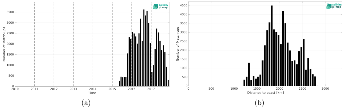
Figure 2: Number of match-ups between Surface drifters and CCI SSS L4 Merged-OI v4.41 - 7-day running (ESA) SSS as a function of time (a) and as function of the distance to coast (b) over the OTT zone Pi-MEP region and for the full satellite product period.
