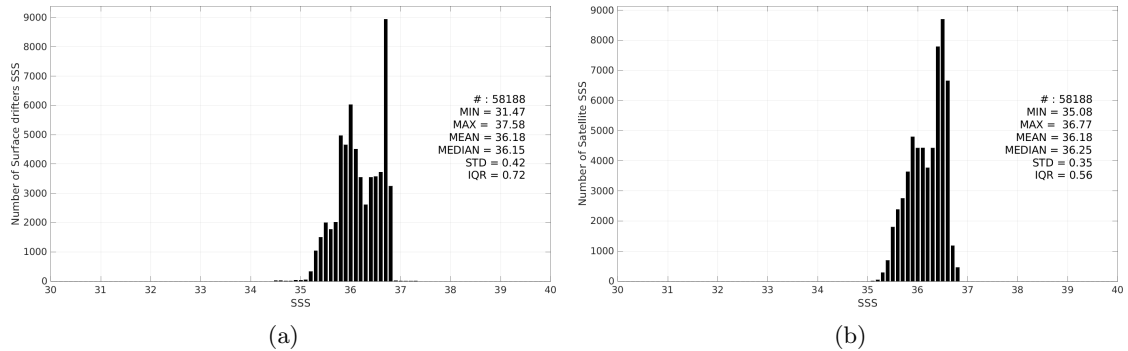
Figure 3: Histograms of SSS from Surface drifters (a) and CCI SSS L4 Merged-OI v4.41 - 7-day running (ESA) (b) considering all match-up pairs per bins of 0.1 over the OTT zone Pi-MEP region and for the full satellite product period.
