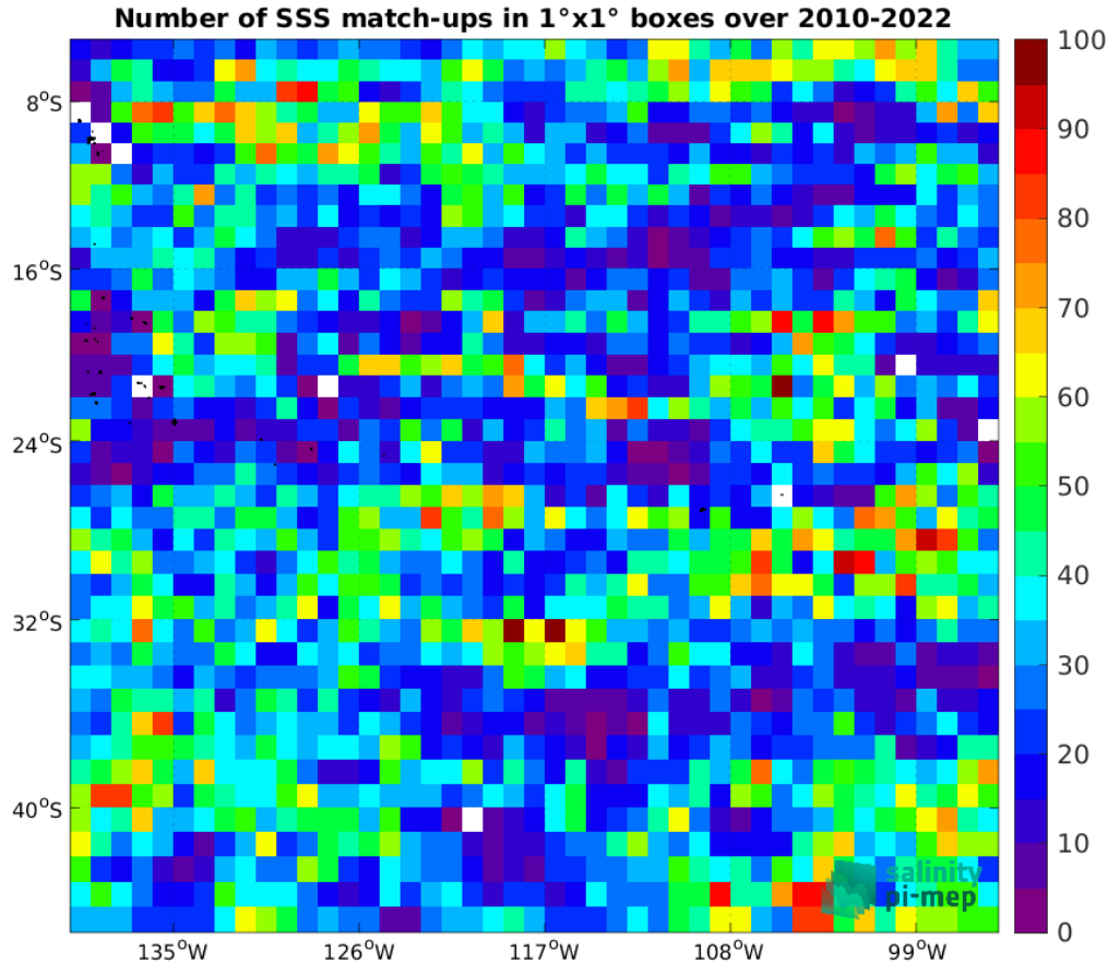
Figure 5: Number of SSS match-ups between Argo SSS and the CCI SSS L4 Merged-OI v4.41 - 7-day running (ESA) SSS product for the OTT zone Pi-MEP region over 1^\circ \times 1^\circ boxes and for the full satellite product period.
