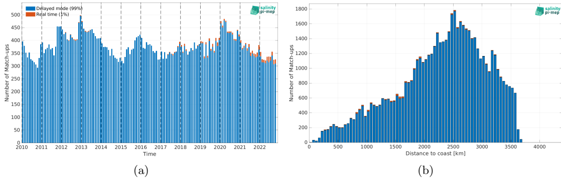
Figure 2: Number of match-ups between Argo and CCI SSS L4 Merged-OI v4.41 - 7-day running (ESA) SSS as a function of time (a) and as function of the distance to coast (b) over the OTT zone Pi-MEP region and for the full satellite product period.
