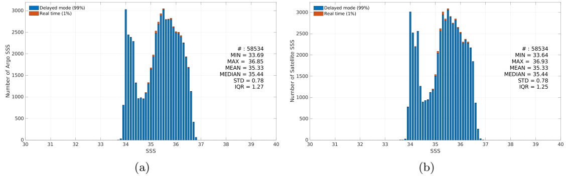
Figure 3: Histograms of SSS from Argo (a) and CCI SSS L4 Merged-OI v4.41 - 7-day running (ESA) (b) considering all match-up pairs per bins of 0.1 over the OTT zone Pi-MEP region and for the full satellite product period.
