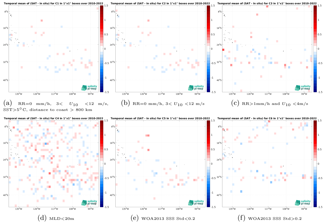
Figure 14: Temporal mean gridded over spatial boxes of size 1^\circ \times 1^\circ of \Delta SSS (CCI SSS L4 Merged-OI v4.41 - 7-day running (ESA) - Argo) for 6 different subdatasets corresponding to:RR=0 mm/h, 3 < U_{10} < 12 m/s, SST > 5^\circ\text{C} , distance to coast > 800 km (a), RR=0 mm/h, 3 < U_{10} < 12 m/s (b), RR > 1 mm/h and U_{10} < 4 m/s (c),MLD < 20 m (d),WOA2013 SSS Std < 0.2 (e),WOA2013 SSS Std > 0.2 (f).
