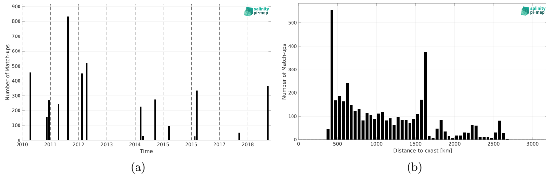
Figure 2: Number of match-ups between TSG (SAMOS) and CCI SSS L4 Merged-OI v4.41 - 30-day running (ESA) SSS as a function of time (a) and as function of the distance to coast (b) over the OTT zone Pi-MEP region and for the full satellite product period.
