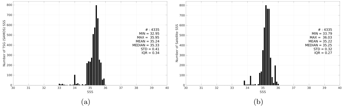
Figure 3: Histograms of SSS from TSG (SAMOS) (a) and CCI SSS L4 Merged-OI v4.41 - 30-day running (ESA) (b) considering all match-up pairs per bins of 0.1 over the OTT zone Pi-MEP region and for the full satellite product period.
