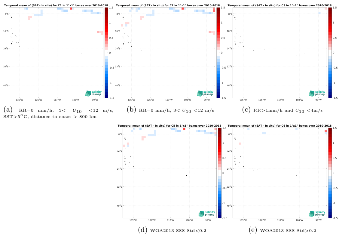
Figure 14: Temporal mean gridded over spatial boxes of size 1^\circ \times 1^\circ of \Delta SSS (CCI SSS L4 Merged-OI v4.41 - 30-day running (ESA) - TSG (SAMOS)) for 5 different subdatasets corresponding to:RR=0 mm/h, 3 < U_{10} < 12 m/s, SST >5^\circ C, distance to coast > 800 km (a), RR=0 mm/h, 3 < U_{10} < 12 m/s (b), RR >1 mm/h and U_{10} < 4 m/s (c), WOA2013 SSS Std <0.2 (d), WOA2013 SSS Std >0.2 (e).
