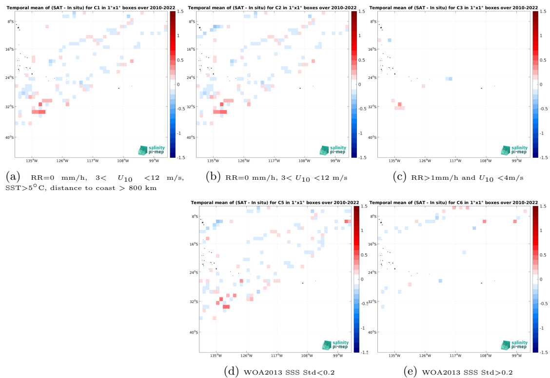
Figure 14: Temporal mean gridded over spatial boxes of size 1^\circ \times 1^\circ of \Delta SSS (CCI SSS L4 Merged-OI v4.41 - 30-day running (ESA) - TSG (LEGOS-DM)) for 5 different subdatasets corresponding to: RR=0 mm/h, 3 < U_{10} < 12 m/s, SST > 5^\circ\text{C} , distance to coast > 800 km (a), RR=0 mm/h, 3 < U_{10} < 12 m/s (b), RR > 1 mm/h and U_{10} < 4 m/s (c), WOA2013 SSS Std < 0.2 (d), WOA2013 SSS Std > 0.2 (e).
