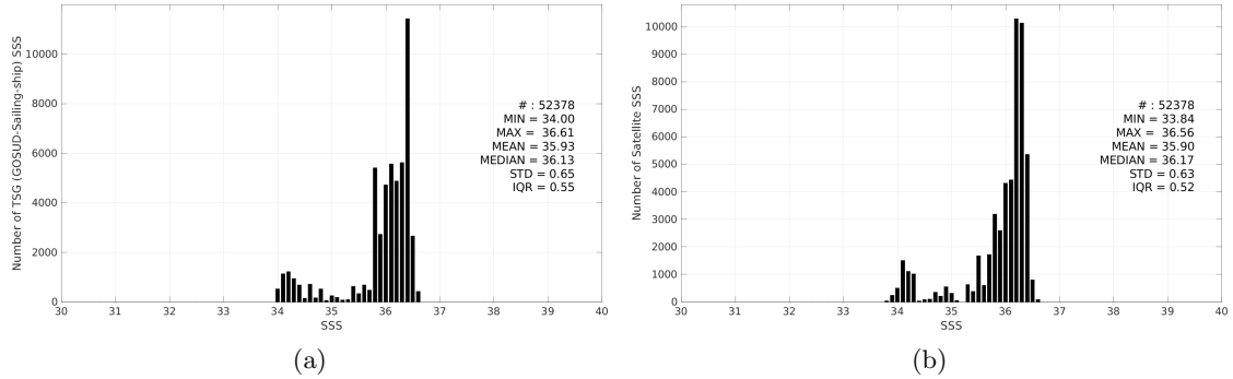
Figure 3: Histograms of SSS from TSG (GOSUD-Sailing-ship) (a) and CCI SSS L4 Merged-OI v4.41 - 30-day running (ESA) (b) considering all match-up pairs per bins of 0.1 over the OTT zone Pi-MEP region and for the full satellite product period.
