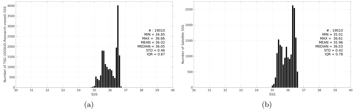
Figure 3: Histograms of SSS from TSG (GOSUD-Research-vessel) (a) and CCI SSS L4 Merged-OI v4.41 - 30-day running (ESA) (b) considering all match-up pairs per bins of 0.1 over the OTT zone Pi-MEP region and for the full satellite product period.
