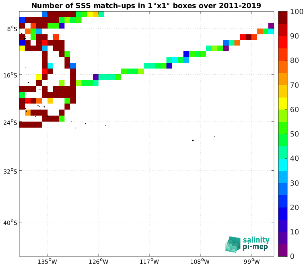
Figure 5: Number of SSS match-ups between TSG (GOSUD-Research-vessel) SSS and the CCI SSS L4 Merged-OI v4.41 - 30-day running (ESA) SSS product for the OTT zone Pi-MEP region over 1^\circ \times 1^\circ boxes and for the full satellite product period.
