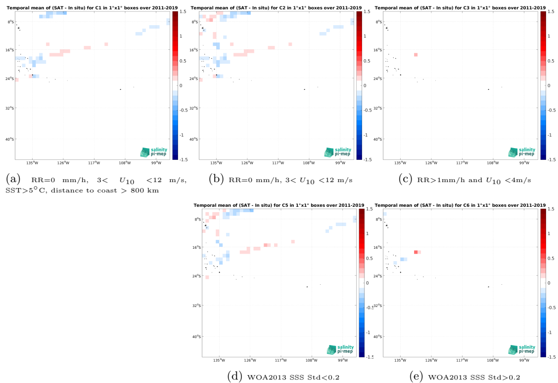
Figure 14: Temporal mean gridded over spatial boxes of size 1^\circ \times 1^\circ of \Delta SSS (CCI SSS L4 Merged-OI v4.41 - 30-day running (ESA) - TSG (GOSUD-Research-vessel)) for 5 different subdatasets corresponding to:RR=0 mm/h, 3 < U_{10} < 12 m/s, SST >5^\circ\text{C} , distance to coast > 800 km (a), RR=0 mm/h, 3 < U_{10} < 12 m/s (b), RR >1 mm/h and U_{10} < 4 m/s (c), WOA2013 SSS Std <0.2 (d), WOA2013 SSS Std >0.2 (e).
