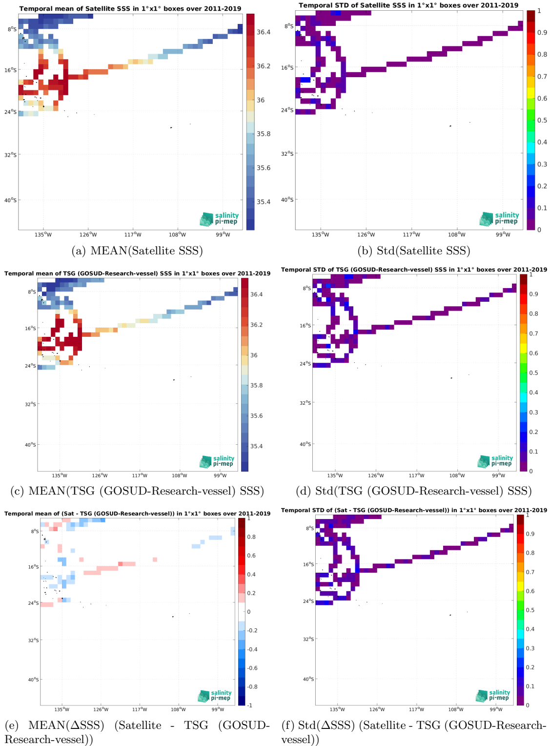
Figure 7: Temporal mean (left) and Std (right) of SSS from CCI SSS L4 Merged-OI v4.41 - 30-day running (ESA) (top), TSG (GOSUD-Research-vessel) (middle), and of \Delta SSS (Satellite - TSG (GOSUD-Research-vessel)). Only match-up pairs are used to generate these maps.
