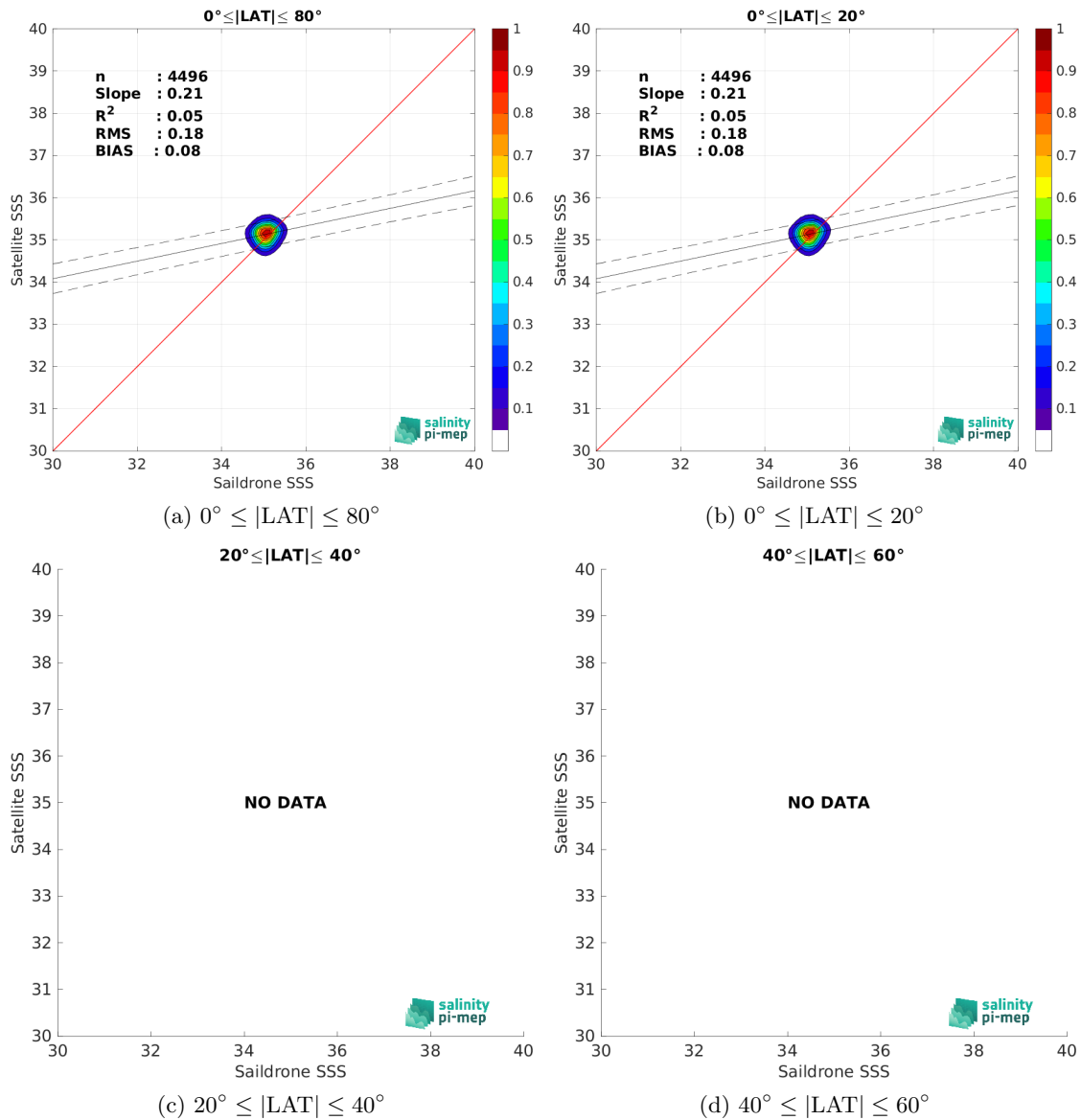
Figure 10: Contour maps of the concentration of CCI SSS L4 Merged-OI v4.41 - 30-day running (ESA) SSS (y-axis) versus Saildrone SSS (x-axis) at match-up pairs for different latitude bands. For each plot, the red line shows x=y . The black thin and dashed lines indicate a linear fit through the data cloud and the \pm 95\% confidence levels, respectively. The number match-up pairs n , the slope and R^2 coefficient of the linear fit, the root mean square (RMS) and the mean bias between satellite and in situ data are indicated for each latitude band in each plots.
