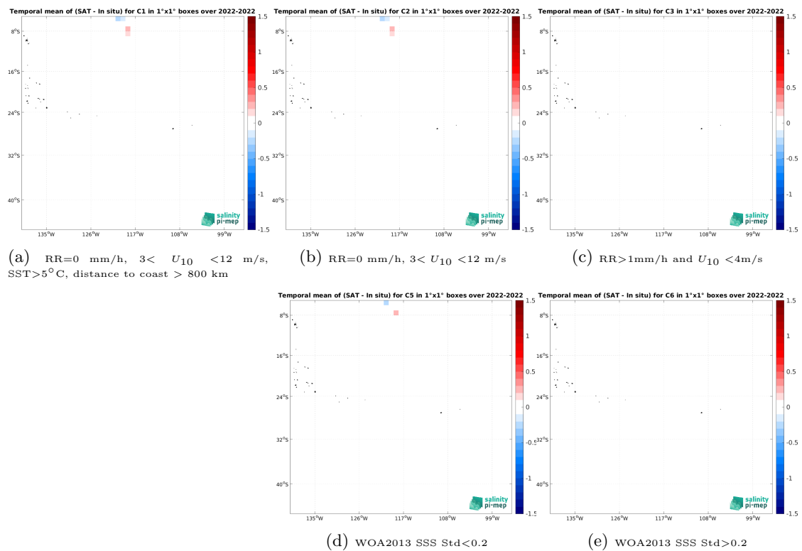
Figure 14: Temporal mean gridded over spatial boxes of size 1^\circ \times 1^\circ of \Delta SSS (CCI SSS L4 Merged-OI v4.41 - 30-day running (ESA) - Saildrone) for 5 different subdatasets corresponding to: RR=0 mm/h, 3 < U_{10} < 12 m/s, SST > 5^\circ C , distance to coast > 800 km (a), RR=0 mm/h, 3 < U_{10} < 12 m/s (b), RR > 1 mm/h and U_{10} < 4 m/s (c), WOA2013 SSS Std < 0.2 (d), WOA2013 SSS Std > 0.2 (e).
