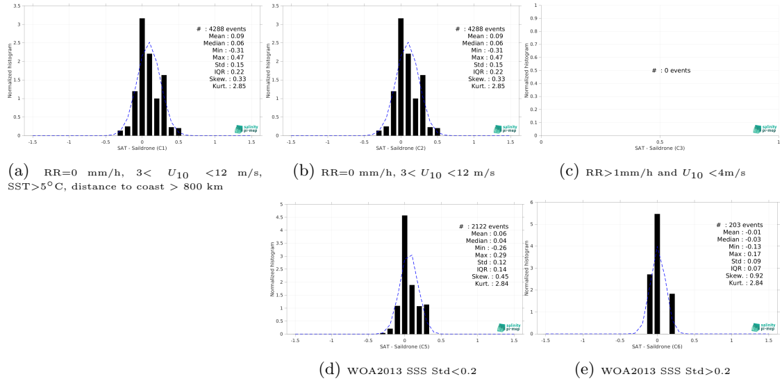
Figure 15: Normalized histogram of \Delta SSS (CCI SSS L4 Merged-OI v4.41 - 30-day running (ESA) - Saildrone) for 5 different subdatasets corresponding to: RR=0 mm/h, 3 < U_{10} < 12 m/s, SST > 5°C, distance to coast > 800 km (a), RR=0 mm/h, 3 < U_{10} < 12 m/s (b), RR > 1mm/h and U_{10} < 4 m/s (c), WOA2013 SSS Std < 0.2 (d), WOA2013 SSS Std > 0.2 (e).
