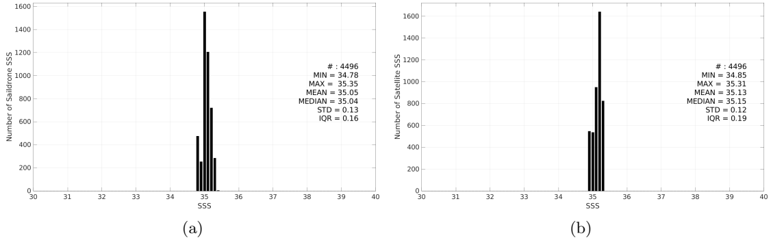
Figure 3: Histograms of SSS from Saildrone (a) and CCI SSS L4 Merged-OI v4.41 - 30-day running (ESA) (b) considering all match-up pairs per bins of 0.1 over the OTT zone Pi-MEP region and for the full satellite product period.
