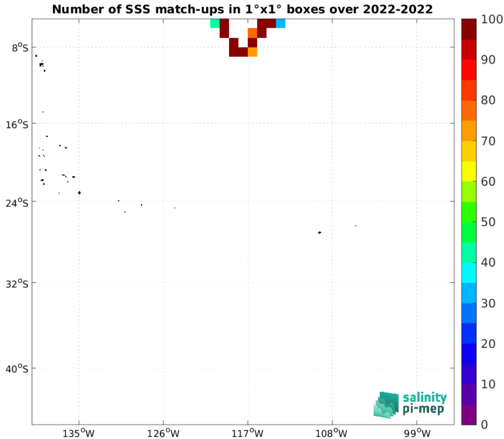
Figure 5: Number of SSS match-ups between Saildrone SSS and the CCI SSS L4 Merged-OI v4.41 - 30-day running (ESA) SSS product for the OTT zone Pi-MEP region over 1^\circ \times 1^\circ boxes and for the full satellite product period.
