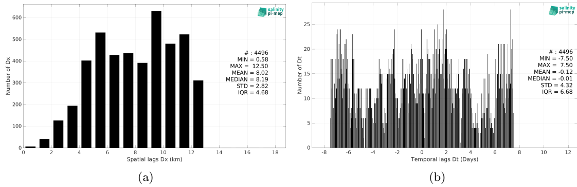
Figure 6: Histograms of the spatial (a) and temporal (b) lags between the location/time of the Saildrone measurement and the date of the corresponding CCI SSS L4 Merged-OI v4.41 - 30-day running (ESA) SSS pixel.
