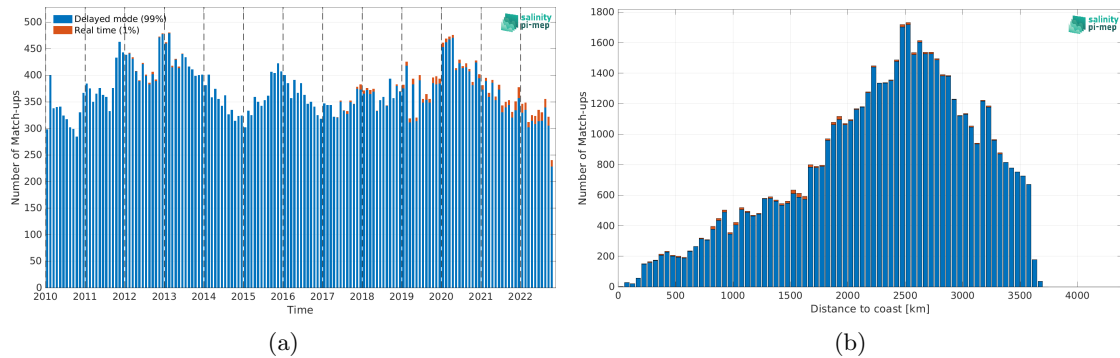
Figure 2: Number of match-ups between Argo and CCI SSS L4 Merged-OI v4.41 - 30-day running (ESA) SSS as a function of time (a) and as function of the distance to coast (b) over the OTT zone Pi-MEP region and for the full satellite product period.
