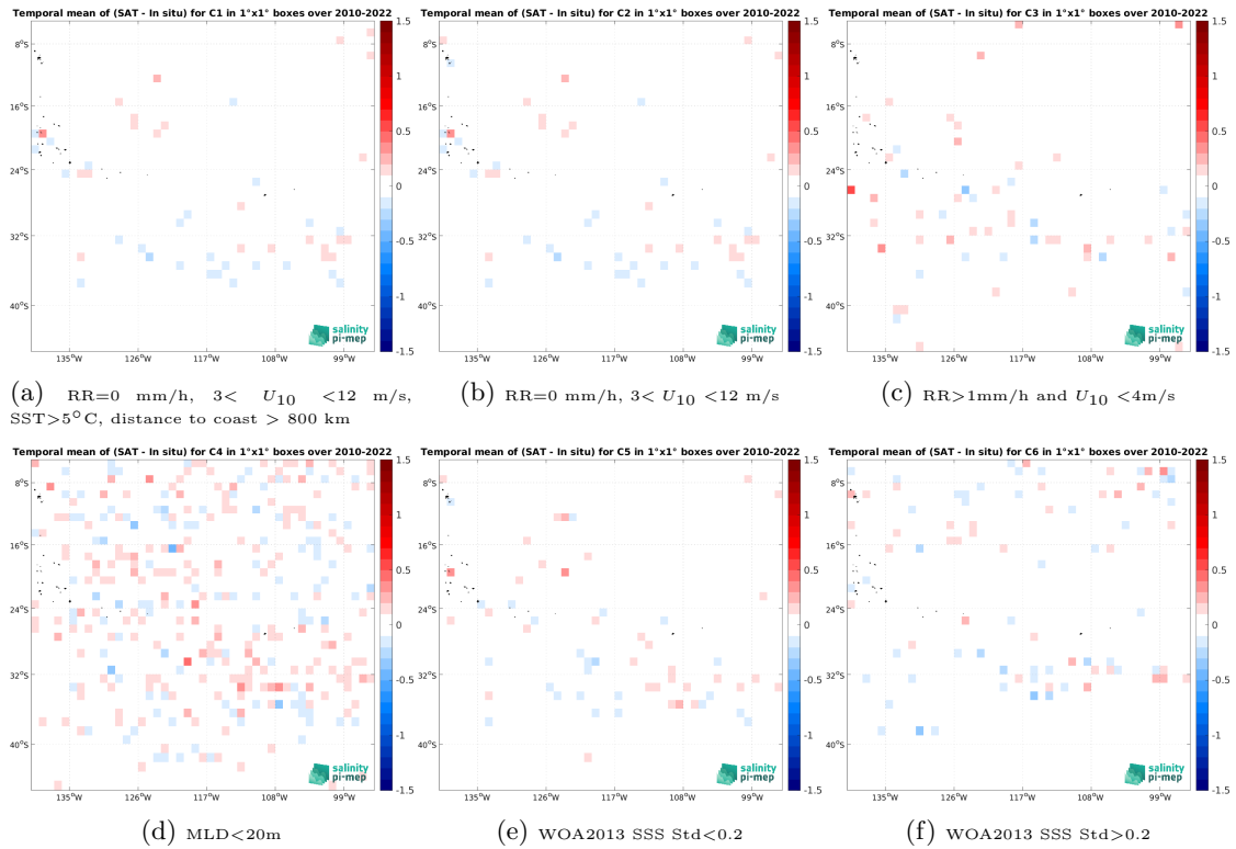
Figure 14: Temporal mean gridded over spatial boxes of size 1^\circ \times 1^\circ of \Delta SSS (CCI SSS L4 Merged-OI v4.41 - 30-day running (ESA) - Argo) for 6 different subdatasets corresponding to:RR=0 mm/h, 3 < U_{10} < 12 m/s, SST >5^\circ C, distance to coast > 800 km (a), RR=0 mm/h, 3 < U_{10} < 12 m/s (b), RR >1 mm/h and U_{10} < 4 m/s (c),MLD <20 m (d),WOA2013 SSS Std <0.2 (e),WOA2013 SSS Std >0.2 (f).
