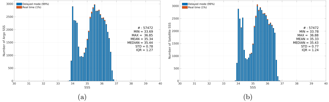
Figure 3: Histograms of SSS from Argo (a) and CCI SSS L4 Merged-OI v4.41 - 30-day running (ESA) (b) considering all match-up pairs per bins of 0.1 over the OTT zone Pi-MEP region and for the full satellite product period.
