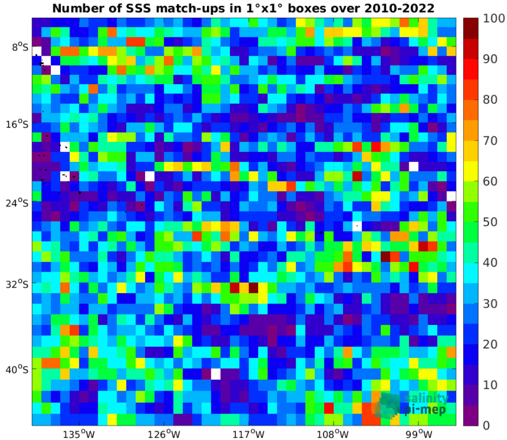
Figure 5: Number of SSS match-ups between Argo SSS and the CCI SSS L4 Merged-OI v4.41 - 30-day running (ESA) SSS product for the OTT zone Pi-MEP region over 1^\circ \times 1^\circ boxes and for the full satellite product period.
