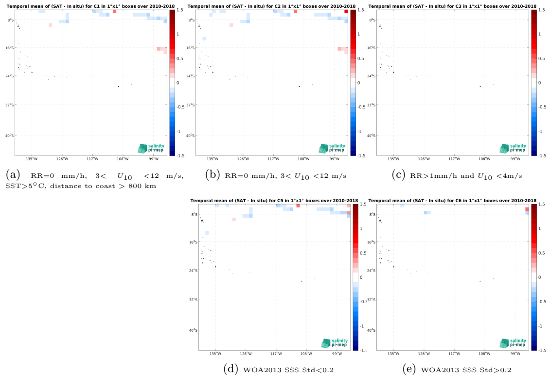
Figure 12: Temporal mean gridded over spatial boxes of size 1^\circ \times 1^\circ of \Delta SSS (CCI SSS L4 Merged-OI v4.4 - 7-day running (ESA) - TSG (SAMOS)) for 5 different subdatasets corresponding to:RR=0 mm/h, 3 < U_{10} < 12 m/s, SST >5^\circ C, distance to coast > 800 km (a), RR=0 mm/h, 3 < U_{10} < 12 m/s (b), RR >1 mm/h and U_{10} < 4 m/s (c), WOA2013 SSS Std <0.2 (d), WOA2013 SSS Std >0.2 (e).
