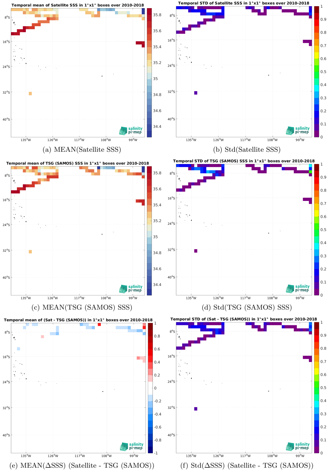
Figure 6: Temporal mean (left) and Std (right) of SSS from CCI SSS L4 Merged-OI v4.4 - 7-day running (ESA) (top), TSG (SAMOS) (middle), and of \Delta SSS (Satellite - TSG (SAMOS)). Only match-up pairs are used to generate these maps.
