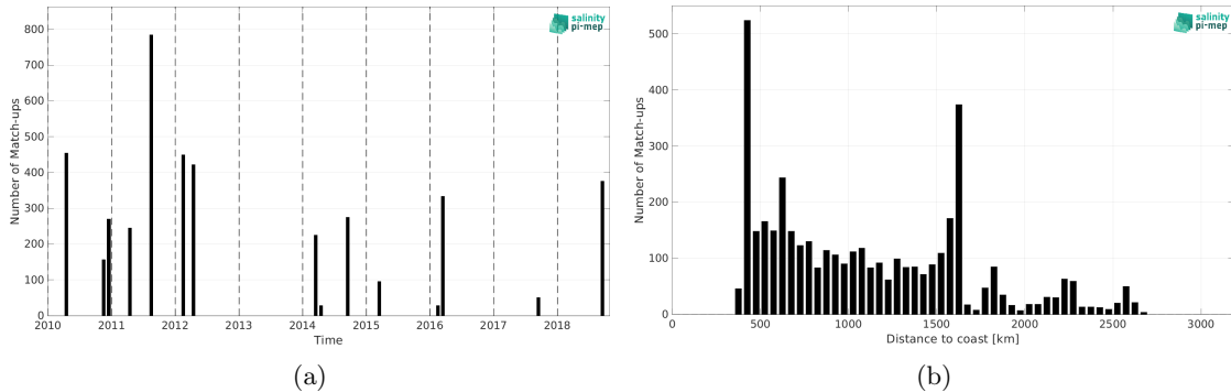
Figure 1: Number of match-ups between TSG (SAMOS) and CCI SSS L4 Merged-OI v4.4 - 7-day running (ESA) SSS as a function of time (a) and as function of the distance to coast (b) over the OTT zone Pi-MEP region and for the full satellite product period.
