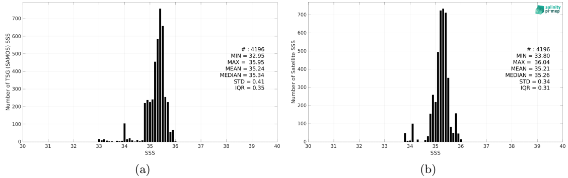
Figure 2: Histograms of SSS from TSG (SAMOS) (a) and CCI SSS L4 Merged-OI v4.4 - 7-day running (ESA) (b) considering all match-up pairs per bins of 0.1 over the OTT zone Pi-MEP region and for the full satellite product period.
