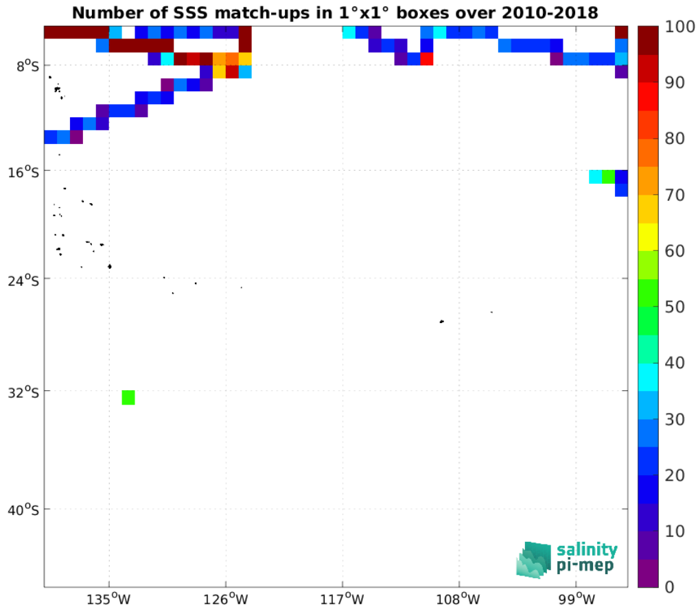
Figure 4: Number of SSS match-ups between TSG (SAMOS) SSS and the CCI SSS L4 Merged-OI v4.4 - 7-day running (ESA) SSS product for the OTT zone Pi-MEP region over 1^\circ \times 1^\circ boxes and for the full satellite product period.
