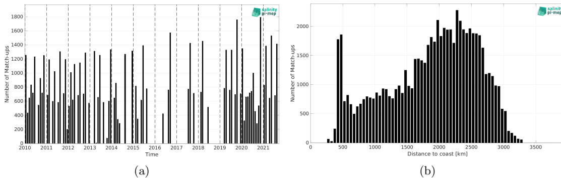
Figure 1: Number of match-ups between TSG (LEGOS-DM) and CCI SSS L4 Merged-OI v4.4 - 7-day running (ESA) SSS as a function of time (a) and as function of the distance to coast (b) over the OTT zone Pi-MEP region and for the full satellite product period.
