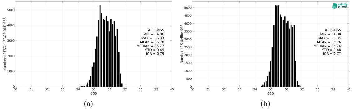
Figure 2: Histograms of SSS from TSG (LEGOS-DM) (a) and CCI SSS L4 Merged-OI v4.4 - 7-day running (ESA) (b) considering all match-up pairs per bins of 0.1 over the OTT zone Pi-MEP region and for the full satellite product period.
