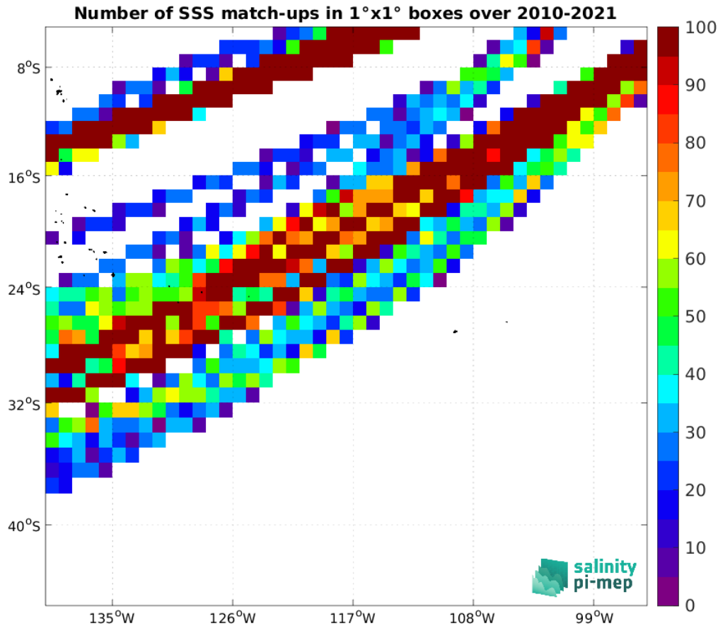
Figure 4: Number of SSS match-ups between TSG (LEGOS-DM) SSS and the CCI SSS L4 Merged-OI v4.4 - 7-day running (ESA) SSS product for the OTT zone Pi-MEP region over 1^\circ \times 1^\circ boxes and for the full satellite product period.
