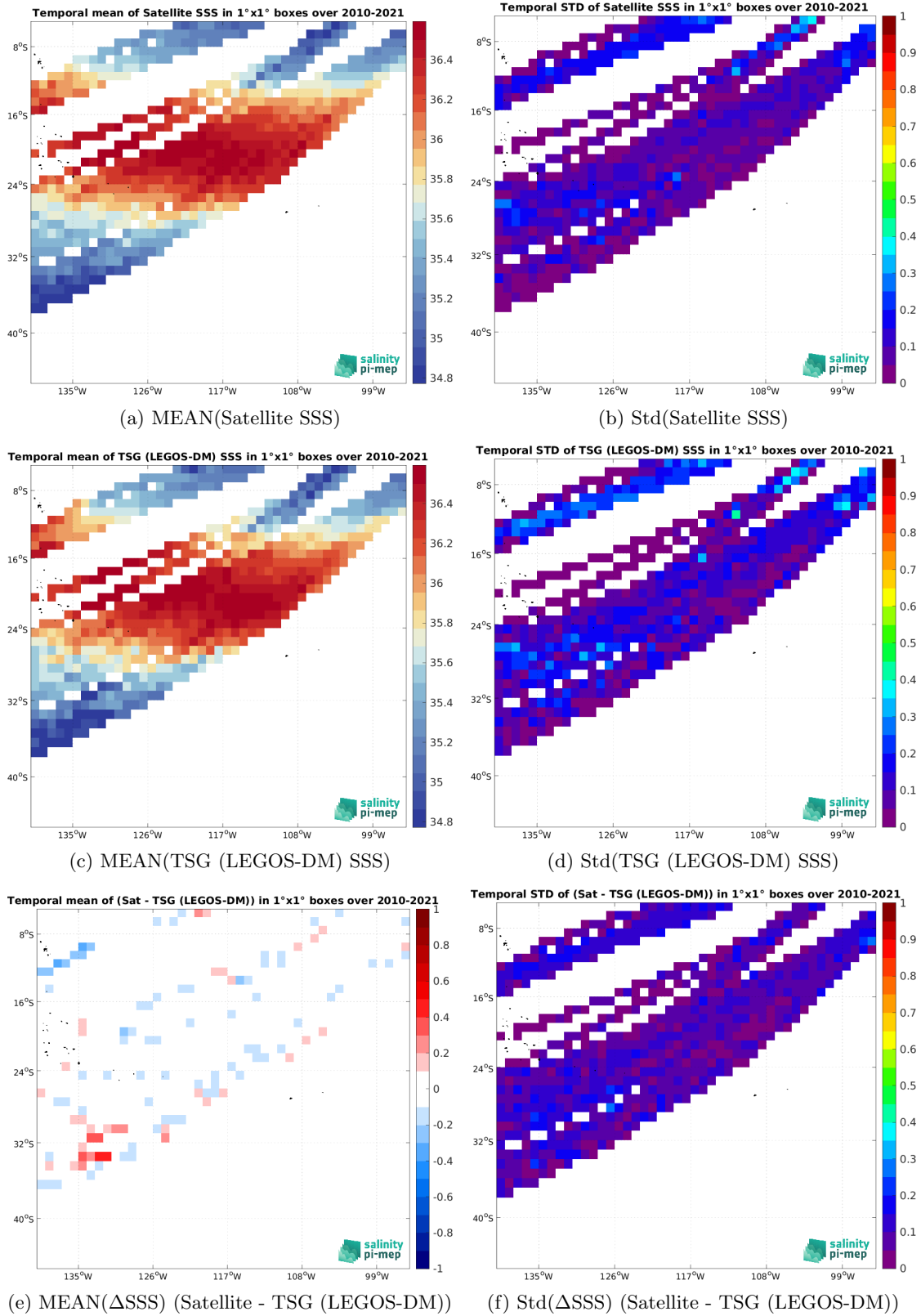
Figure 6: Temporal mean (left) and Std (right) of SSS from CCI SSS L4 Merged-OI v4.4 - 7-day running (ESA) (top), TSG (LEGOS-DM) (middle), and of \Delta SSS (Satellite - TSG (LEGOS-DM)). Only match-up pairs are used to generate these maps.
