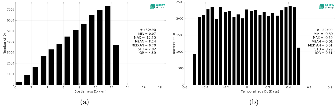
Figure 5: Histograms of the spatial (a) and temporal (b) lags between the location/time of the TSG (GOSUD-Sailing-ship) measurement and the date of the corresponding CCI SSS L4 Merged-OI v4.4 - 7-day running (ESA) SSS pixel.
