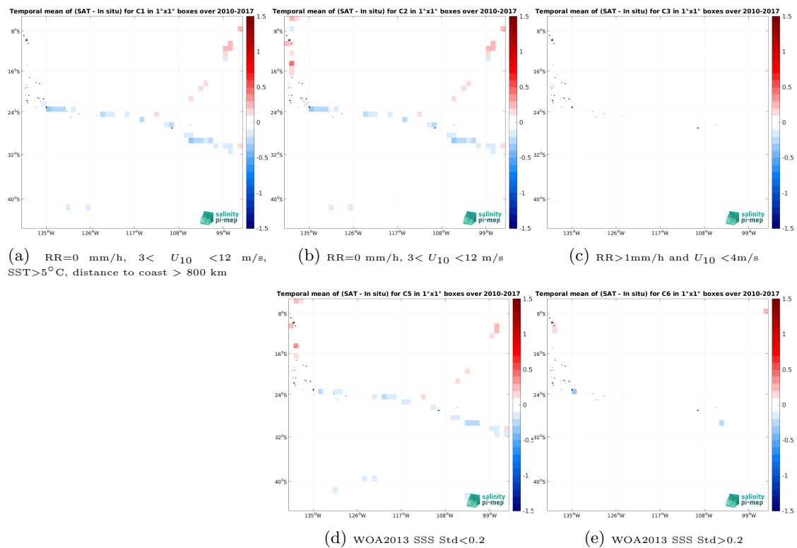
Figure 12: Temporal mean gridded over spatial boxes of size 1^\circ \times 1^\circ of \Delta SSS (CCI SSS L4 Merged-OI v4.4 - 7-day running (ESA) - TSG (GOSUD-Sailing-ship)) for 5 different subdatasets corresponding to:RR=0 mm/h, 3 < U_{10} < 12 m/s, SST >5^\circ C, distance to coast > 800 km (a), RR=0 mm/h, 3 < U_{10} < 12 m/s (b), RR >1 mm/h and U_{10} < 4 m/s (c), WOA2013 SSS Std <0.2 (d), WOA2013 SSS Std >0.2 (e).
