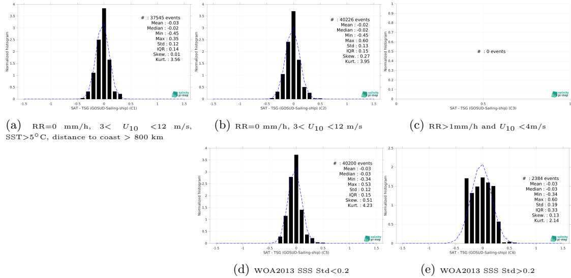
Figure 13: Normalized histogram of \Delta SSS (CCI SSS L4 Merged-OI v4.4 - 7-day running (ESA) - TSG (GOSUD-Sailing-ship)) for 5 different subdatasets corresponding to: RR=0 mm/h, 3 < U_{10} < 12 m/s, SST > 5°C, distance to coast > 800 km (a), RR=0 mm/h, 3 < U_{10} < 12 m/s (b), RR > 1mm/h and U_{10} < 4 m/s (c), WOA2013 SSS Std < 0.2 (d), WOA2013 SSS Std > 0.2 (e).
