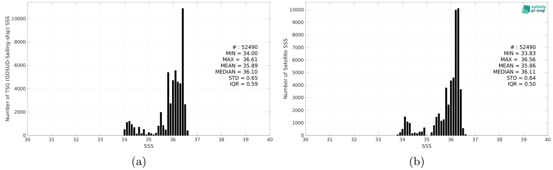
Figure 2: Histograms of SSS from TSG (GOSUD-Sailing-ship) (a) and CCI SSS L4 Merged-OI v4.4 - 7-day running (ESA) (b) considering all match-up pairs per bins of 0.1 over the OTT zone Pi-MEP region and for the full satellite product period.
