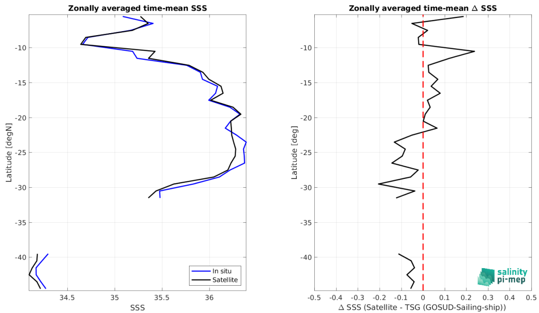
Figure 8: Left panel: Zonal mean SSS from CCI SSS L4 Merged-OI v4.4 - 7-day running (ESA) satellite product (black) and from TSG (GOSUD-Sailing-ship) (blue). Right panel: Zonal mean of \Delta SSS (Satellite - TSG (GOSUD-Sailing-ship)) for all the collected Pi-MEP match-up pairs estimated over the full satellite product period.
