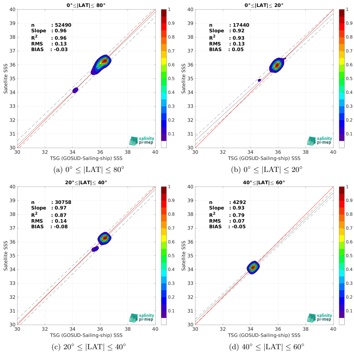
Figure 9: Contour maps of the concentration of CCI SSS L4 Merged-OI v4.4 - 7-day running (ESA) SSS (y-axis) versus TSG (GOSUD-Sailing-ship) SSS (x-axis) at match-up pairs for different latitude bands. For each plot, the red line shows x=y . The black thin and dashed lines indicate a linear fit through the data cloud and the \pm 95\% confidence levels, respectively. The number match-up pairs n , the slope and R^2 coefficient of the linear fit, the root mean square (RMS) and the mean bias between satellite and in situ data are indicated for each latitude band in each plots.
