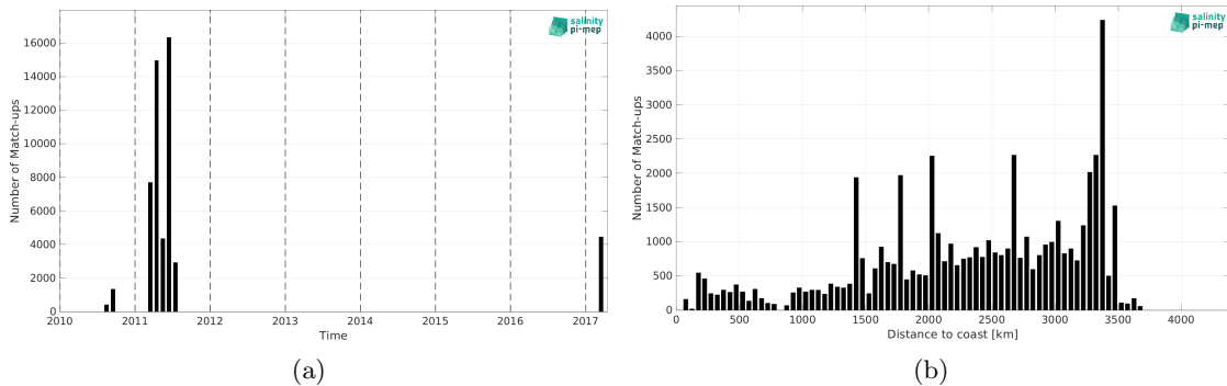
Figure 1: Number of match-ups between TSG (GOSUD-Sailing-ship) and CCI SSS L4 Merged-OI v4.4 - 7-day running (ESA) SSS as a function of time (a) and as function of the distance to coast (b) over the OTT zone Pi-MEP region and for the full satellite product period.
