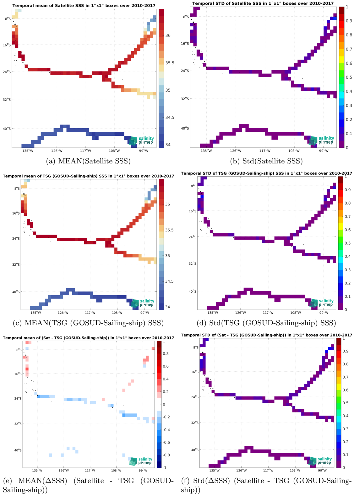
Figure 6: Temporal mean (left) and Std (right) of SSS from CCI SSS L4 Merged-OI v4.4 - 7-day running (ESA) (top), TSG (GOSUD-Sailing-ship) (middle), and of \Delta SSS (Satellite - TSG (GOSUD-Sailing-ship)). Only match-up pairs are used to generate these maps.
