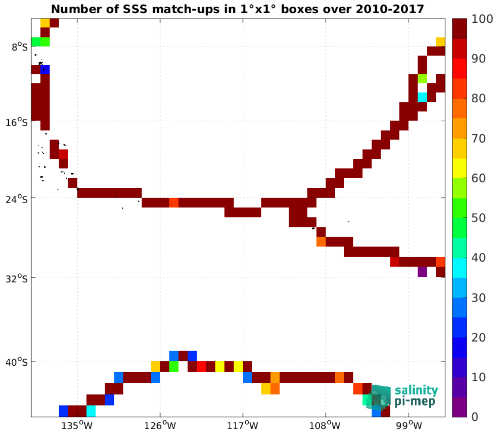
Figure 4: Number of SSS match-ups between TSG (GOSUD-Sailing-ship) SSS and the CCI SSS L4 Merged-OI v4.4 - 7-day running (ESA) SSS product for the OTT zone Pi-MEP region over 1^\circ \times 1^\circ boxes and for the full satellite product period.
