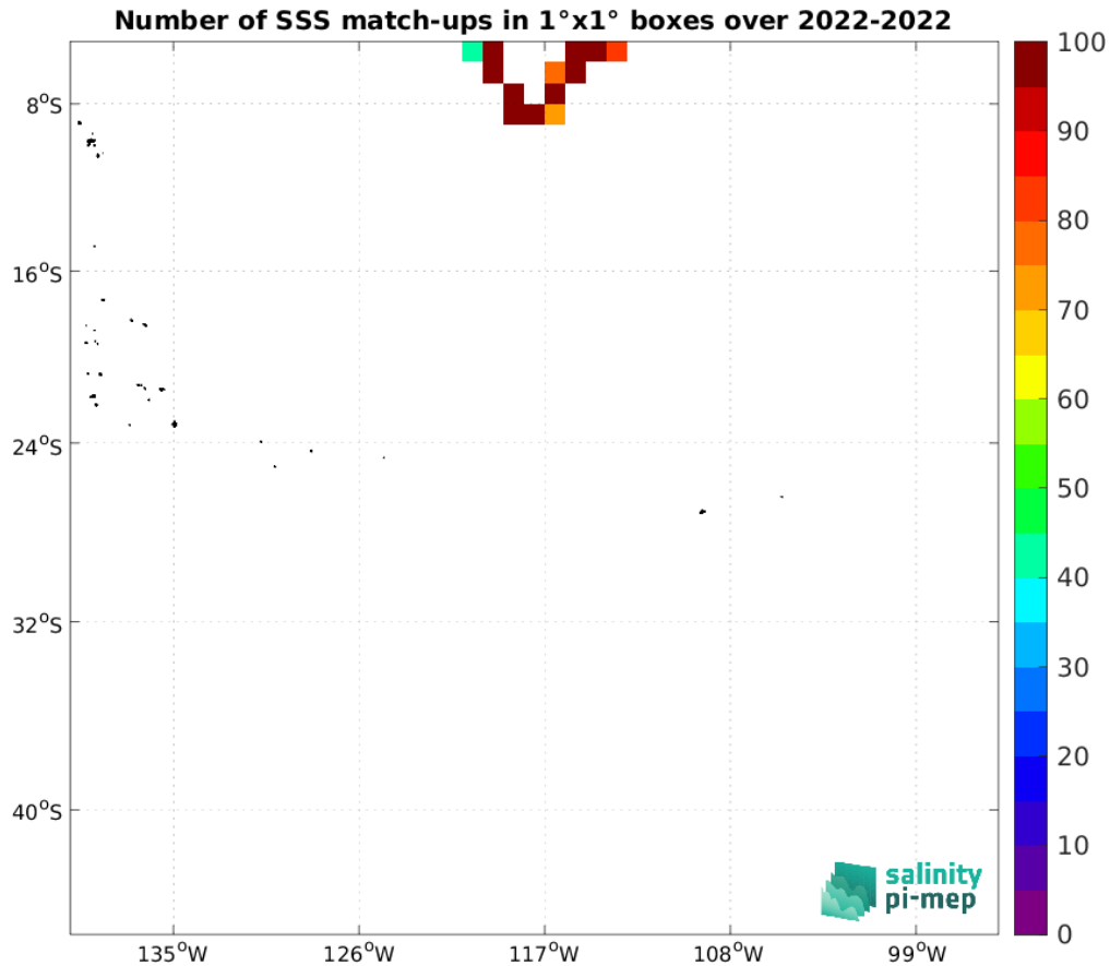
Figure 4: Number of SSS match-ups between Saildrone SSS and the CCI SSS L4 Merged-OI v4.4 - 7-day running (ESA) SSS product for the OTT zone Pi-MEP region over 1^\circ \times 1^\circ boxes and for the full satellite product period.
