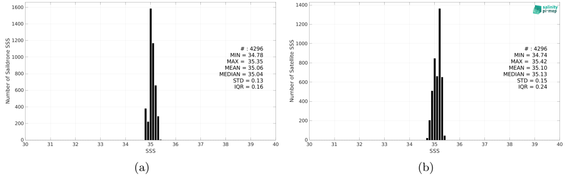
Figure 2: Histograms of SSS from Saildrone (a) and CCI SSS L4 Merged-OI v4.4 - 7-day running (ESA) (b) considering all match-up pairs per bins of 0.1 over the OTT zone Pi-MEP region and for the full satellite product period.
