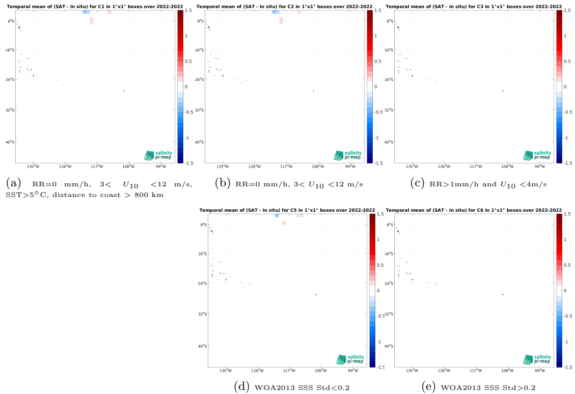
Figure 12: Temporal mean gridded over spatial boxes of size 1^\circ \times 1^\circ of \Delta SSS (CCI SSS L4 Merged-OI v4.4 - 7-day running (ESA) - Saildrone) for 5 different subdatasets corresponding to: RR=0 mm/h, 3 < U_{10} < 12 m/s, SST > 5^\circ C , distance to coast > 800 km (a), RR=0 mm/h, 3 < U_{10} < 12 m/s (b), RR > 1 mm/h and U_{10} < 4 m/s (c), WOA2013 SSS Std < 0.2 (d), WOA2013 SSS Std > 0.2 (e).
