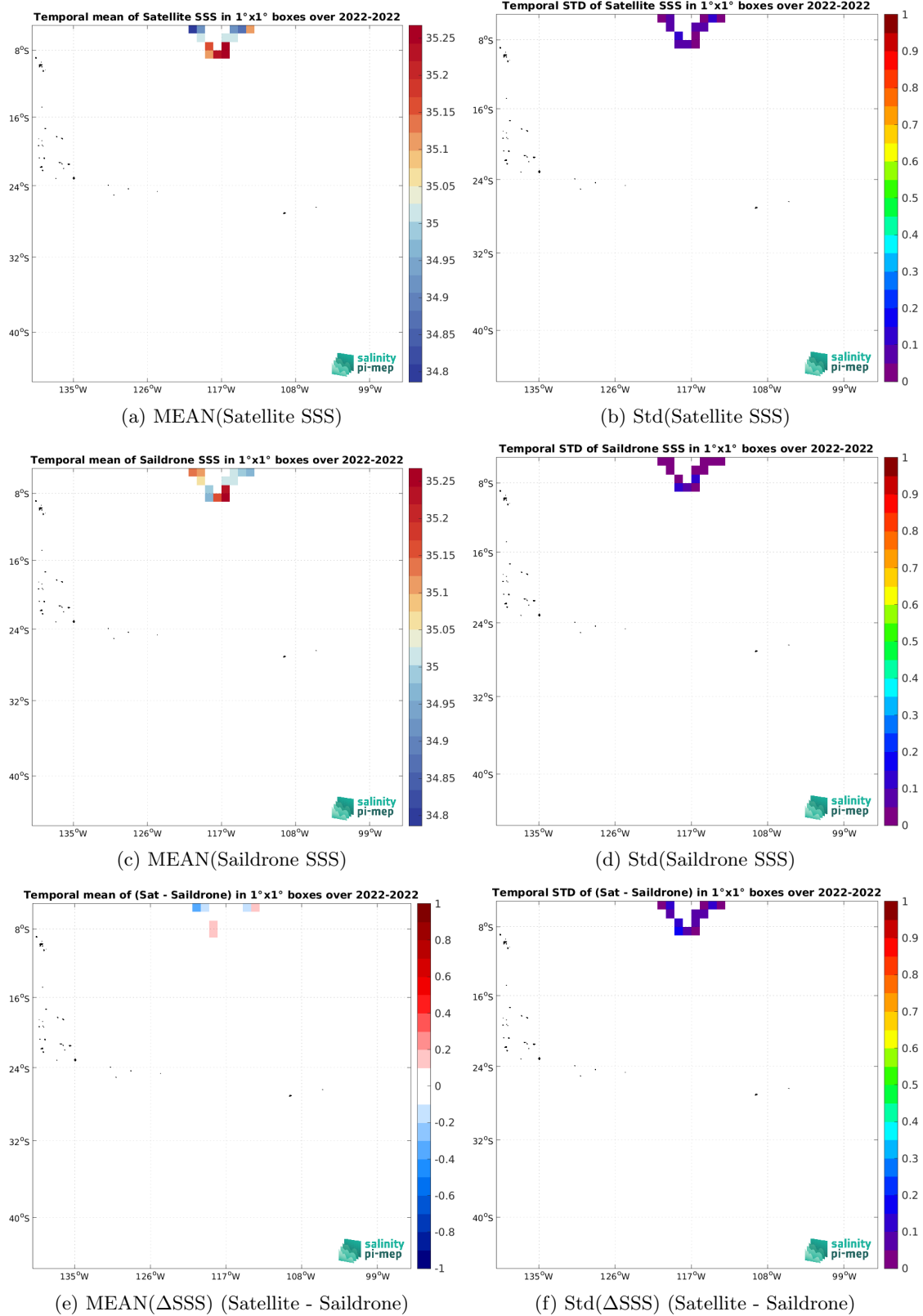
Figure 6: Temporal mean (left) and Std (right) of SSS from CCI SSS L4 Merged-OI v4.4 - 7-day running (ESA) (top), Saildrone (middle), and of \Delta SSS (Satellite - Saildrone). Only match-up pairs are used to generate these maps.
