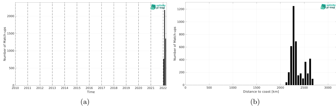
Figure 1: Number of match-ups between Saildrone and CCI SSS L4 Merged-OI v4.4 - 7-day running (ESA) SSS as a function of time (a) and as function of the distance to coast (b) over the OTT zone Pi-MEP region and for the full satellite product period.
