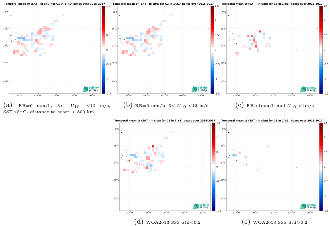
Figure 11: Temporal mean gridded over spatial boxes of size 1^\circ \times 1^\circ of \Delta SSS (CCI SSS L4 Merged-OI v4.4 - 7-day running (ESA) - Surface drifters) for 5 different subdatasets corresponding to: RR=0 mm/h, 3 < U_{10} < 12 m/s, SST > 5^\circ C, distance to coast > 800 km (a), RR=0 mm/h, 3 < U_{10} < 12 m/s (b), RR > 1 mm/h and U_{10} < 4 m/s (c), WOA2013 SSS Std < 0.2 (d), WOA2013 SSS Std > 0.2 (e).
