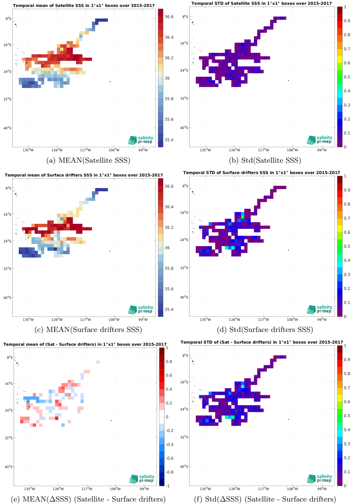
Figure 5: Temporal mean (left) and Std (right) of SSS from CCI SSS L4 Merged-OI v4.4 - 7-day running (ESA) (top), Surface drifters (middle), and of \Delta SSS (Satellite - Surface drifters). Only match-up pairs are used to generate these maps.
