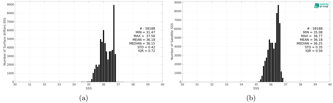
Figure 2: Histograms of SSS from Surface drifters (a) and CCI SSS L4 Merged-OI v4.4 - 7-day running (ESA) (b) considering all match-up pairs per bins of 0.1 over the OTT zone Pi-MEP region and for the full satellite product period.
