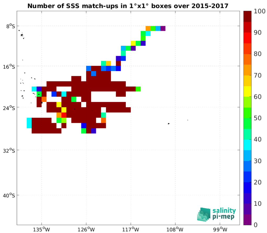
Figure 3: Number of SSS match-ups between Surface drifters SSS and the CCI SSS L4 Merged-OI v4.4 - 7-day running (ESA) SSS product for the OTT zone Pi-MEP region over 1°x1° boxes and for the full satellite product period.
