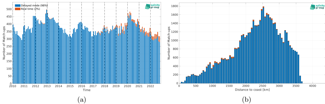
Figure 1: Number of match-ups between Argo and CCI SSS L4 Merged-OI v4.4 - 7-day running (ESA) SSS as a function of time (a) and as function of the distance to coast (b) over the OTT zone Pi-MEP region and for the full satellite product period.
