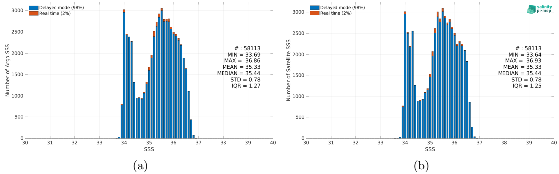
Figure 2: Histograms of SSS from Argo (a) and CCI SSS L4 Merged-OI v4.4 - 7-day running (ESA) (b) considering all match-up pairs per bins of 0.1 over the OTT zone Pi-MEP region and for the full satellite product period.
