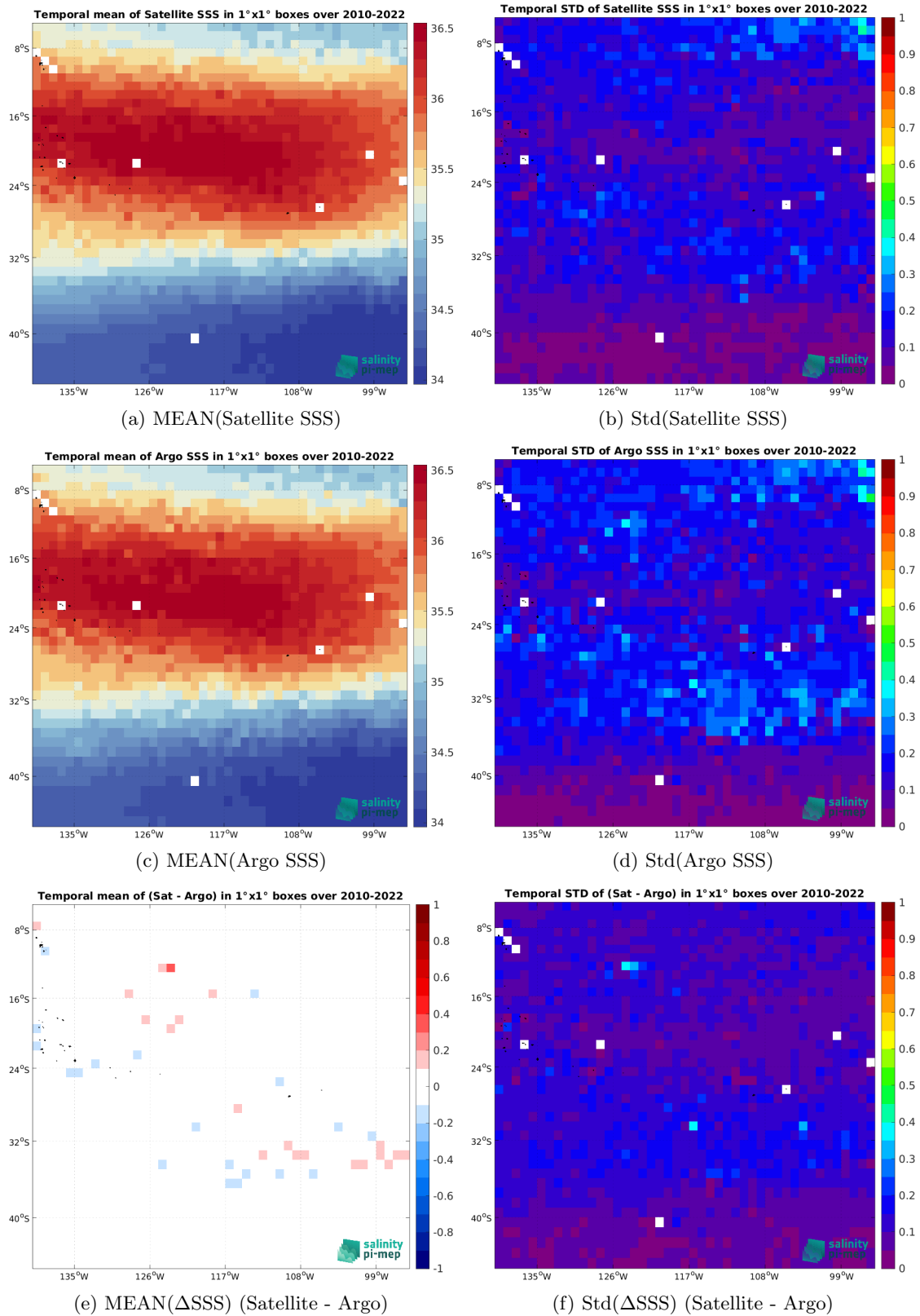
Figure 6: Temporal mean (left) and Std (right) of SSS from CCI SSS L4 Merged-OI v4.4 - 7-day running (ESA) (top), Argo (middle), and of \Delta SSS (Satellite - Argo). Only match-up pairs are used to generate these maps.
