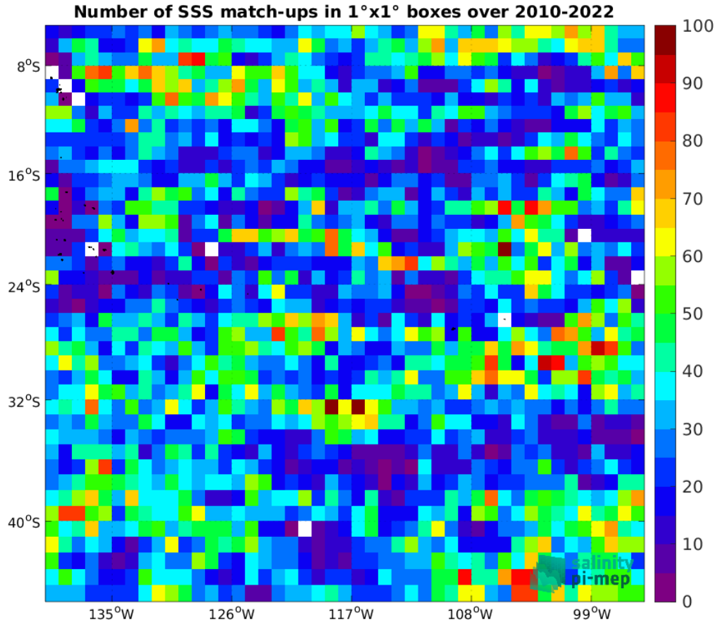
Figure 4: Number of SSS match-ups between Argo SSS and the CCI SSS L4 Merged-OI v4.4 - 7-day running (ESA) SSS product for the OTT zone Pi-MEP region over 1^\circ \times 1^\circ boxes and for the full satellite product period.
