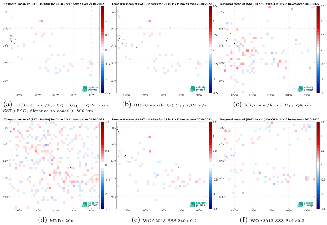
Figure 12: Temporal mean gridded over spatial boxes of size 1^\circ \times 1^\circ of \Delta SSS (CCI SSS L4 Merged-OI v4.4 - 7-day running (ESA) - Argo) for 6 different subdatasets corresponding to:RR=0 mm/h, 3 < U_{10} < 12 m/s, SST >5^\circ C, distance to coast > 800 km (a), RR=0 mm/h, 3 < U_{10} < 12 m/s (b), RR >1 mm/h and U_{10} < 4 m/s (c),MLD <20 m (d),WOA2013 SSS Std <0.2 (e),WOA2013 SSS Std >0.2 (f).
