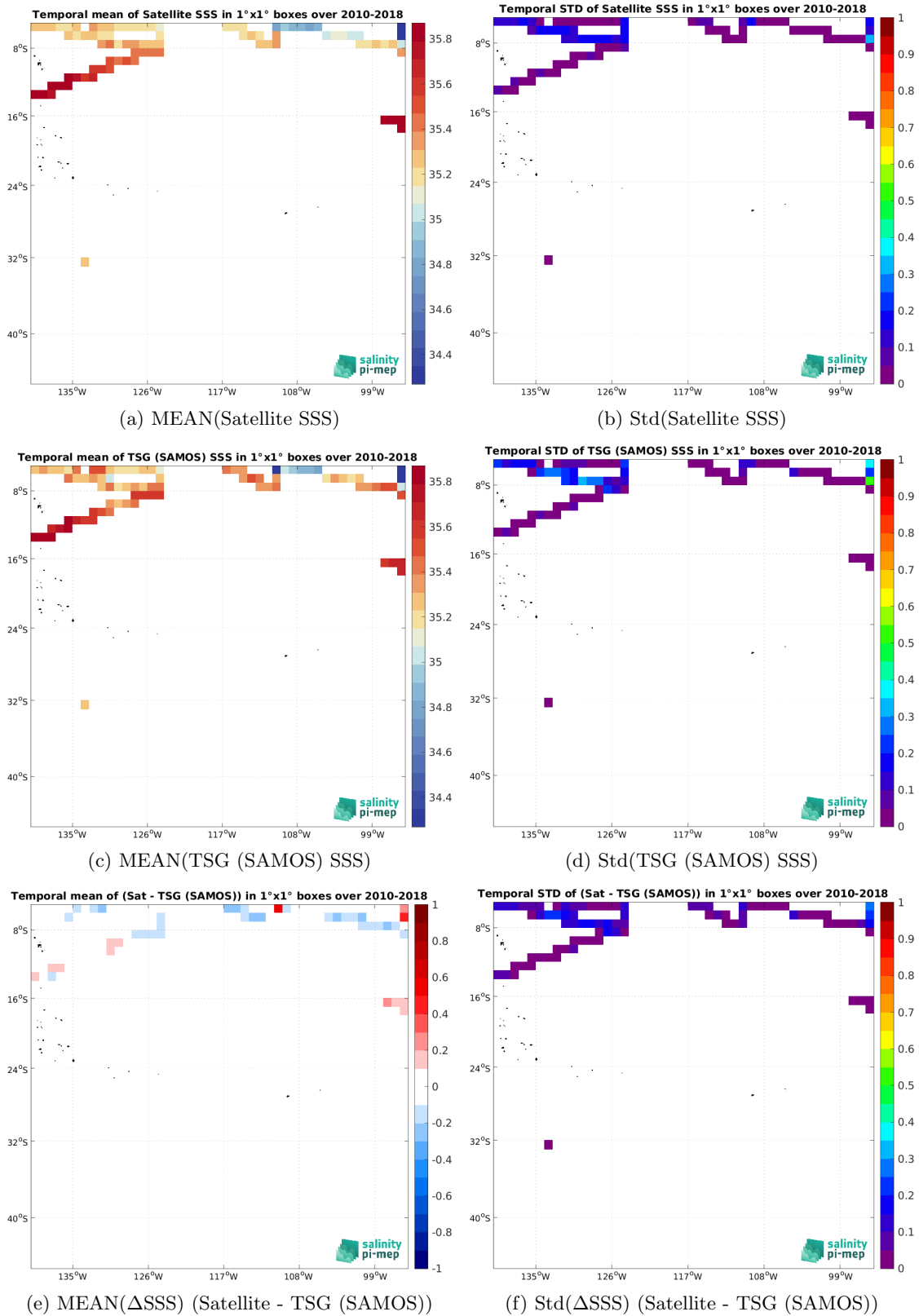
Figure 6: Temporal mean (left) and Std (right) of SSS from CCI SSS L4 Merged-OI v4.4 - 30-day running (ESA) (top), TSG (SAMOS) (middle), and of \Delta SSS (Satellite - TSG (SAMOS)). Only match-up pairs are used to generate these maps.
