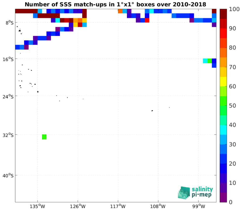
Figure 4: Number of SSS match-ups between TSG (SAMOS) SSS and the CCI SSS L4 Merged-OI v4.4 - 30-day running (ESA) SSS product for the OTT zone Pi-MEP region over 1^\circ \times 1^\circ boxes and for the full satellite product period.
