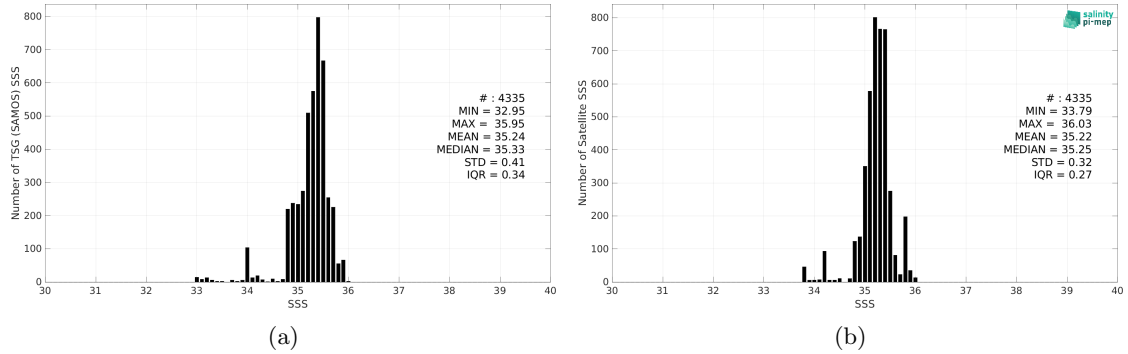
Figure 2: Histograms of SSS from TSG (SAMOS) (a) and CCI SSS L4 Merged-OI v4.4 - 30-day running (ESA) (b) considering all match-up pairs per bins of 0.1 over the OTT zone Pi-MEP region and for the full satellite product period.
