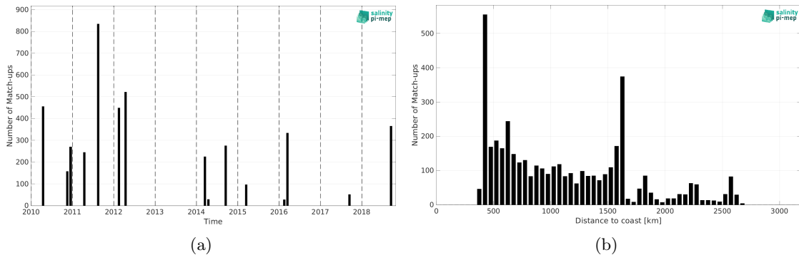
Figure 1: Number of match-ups between TSG (SAMOS) and CCI SSS L4 Merged-OI v4.4 - 30-day running (ESA) SSS as a function of time (a) and as function of the distance to coast (b) over the OTT zone Pi-MEP region and for the full satellite product period.
