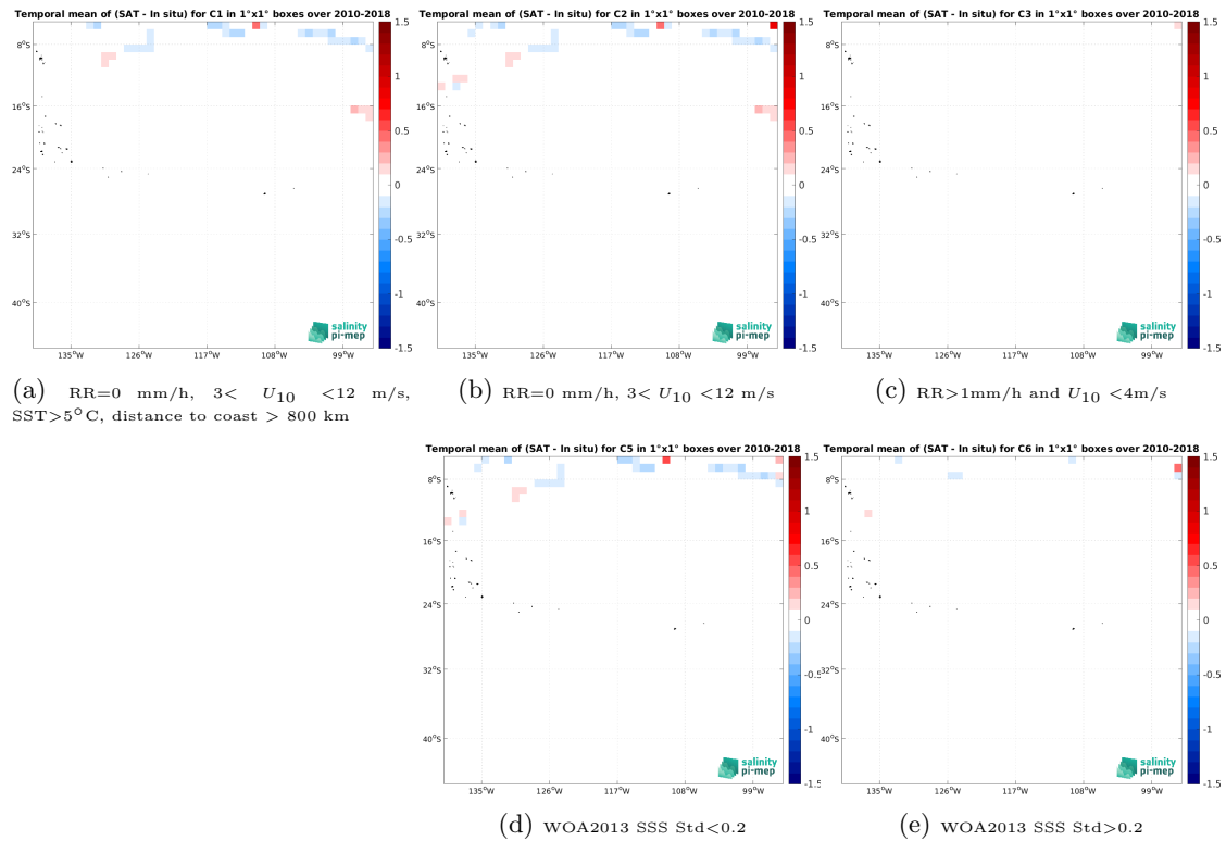
Figure 12: Temporal mean gridded over spatial boxes of size 1^\circ \times 1^\circ of \Delta SSS (CCI SSS L4 Merged-OI v4.4 - 30-day running (ESA) - TSG (SAMOS)) for 5 different subdatasets corresponding to:RR=0 mm/h, 3 < U_{10} < 12 m/s, SST >5^\circ C, distance to coast > 800 km (a), RR=0 mm/h, 3 < U_{10} < 12 m/s (b), RR >1 mm/h and U_{10} < 4 m/s (c), WOA2013 SSS Std <0.2 (d), WOA2013 SSS Std >0.2 (e).
