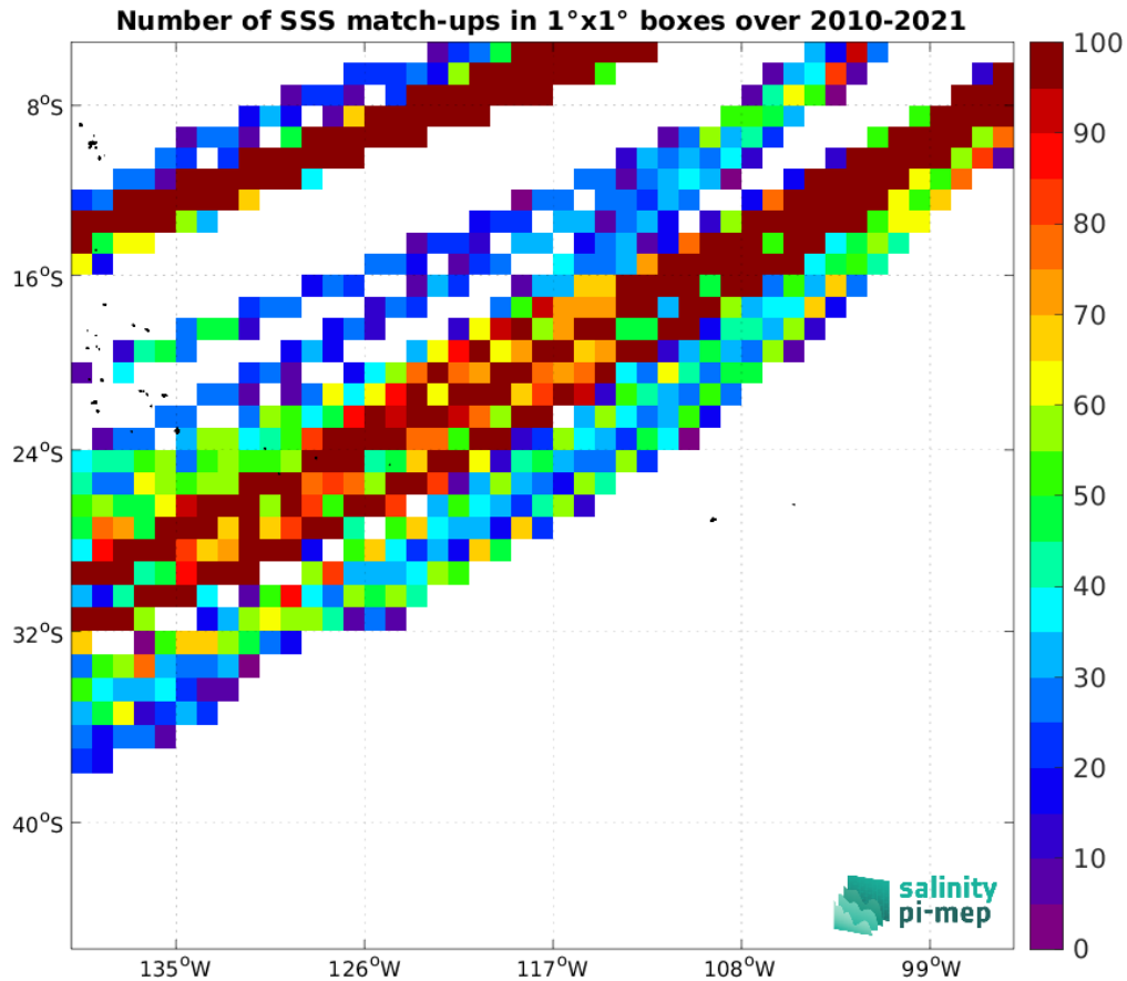
Figure 4: Number of SSS match-ups between TSG (LEGOS-DM) SSS and the CCI SSS L4 Merged-OI v4.4 - 30-day running (ESA) SSS product for the OTT zone Pi-MEP region over 1^\circ \times 1^\circ boxes and for the full satellite product period.
