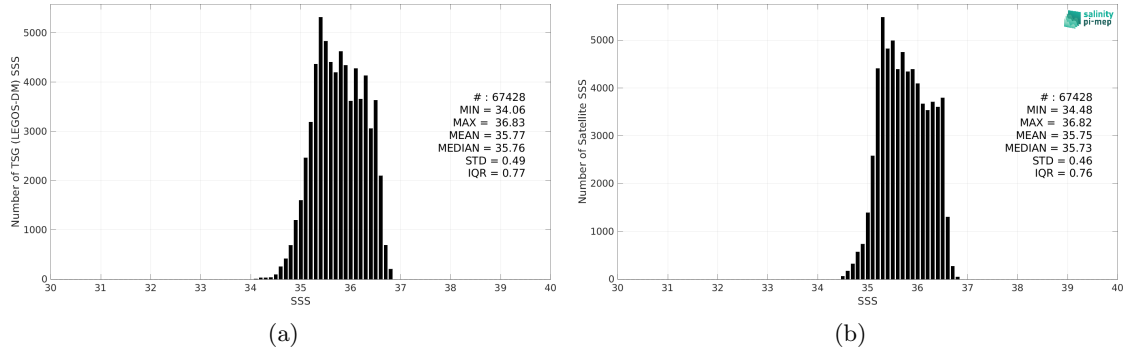
Figure 2: Histograms of SSS from TSG (LEGOS-DM) (a) and CCI SSS L4 Merged-OI v4.4 - 30-day running (ESA) (b) considering all match-up pairs per bins of 0.1 over the OTT zone Pi-MEP region and for the full satellite product period.
