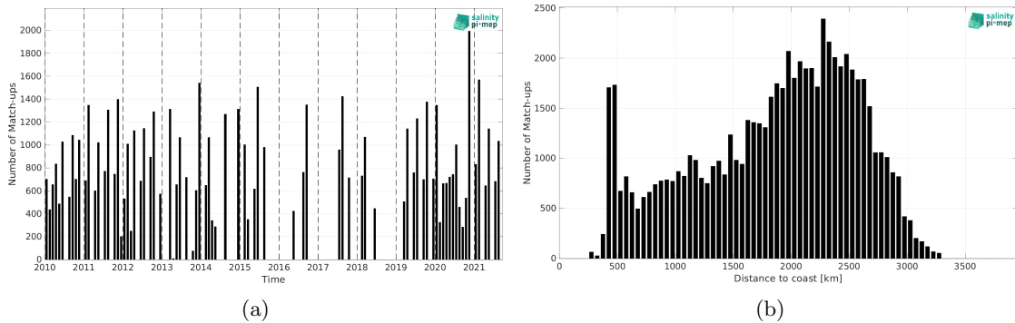
Figure 1: Number of match-ups between TSG (LEGOS-DM) and CCI SSS L4 Merged-OI v4.4 - 30-day running (ESA) SSS as a function of time (a) and as function of the distance to coast (b) over the OTT zone Pi-MEP region and for the full satellite product period.
