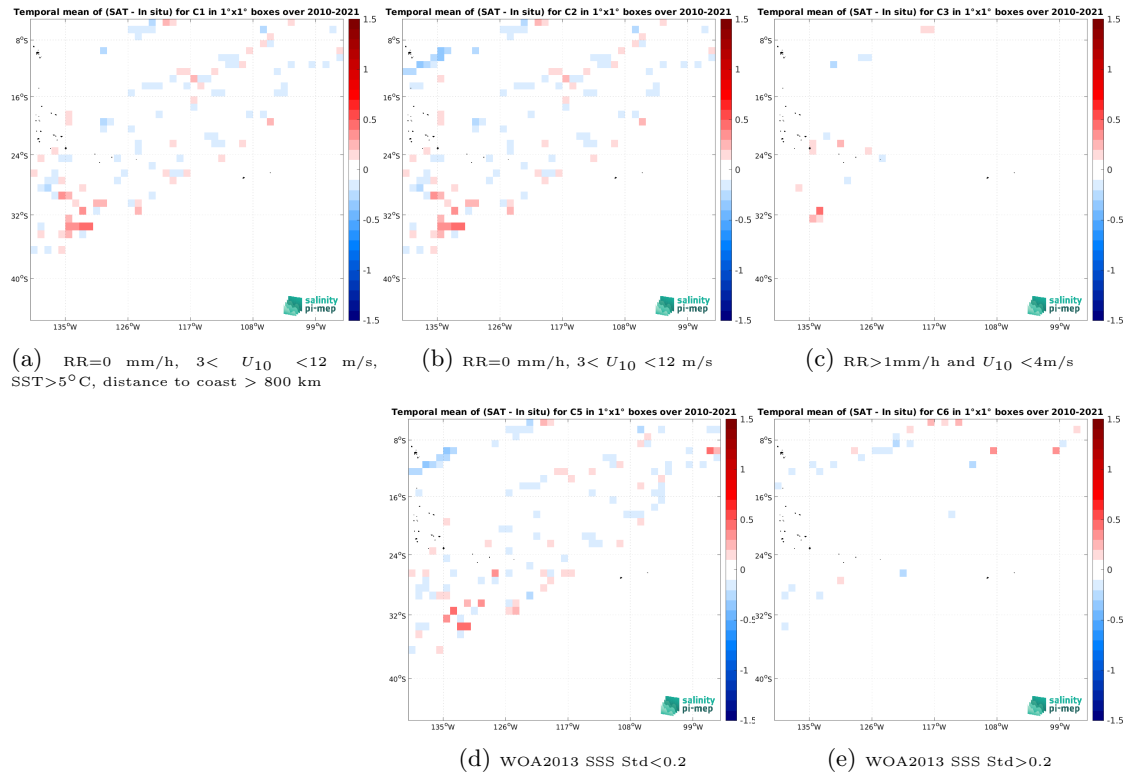
Figure 12: Temporal mean gridded over spatial boxes of size 1^{\circ}\times 1^{\circ} of \Delta\text{SSS} (CCI SSS L4 Merged-OI v4.4 - 30-day running (ESA) - TSG (LEGOS-DM)) for 5 different subdatasets corresponding to:RR=0 mm/h, 3 < U_{10} < 12 m/s, SST >5^{\circ}\text{C} , distance to coast > 800 km (a), RR=0 mm/h, 3 < U_{10} < 12 m/s (b), RR >1 mm/h and U_{10} < 4 m/s (c), WOA2013 SSS Std <0.2 (d), WOA2013 SSS Std >0.2 (e).
