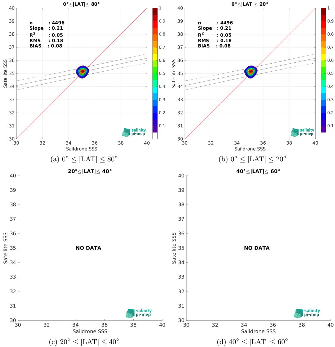
Figure 9: Contour maps of the concentration of CCI SSS L4 Merged-OI v4.4 - 30-day running (ESA) SSS (y-axis) versus Ssaldrone SSS (x-axis) at match-up pairs for different latitude bands. For each plot, the red line shows x=y . The black thin and dashed lines indicate a linear fit through the data cloud and the \pm 95\% confidence levels, respectively. The number match-up pairs n , the slope and R^2 coefficient of the linear fit, the root mean square (RMS) and the mean bias between satellite and in situ data are indicated for each latitude band in each plots.
