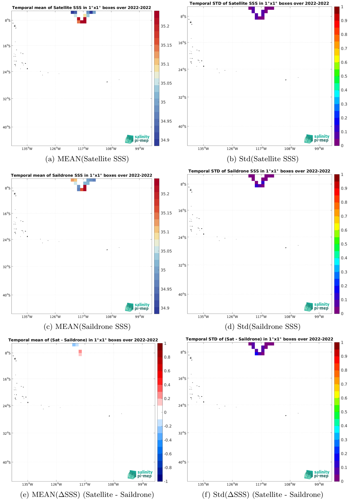
Figure 6: Temporal mean (left) and Std (right) of SSS from CCI SSS L4 Merged-OI v4.4 - 30-day running (ESA) (top), Saildrone (middle), and of \Delta SSS (Satellite - Saildrone). Only match-up pairs are used to generate these maps.
