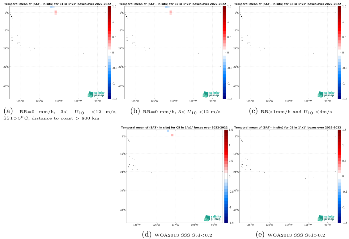
Figure 12: Temporal mean gridded over spatial boxes of size 1^\circ \times 1^\circ of \Delta SSS (CCI SSS L4 Merged-OI v4.4 - 30-day running (ESA) - Saildrone) for 5 different subdatasets corresponding to: RR=0 mm/h, 3 < U_{10} < 12 m/s, SST > 5^\circ C , distance to coast > 800 km (a), RR=0 mm/h, 3 < U_{10} < 12 m/s (b), RR > 1 mm/h and U_{10} < 4 m/s (c), WOA2013 SSS Std < 0.2 (d), WOA2013 SSS Std > 0.2 (e).
