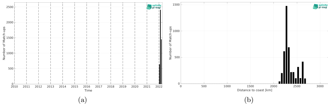
Figure 1: Number of match-ups between Saildrone and CCI SSS L4 Merged-OI v4.4 - 30-day running (ESA) SSS as a function of time (a) and as function of the distance to coast (b) over the OTT zone Pi-MEP region and for the full satellite product period.
