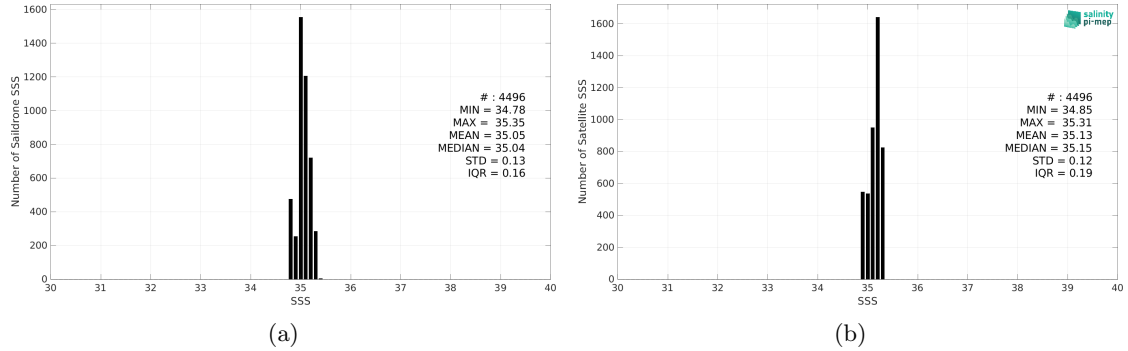
Figure 2: Histograms of SSS from Saildrone (a) and CCI SSS L4 Merged-OI v4.4 - 30-day running (ESA) (b) considering all match-up pairs per bins of 0.1 over the OTT zone Pi-MEP region and for the full satellite product period.
