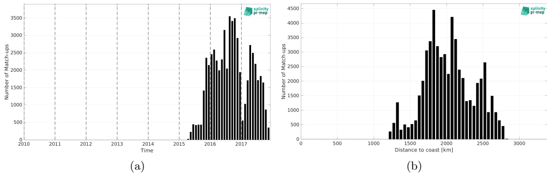
Figure 1: Number of match-ups between Surface drifters and CCI SSS L4 Merged-OI v4.4 - 30-day running (ESA) SSS as a function of time (a) and as function of the distance to coast (b) over the OTT zone Pi-MEP region and for the full satellite product period.
