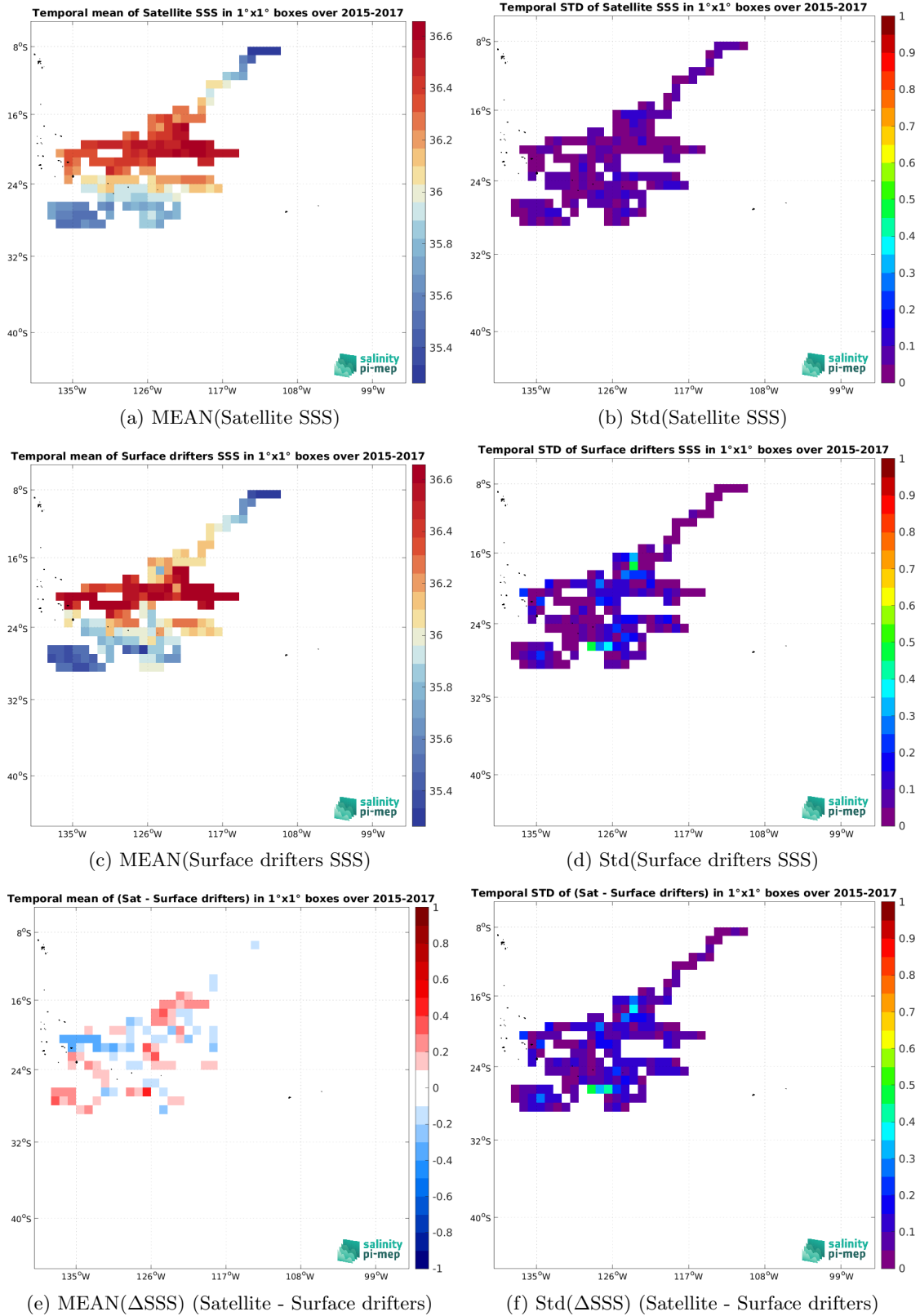
Figure 5: Temporal mean (left) and Std (right) of SSS from CCI SSS L4 Merged-OI v4.4 - 30-day running (ESA) (top), Surface drifters (middle), and of \Delta SSS (Satellite - Surface drifters). Only match-up pairs are used to generate these maps.
