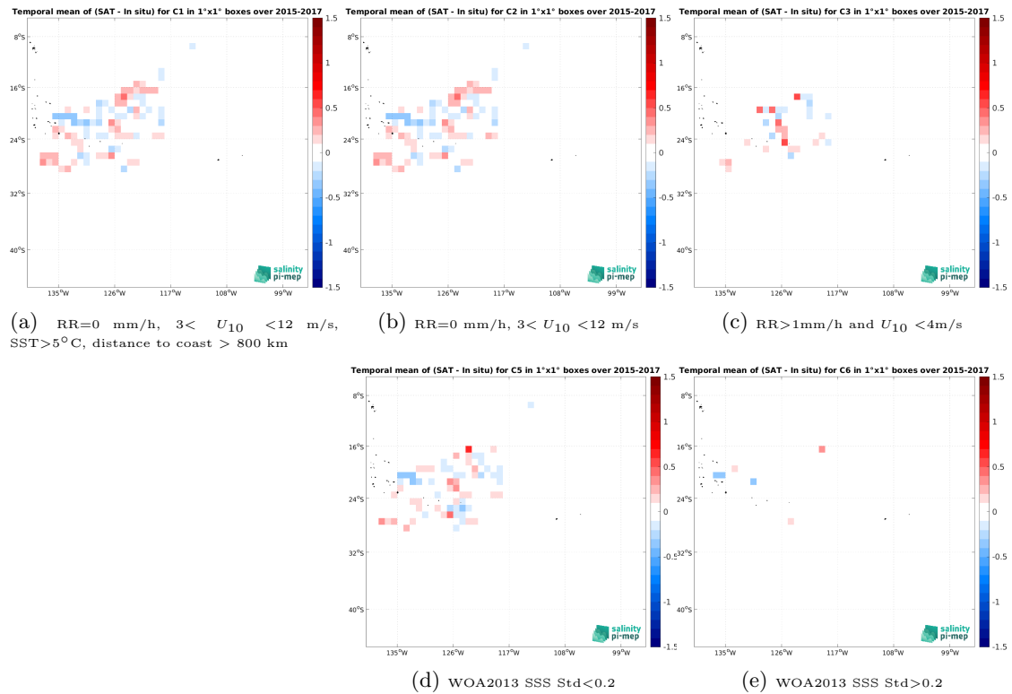
Figure 11: Temporal mean gridded over spatial boxes of size 1^\circ \times 1^\circ of \Delta SSS (CCI SSS L4 Merged-OI v4.4 - 30-day running (ESA) - Surface drifters) for 5 different subdatasets corresponding to: RR=0 mm/h, 3 < U_{10} < 12 m/s, SST > 5^\circ\text{C} , distance to coast > 800 km (a), RR=0 mm/h, 3 < U_{10} < 12 m/s (b), RR > 1 mm/h and U_{10} < 4 m/s (c), WOA2013 SSS Std < 0.2 (d), WOA2013 SSS Std > 0.2 (e).
