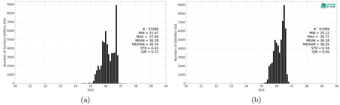
Figure 2: Histograms of SSS from Surface drifters (a) and CCI SSS L4 Merged-OI v4.4 - 30-day running (ESA) (b) considering all match-up pairs per bins of 0.1 over the OTT zone Pi-MEP region and for the full satellite product period.
