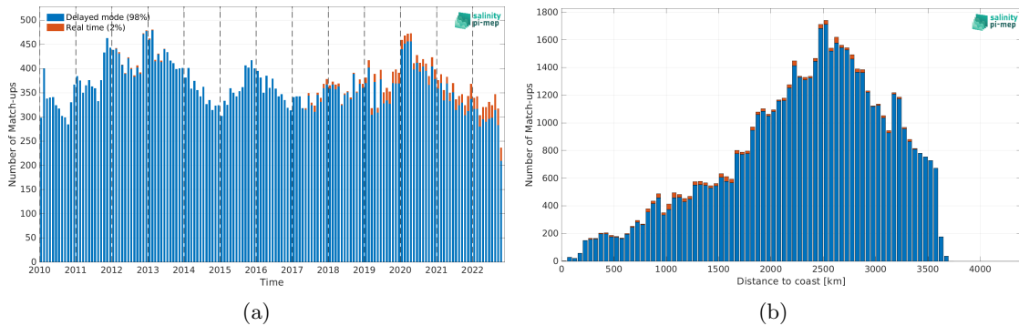
Figure 1: Number of match-ups between Argo and CCI SSS L4 Merged-OI v4.4 - 30-day running (ESA) SSS as a function of time (a) and as function of the distance to coast (b) over the OTT zone Pi-MEP region and for the full satellite product period.
