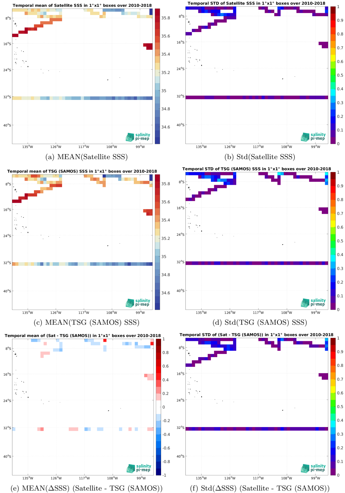
Figure 6: Temporal mean (left) and Std (right) of SSS from CCI SSS L4 Merged-OI v3.2 - 7-day running (ESA) (top), TSG (SAMOS) (middle), and of \Delta SSS (Satellite - TSG (SAMOS)). Only match-up pairs are used to generate these maps.
