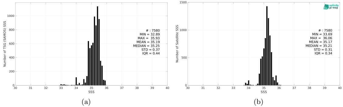
Figure 2: Histograms of SSS from TSG (SAMOS) (a) and CCI SSS L4 Merged-OI v3.2 - 7-day running (ESA) (b) considering all match-up pairs per bins of 0.1 over the OTT zone Pi-MEP region and for the full satellite product period.
