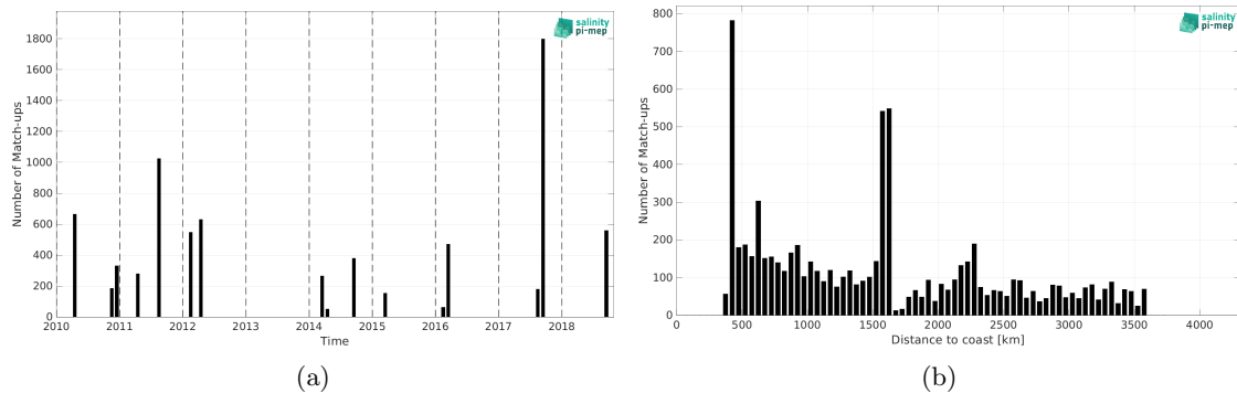
Figure 1: Number of match-ups between TSG (SAMOS) and CCI SSS L4 Merged-OI v3.2 - 7-day running (ESA) SSS as a function of time (a) and as function of the distance to coast (b) over the OTT zone Pi-MEP region and for the full satellite product period.
