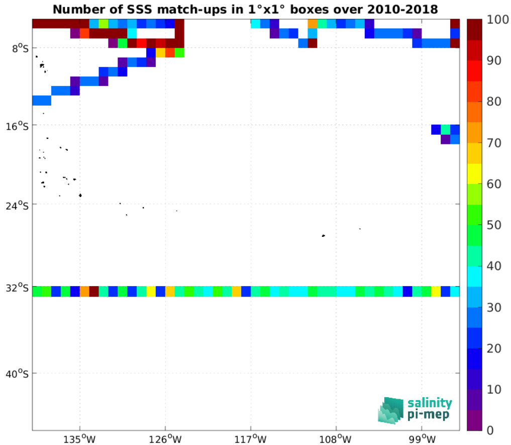
Figure 4: Number of SSS match-ups between TSG (SAMOS) SSS and the CCI SSS L4 Merged-OI v3.2 - 7-day running (ESA) SSS product for the OTT zone Pi-MEP region over 1^\circ \times 1^\circ boxes and for the full satellite product period.
