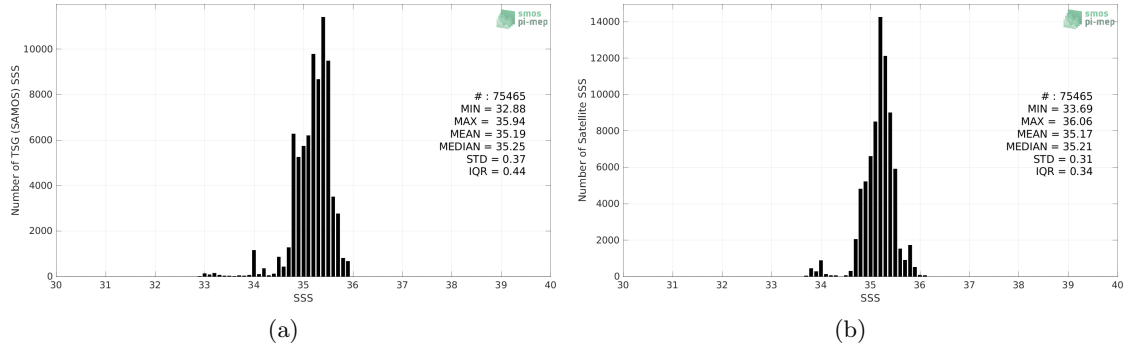
Figure 2: Histograms of SSS from TSG (SAMOS) (a) and CCI SSS L4 Merged-OI v3.2 - 7-day running (ESA) (b) considering all match-up pairs per bins of 0.1 over the OTT zone Pi-MEP region and for the full satellite product period.
