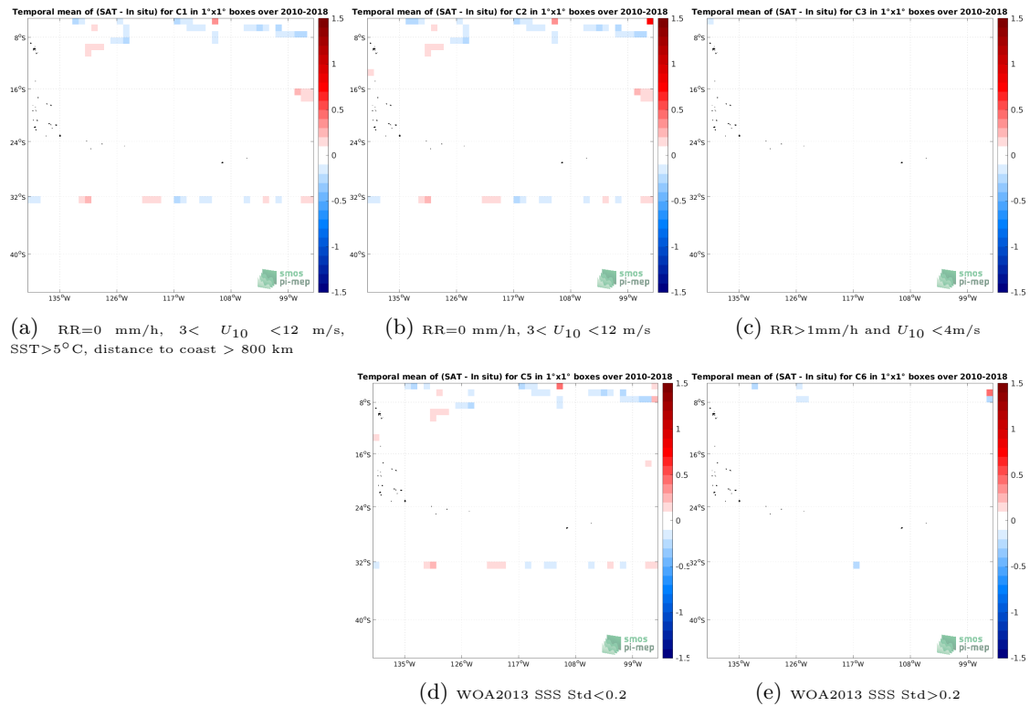
Figure 12: Temporal mean gridded over spatial boxes of size 1^\circ \times 1^\circ of \Delta SSS (CCI SSS L4 Merged-OI v3.2 - 7-day running (ESA) - TSG (SAMOS)) for 5 different subdatasets corresponding to: RR=0 mm/h, 3 < U_{10} < 12 m/s, SST > 5^\circ C , distance to coast > 800 km (a), RR=0 mm/h, 3 < U_{10} < 12 m/s (b), RR > 1 mm/h and U_{10} < 4 m/s (c), WOA2013 SSS Std < 0.2 (d), WOA2013 SSS Std > 0.2 (e).
