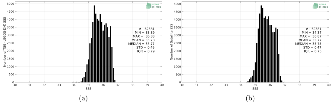
Figure 2: Histograms of SSS from TSG (LEGOS-DM) (a) and CCI SSS L4 Merged-OI v3.2 - 7-day running (ESA) (b) considering all match-up pairs per bins of 0.1 over the OTT zone Pi-MEP region and for the full satellite product period.
