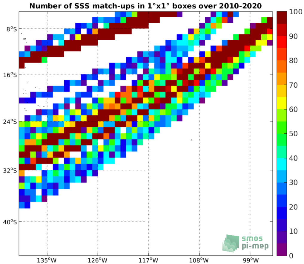
Figure 4: Number of SSS match-ups between TSG (LEGOS-DM) SSS and the CCI SSS L4 Merged-OI v3.2 - 7-day running (ESA) SSS product for the OTT zone Pi-MEP region over 1^\circ \times 1^\circ boxes and for the full satellite product period.
