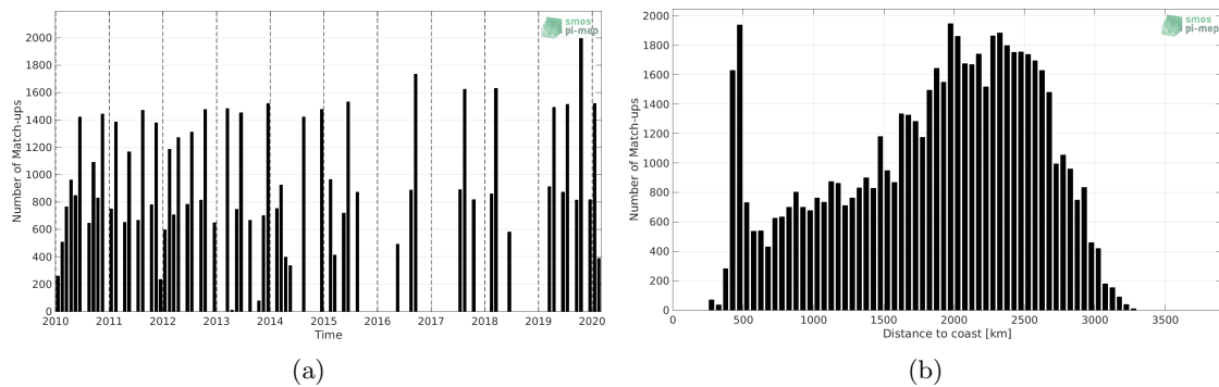
Figure 1: Number of match-ups between TSG (LEGOS-DM) and CCI SSS L4 Merged-OI v3.2 - 7-day running (ESA) SSS as a function of time (a) and as function of the distance to coast (b) over the OTT zone Pi-MEP region and for the full satellite product period.
