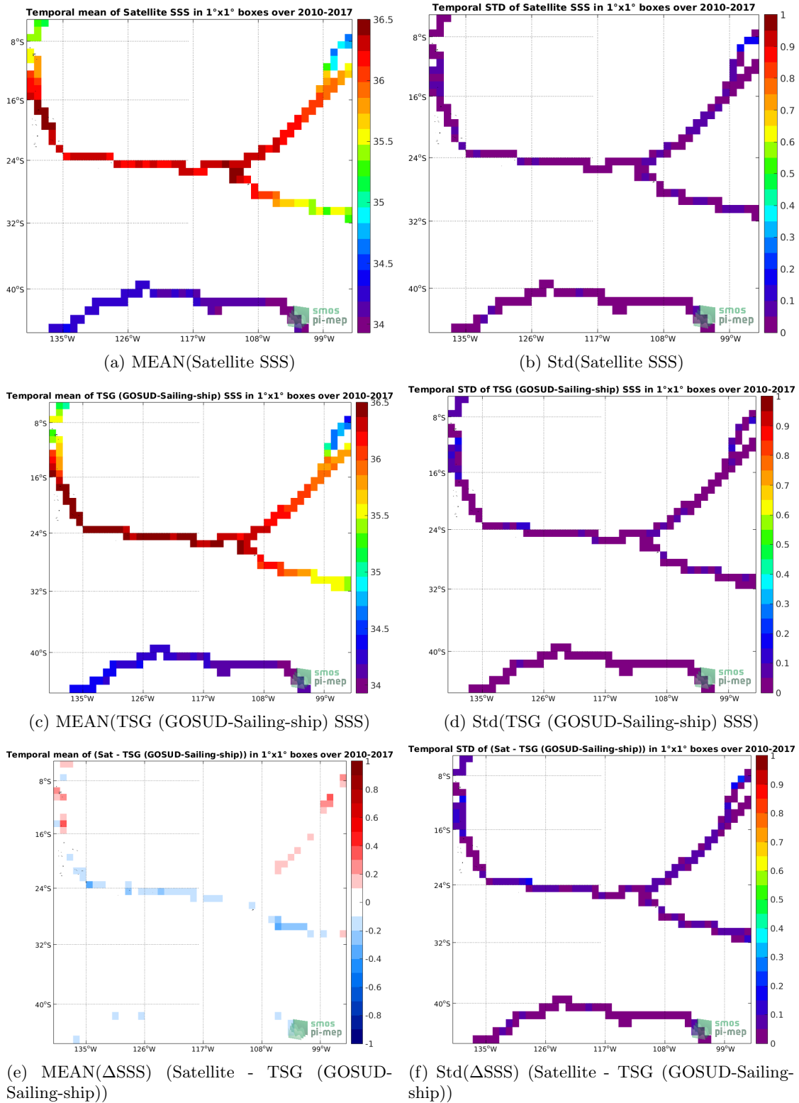
Figure 6: Temporal mean (left) and Std (right) of SSS from CCI SSS L4 Merged-OI v3.2 - 7-day running (ESA) (top), TSG (GOSUD-Sailing-ship) (middle), and of \Delta SSS (Satellite - TSG (GOSUD-Sailing-ship)). Only match-up pairs are used to generate these maps.
